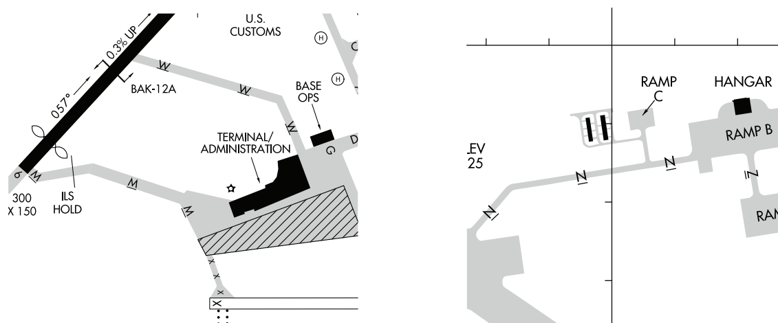
Figure 3.9 Taxiway Identification - Use of M, N, W and Z
