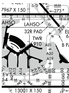
Figure 3.10 Taxiway Identification - Use of M, MM and M with a Number
