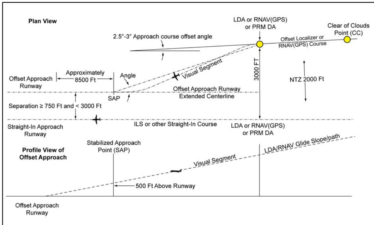
FIG 5-4-22 SOIA Approach Geometry
