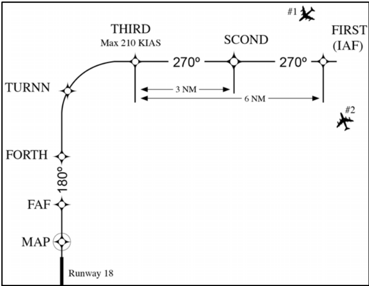
FIG 5-4-13 Example of an RNAV Approach with RF Leg
