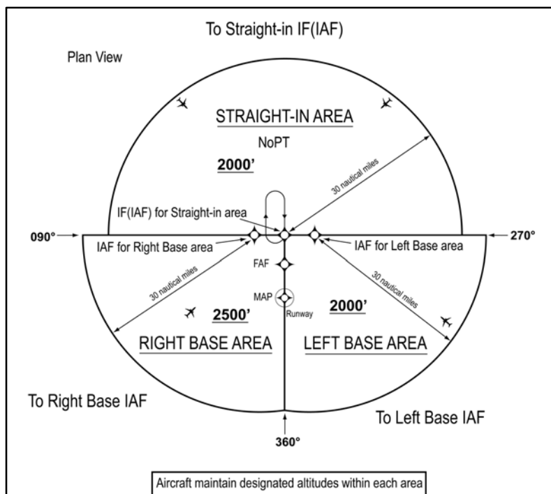
FIG ENR 1.5–21 TAA Area
