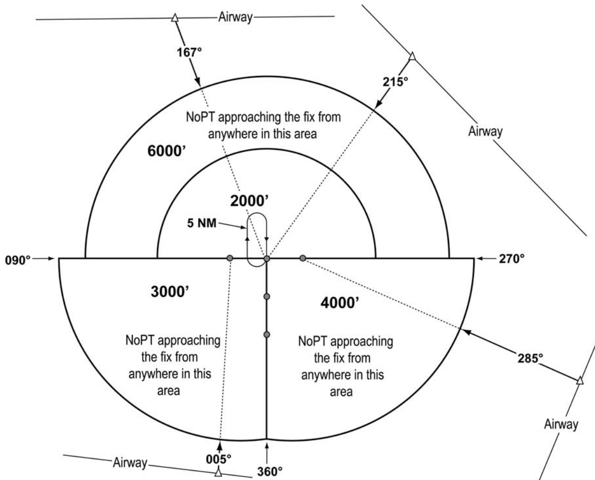
FIG ENR 1.5–27 Examples of a TAA with Feeders from an Airway
