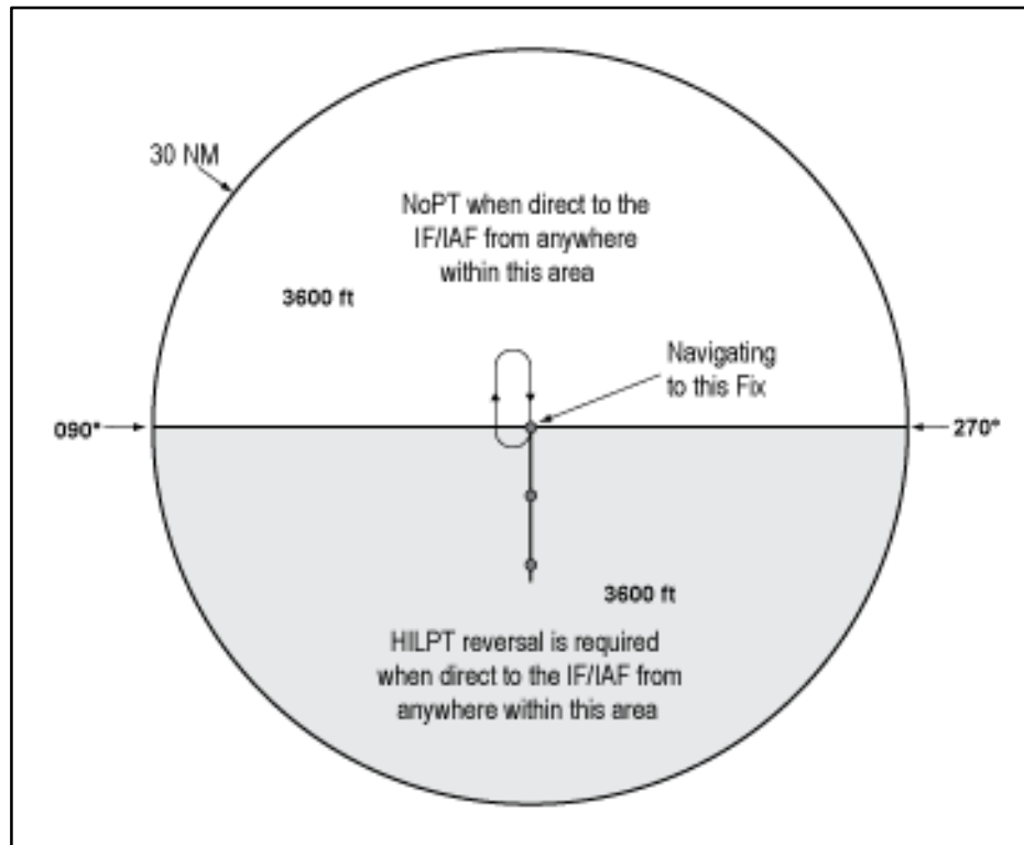
FIG ENR 1.5–24 TAA with Left and Right Base Areas Eliminated
