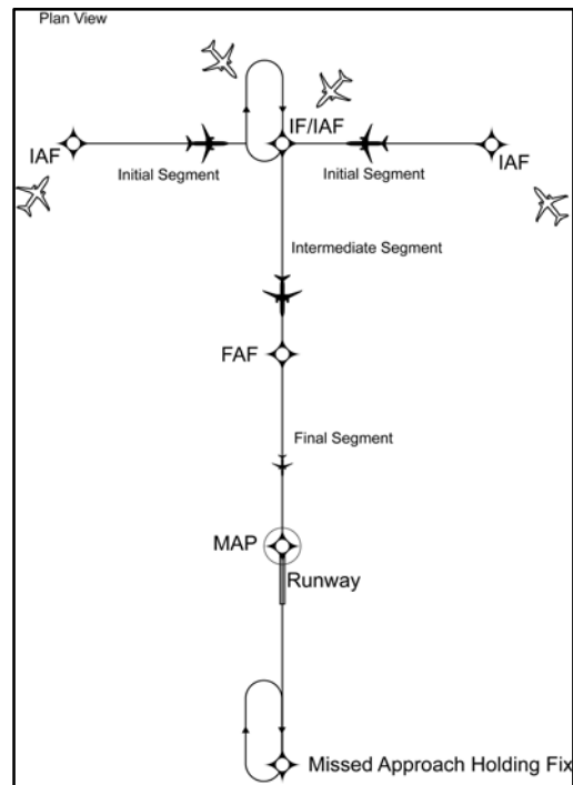
FIG ENR 1.5-19 Basic “T” Design
