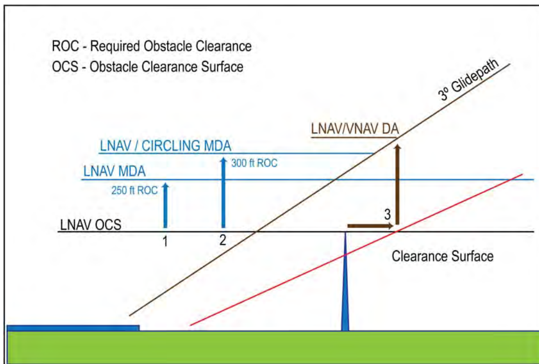
FIG ENR 1.5–30 Explanation of LNAV and/or Circling Minima Lower than LNAV/VNAV DA
