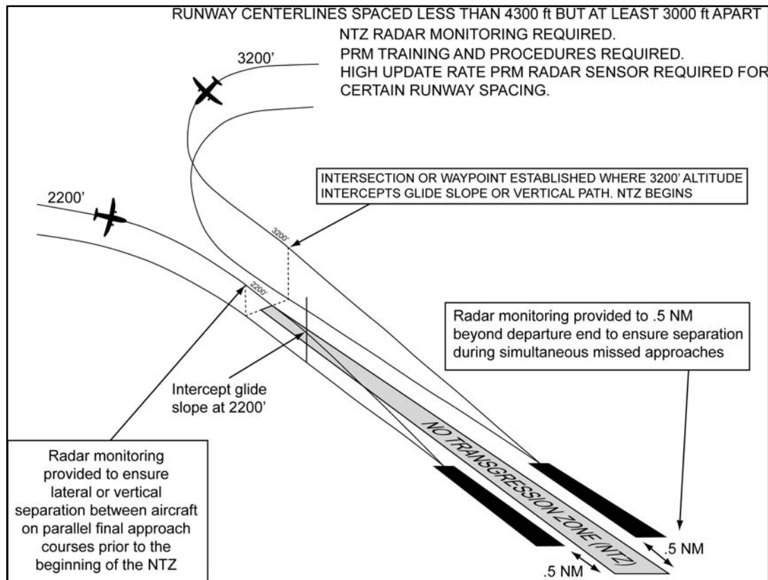
FIG ENR 1.5–35 PRM Approaches Simultaneous Close Parallel
