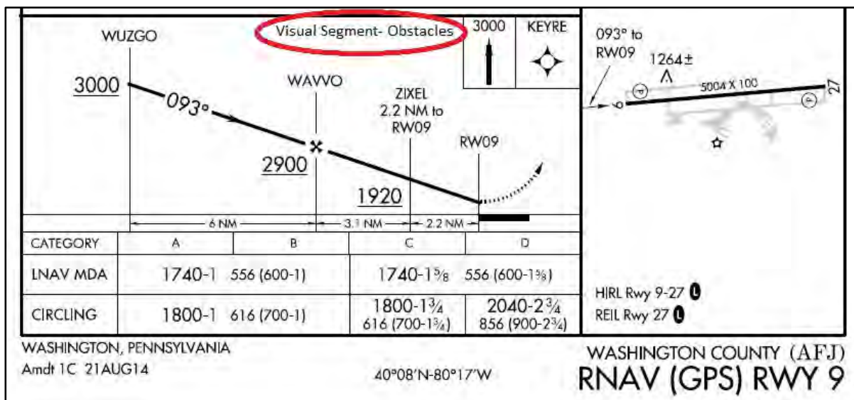
FIG ENR 1.5–31 Example of a Chart Note
