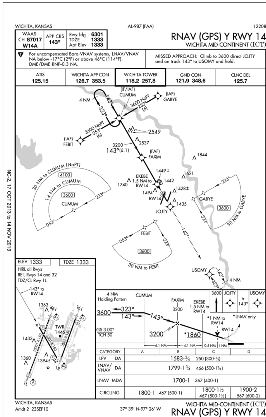
FIG ENR 1.5-23 RNAV (GPS) Approach Chart
