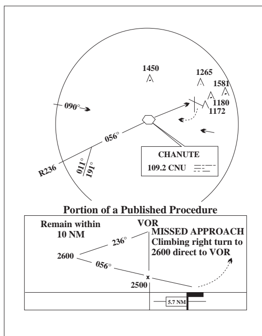
FIG ENR 1.5-39 Missed Approach
