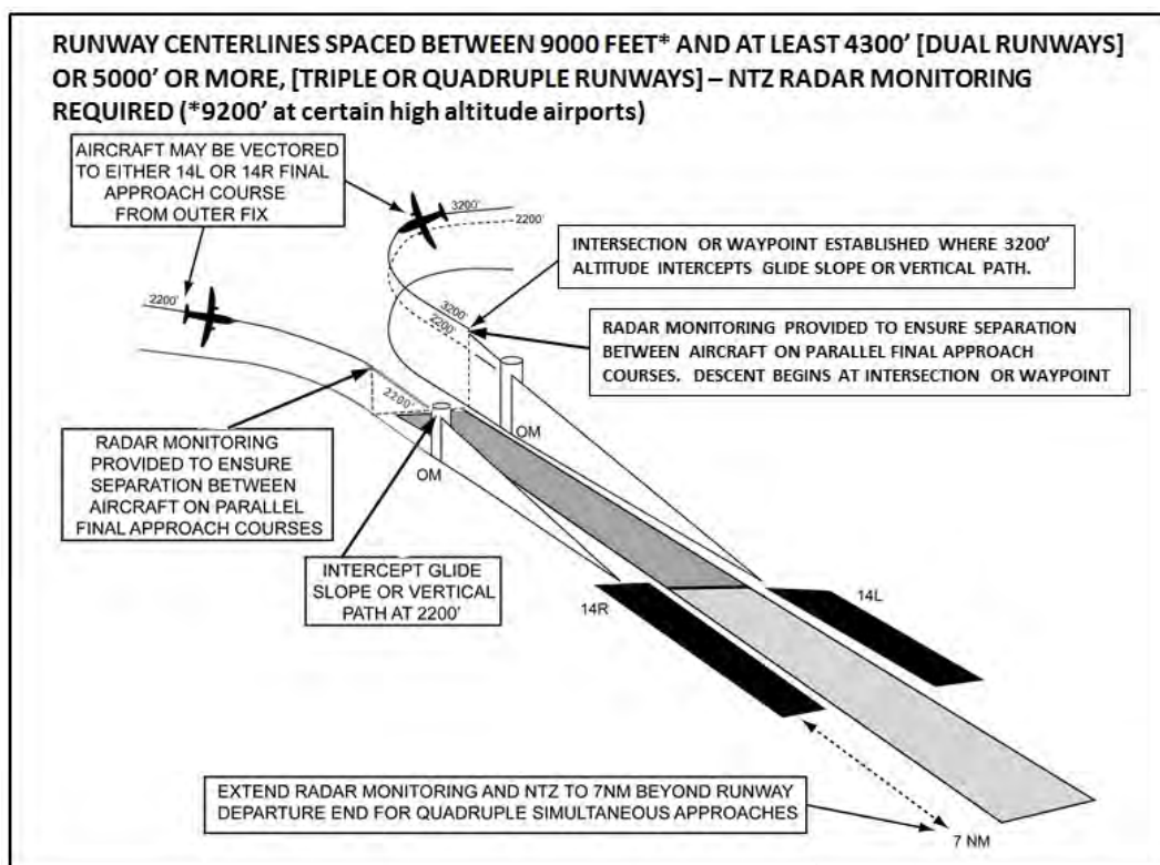
FIG ENR 1.5–34 Simultaneous (Parallel) Independent ILS/RNAV/GLS Approaches
