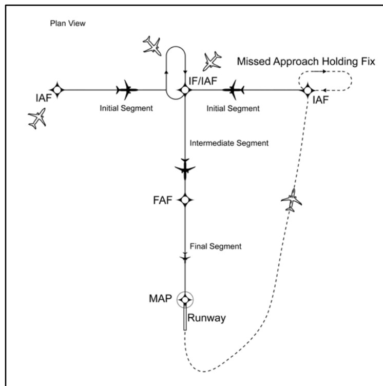
FIG ENR 1.5-20 Basic “T” Design
