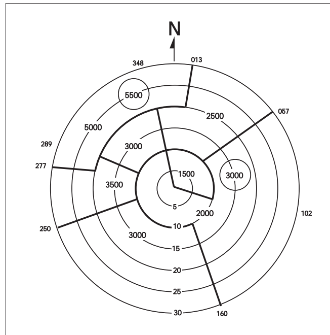
FIG ENR 1.5–28 Minimum Vectoring Altitude Charts
