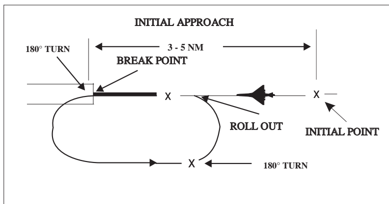
FIG ENR 1.5-40 Overhead Maneuver
