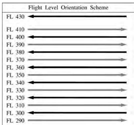
FIG ENR 1.1–30 Flight Level Orientation Scheme
