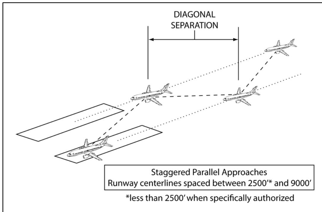
FIG ENR 1.5-33 Simultaneous (Parallel) Dependent Approaches
