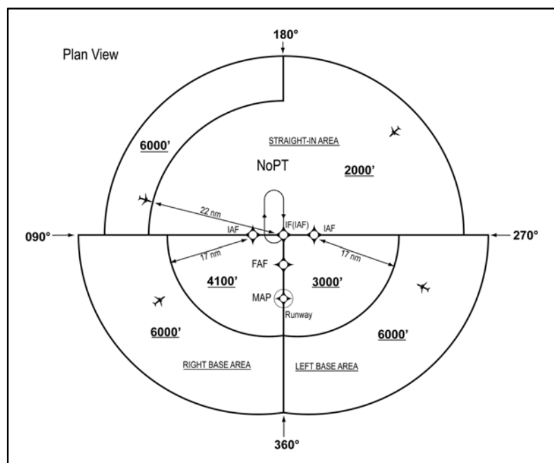
FIG ENR 1.5–22 Sectored TAA Areas
