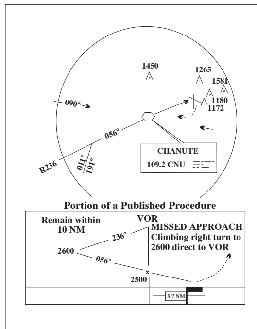
FIG 5-4-33 Missed Approach
