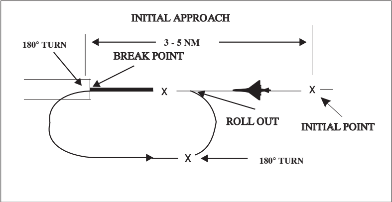
FIG 5-4-36 Overhead Maneuver
