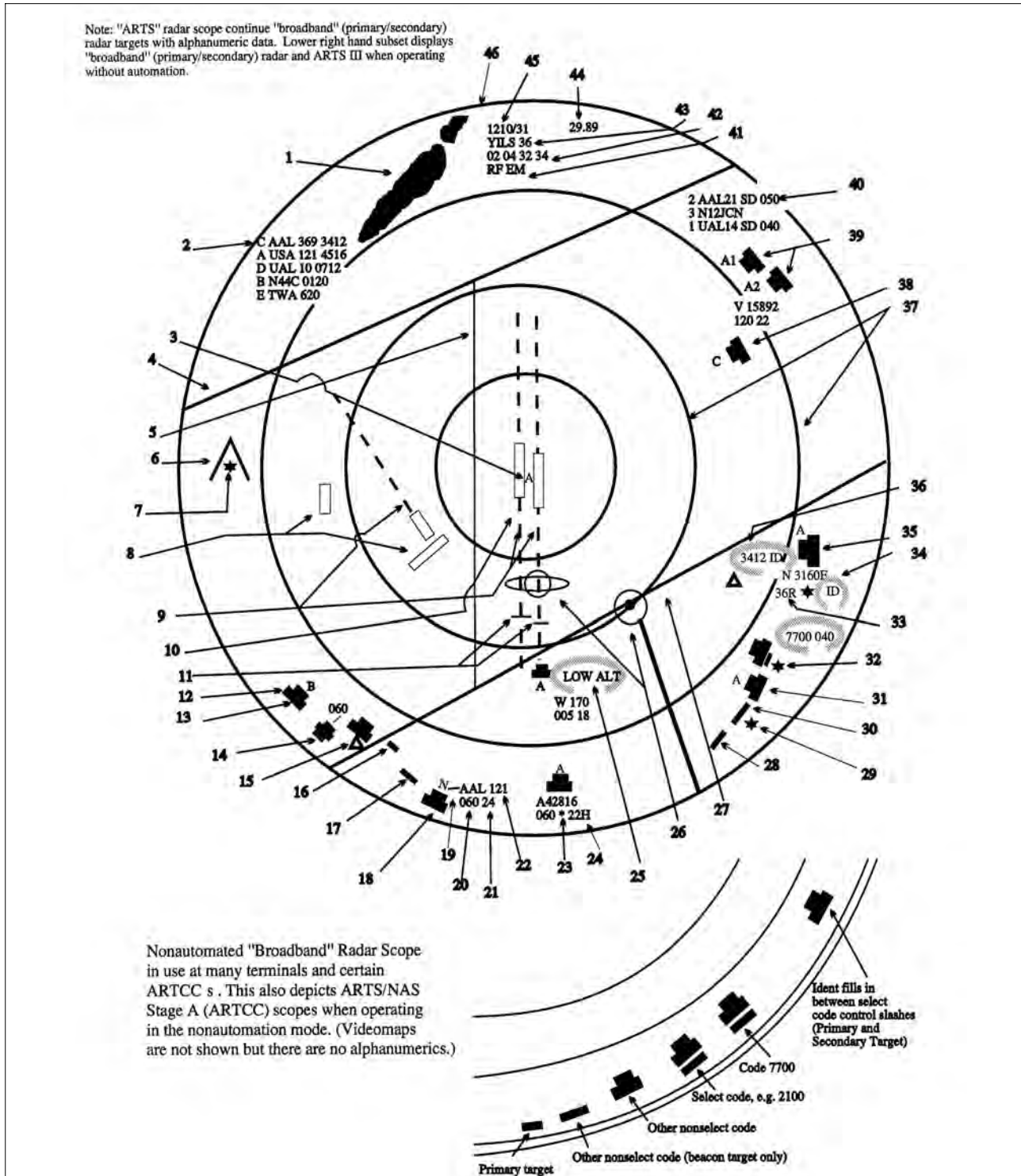
FIG 4-5-3 ARTS III Radar Scope With Alphanumeric Data
