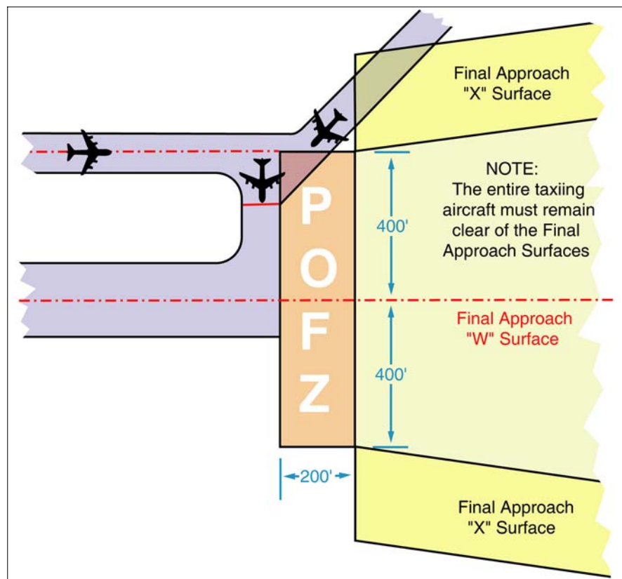
FIG 5-4-28 Precision Obstacle Free Zone (POFZ)
