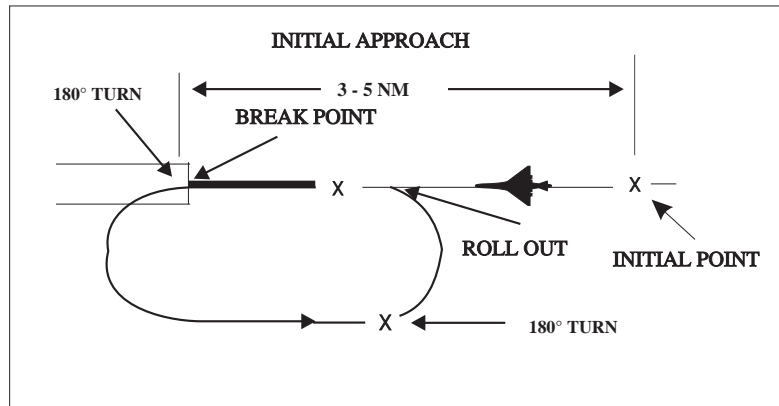
FIG 5-4-31 Overhead Maneuver
