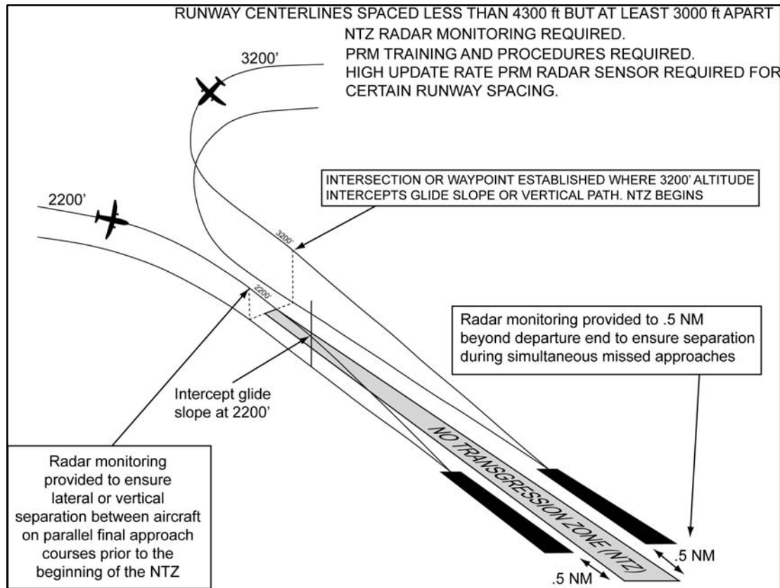
FIG 5-4-21 PRM Approaches Simultaneous Close Parallel
