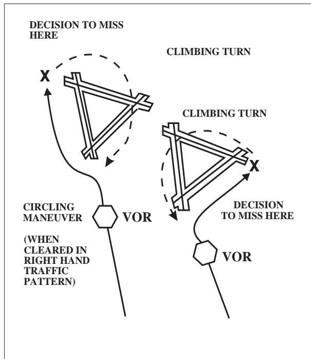
FIG 5-4-29 Circling and Missed Approach Obstruction Clearance Areas
