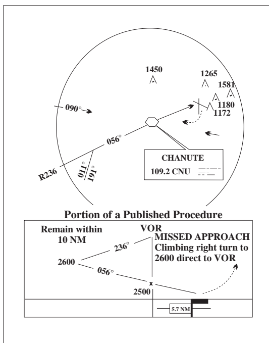
FIG 5-4-30 Missed Approach
