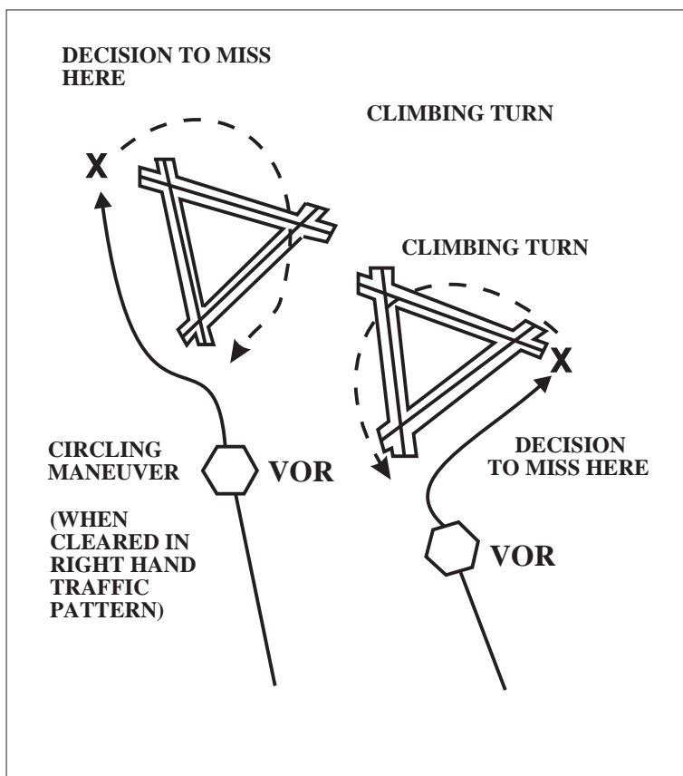
FIG ENR 1.5-42 Circling and Missed Approach Obstruction Clearance Areas
