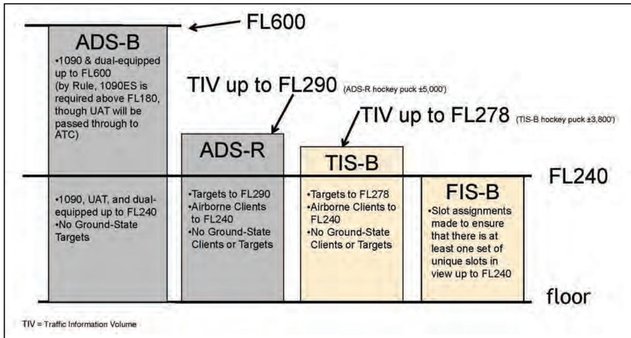
FIG ENR 1.1–36 Terminal – ADS-B/ADS-R/TIS-B/FIS-B Service Ceilings/Floors
