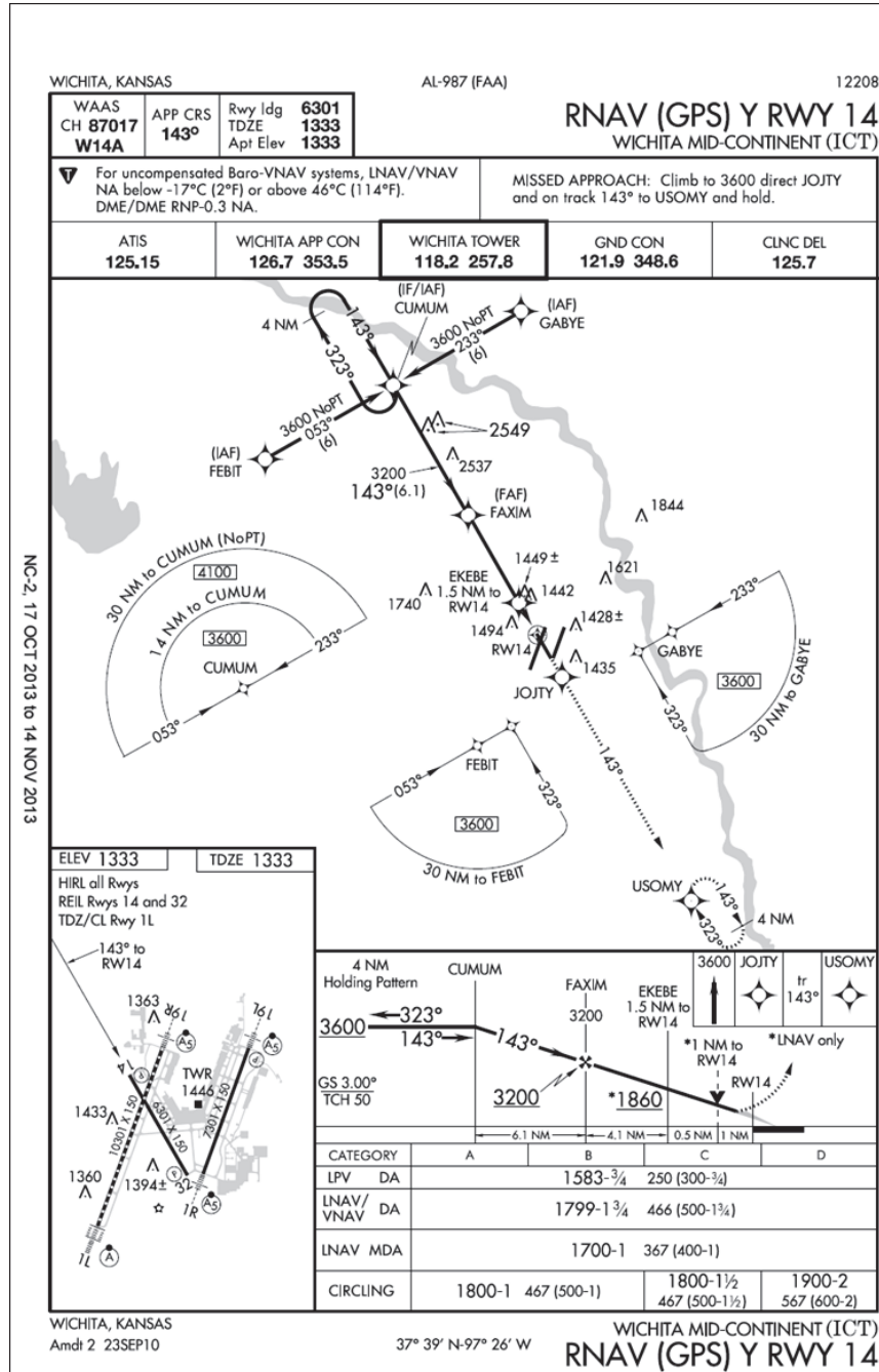
FIG ENR 1.5-22 RNAV (GPS) Approach Chart
