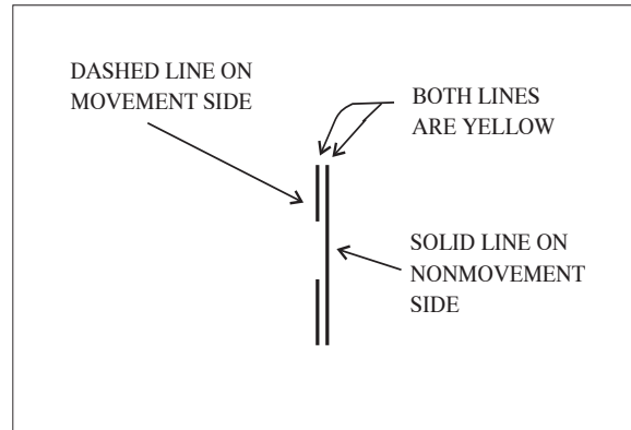
FIG AD 1.1-33 Nonmovement Area Boundary Markings
