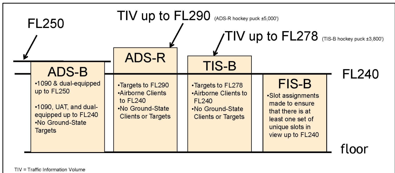
FIG ENR 1.1-37 Terminal – ADS-B/ADS-R/TIS-B/FIS-B Service Ceilings/Floors
