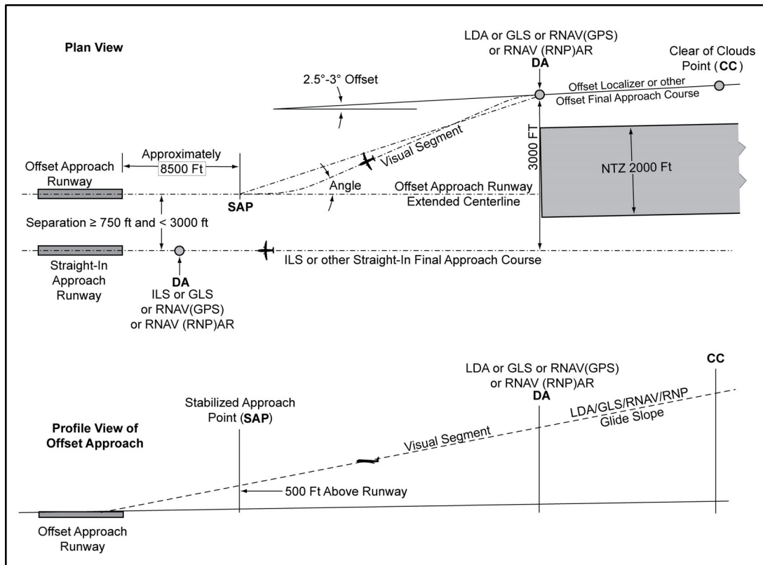
FIG ENR 1.5-36 SOIA Approach Geometry
