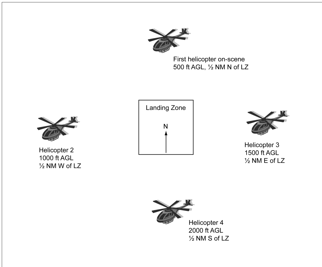
FIG ENR 6.2-9 EMS Multiple Helicopter LZ/Heliport Operation
