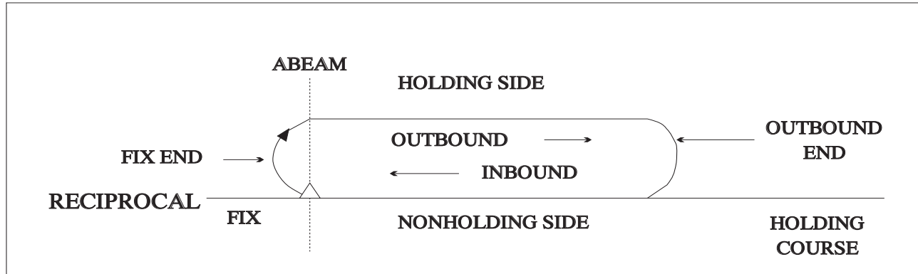
FIG ENR 1.5-1 Holding Pattern Descriptive Terms
