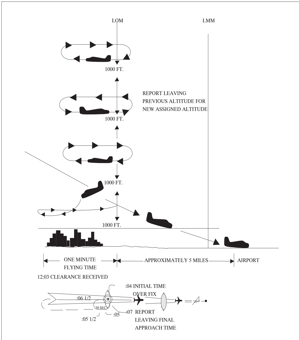
FIG ENR 1.5-37 Timed Approaches from a Holding Fix
