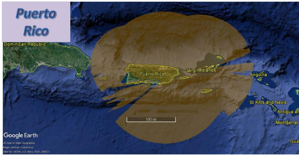
FIG ENR 1.6-10 Hawaii, Puerto Rico, and Guam with ADS-B Coverage at 1,500' AGL
