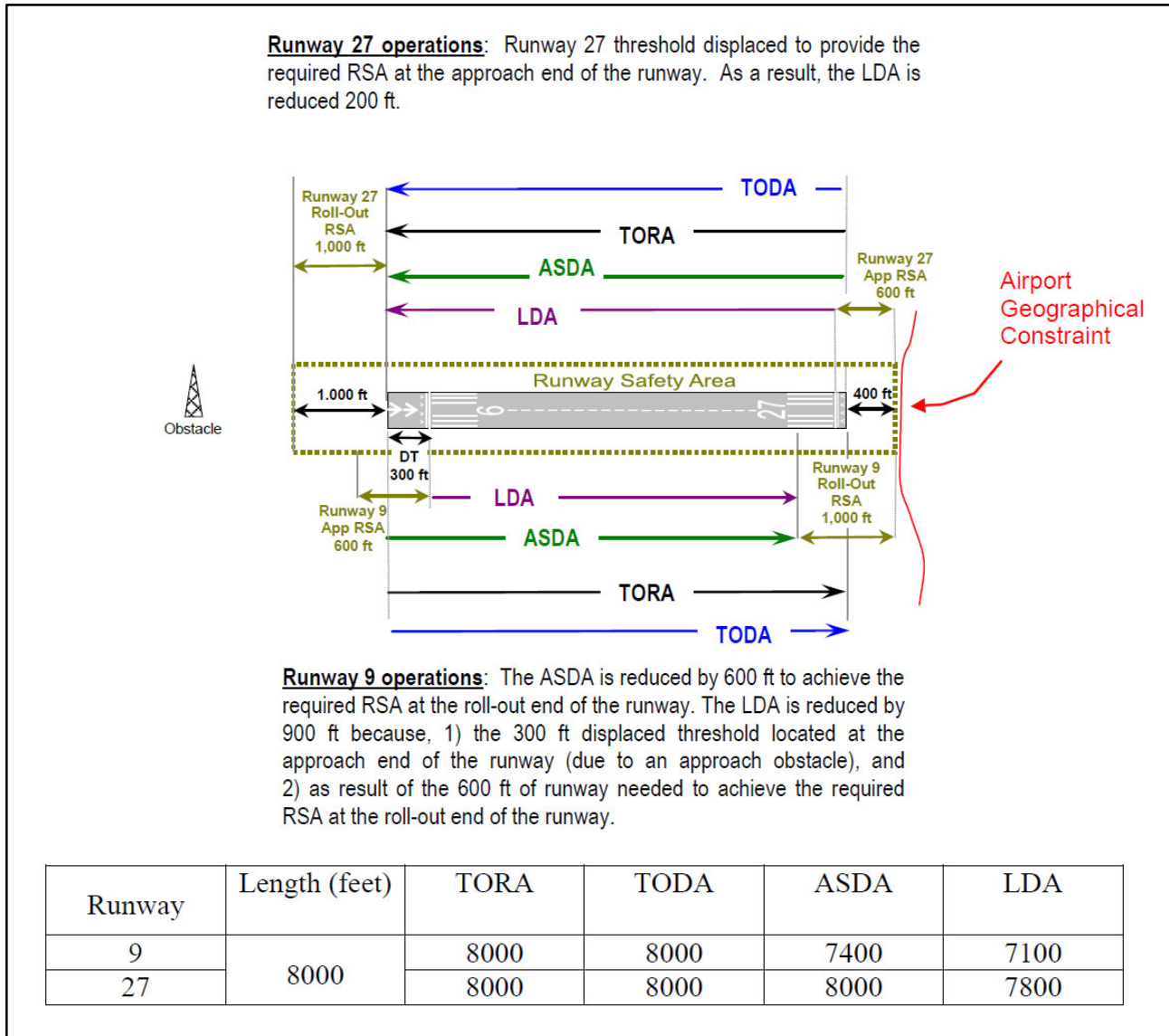
FIG ENR 1.1-6 Effects of a Geographical Constraint on a Runway's Declared Distances
