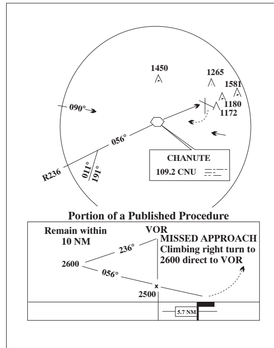
FIG ENR 1.5-41 Missed Approach
