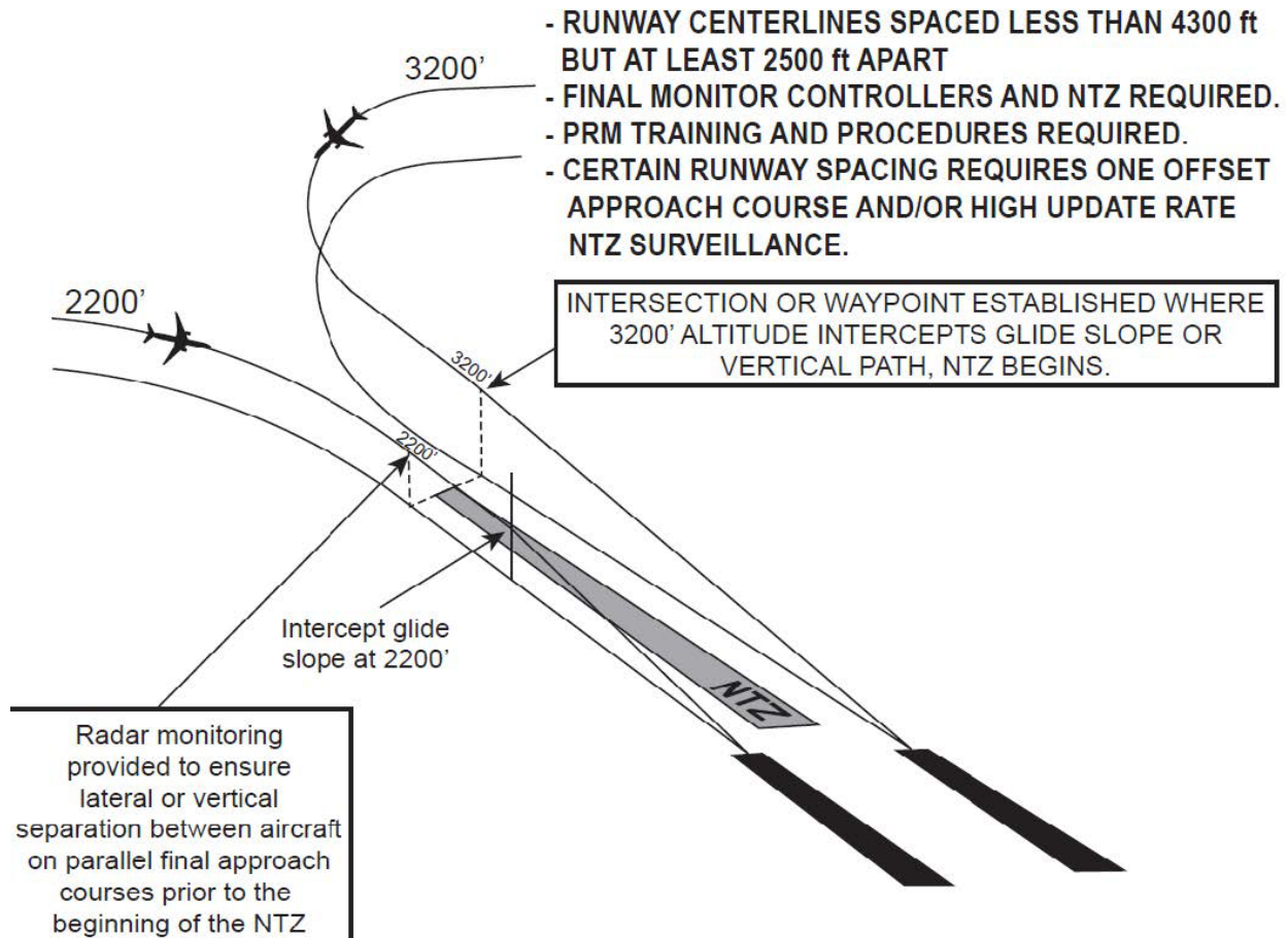
FIG ENR 1.5-34 PRM Approaches Simultaneous Close Parallel
