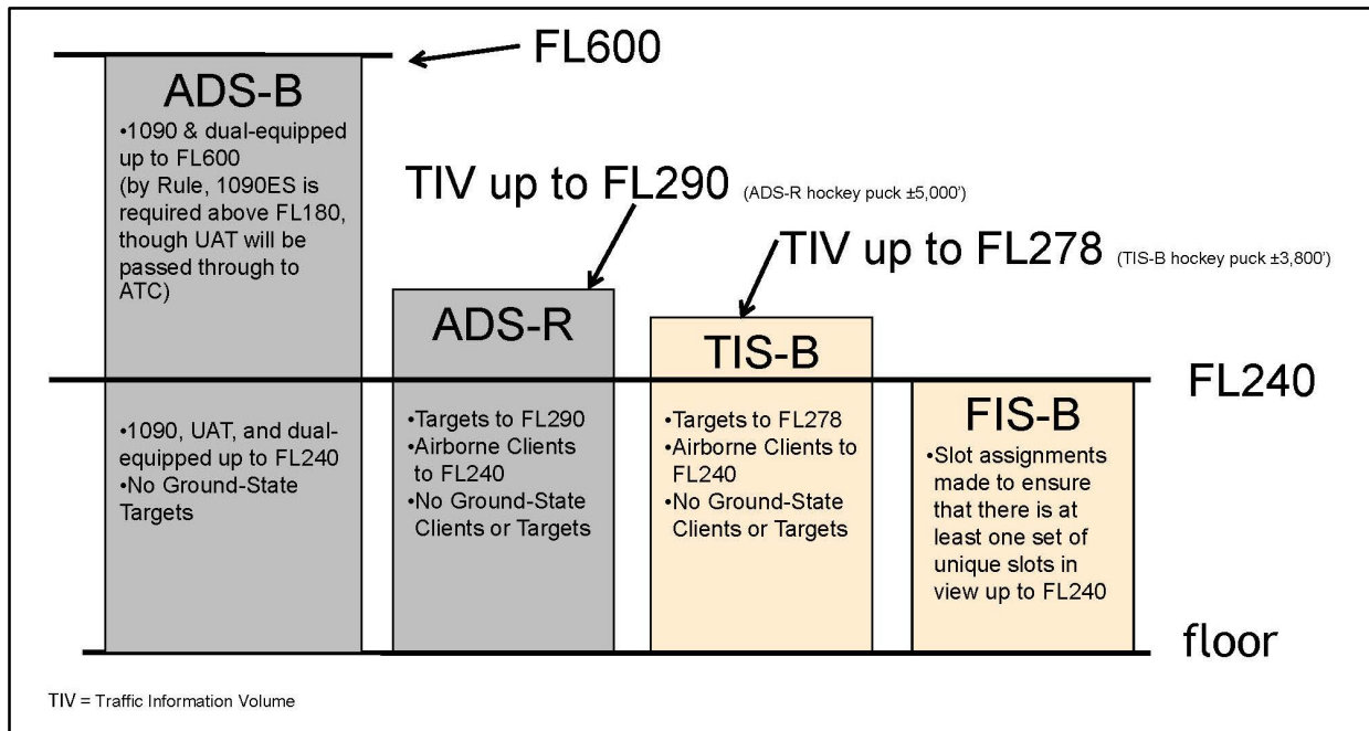
FIG ENR 1.1-37 Terminal – ADS-B/ADS-R/TIS-B/FIS-B Service Ceilings/Floors
