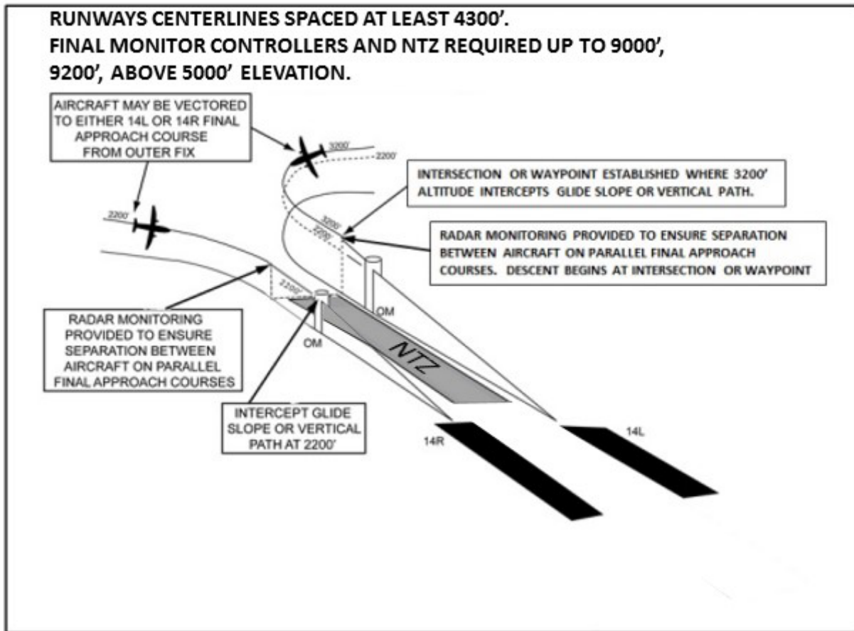
FIG ENR 1.5-33 Simultaneous Independent ILS/RNAV/GLS Approaches
