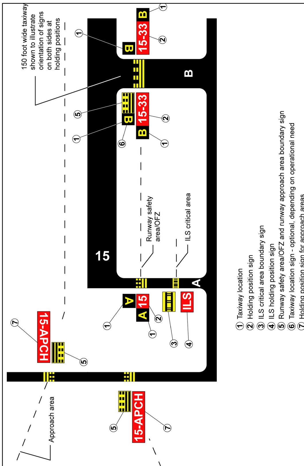
FIG AD 1.1-27 Taxiways Located in Runway Approach Area
