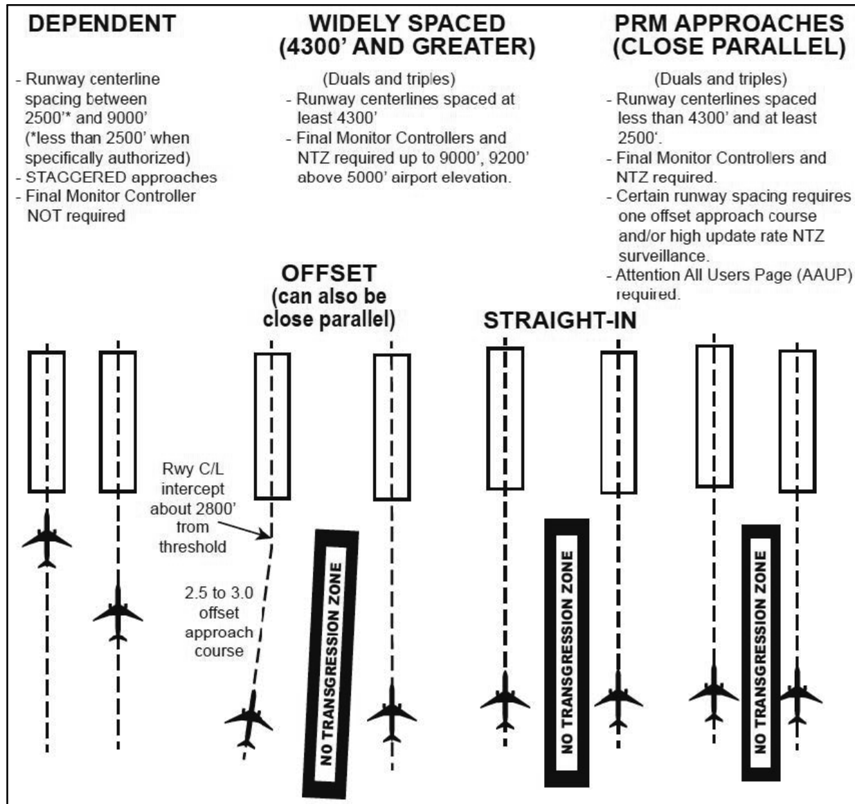
FIG ENR 1.5-33 Simultaneous Approaches (Approach Courses Parallel and Offset between 2.5 and 3.0 degrees)
