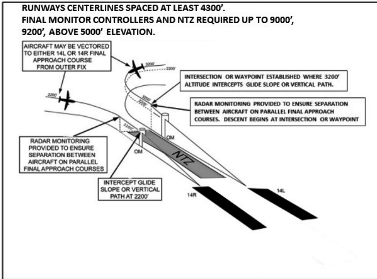
FIG ENR 1.5–35 Simultaneous Independent ILS/RNAV/GLS Approaches
