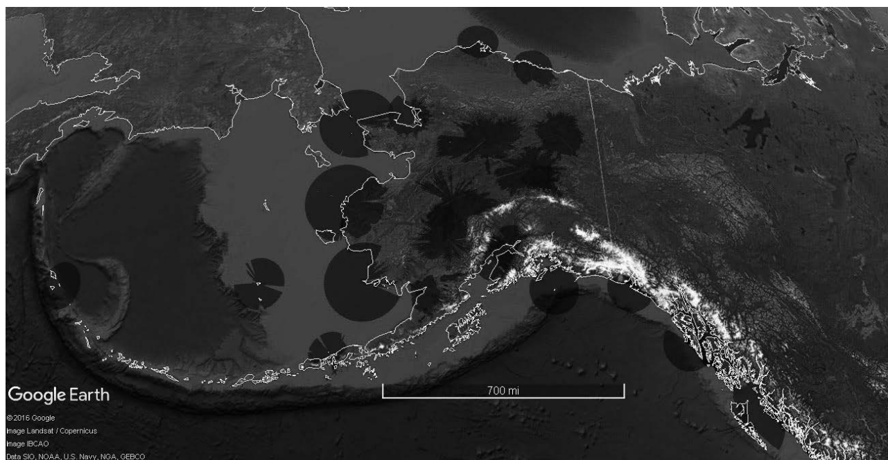
FIG ENR 1.6-5 Alaska with SSR Coverage at 1,500' AGL
