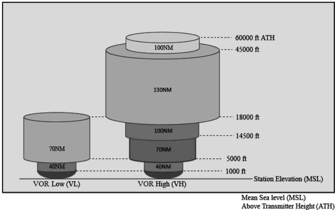
FIG GEN 3.4-4 New VOR Service Volumes
