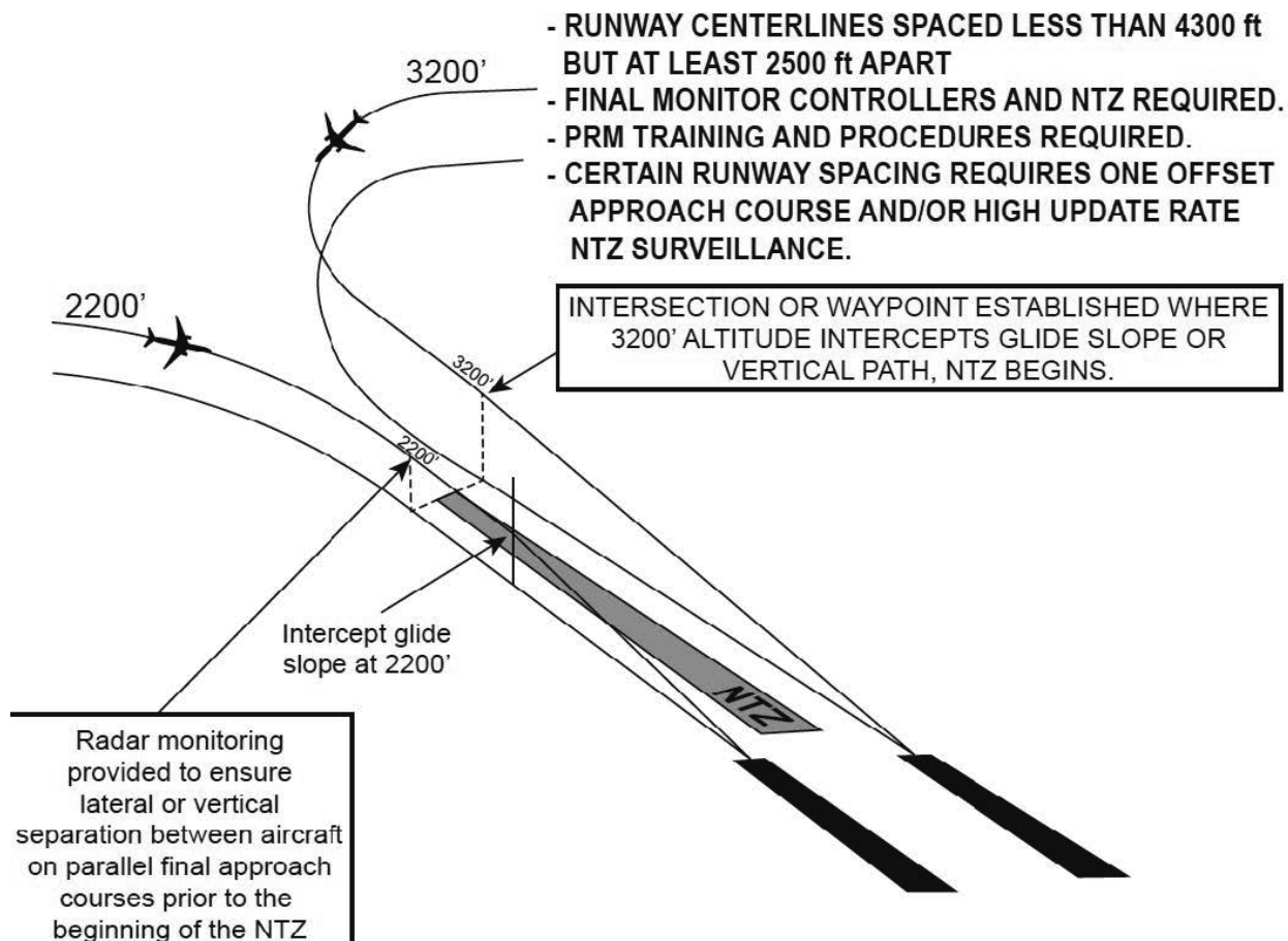
FIG ENR 1.5-36 PRM Approaches Simultaneous Close Parallel
