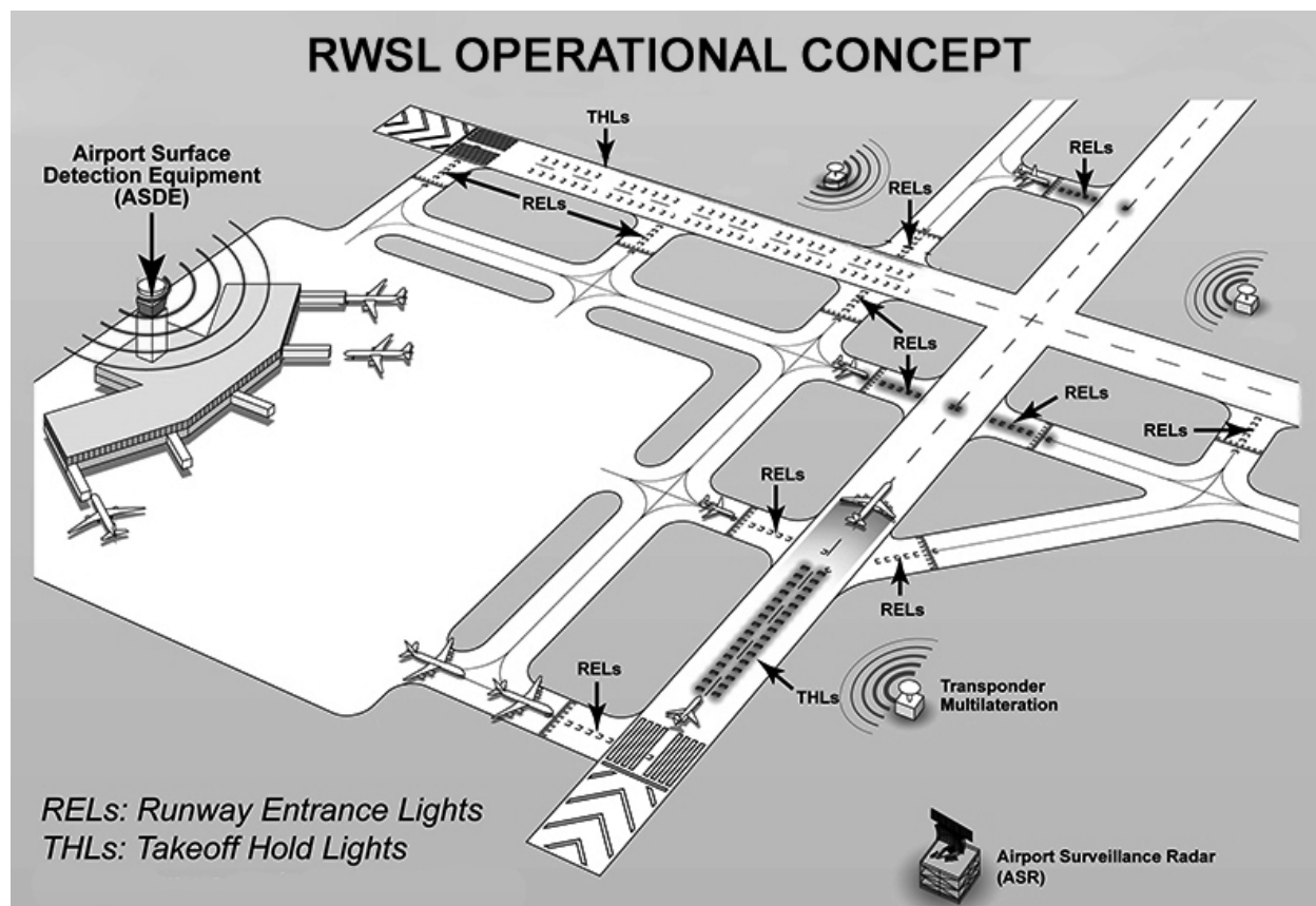
FIG AD 1.1-9 Runway Status Light System
