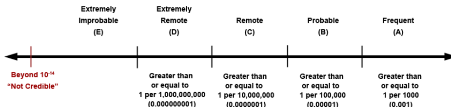
Figure 3.6: Likelihood Continuum
