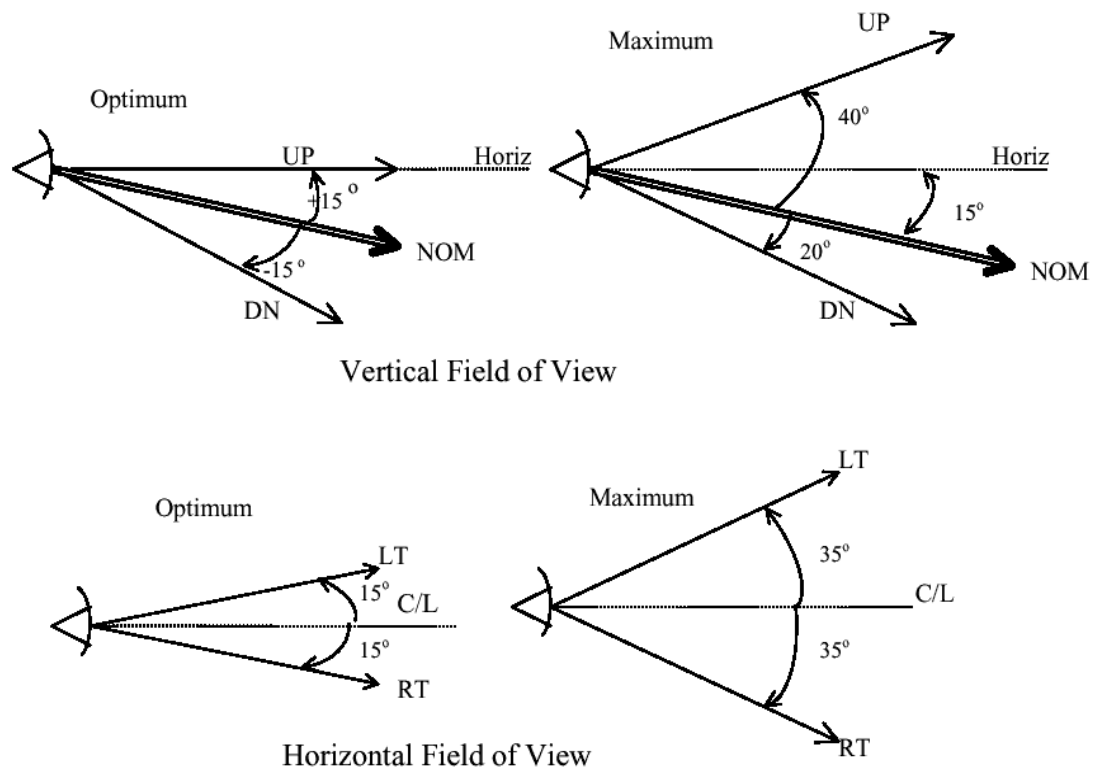
Figure C-2. Primary Field-of-View
