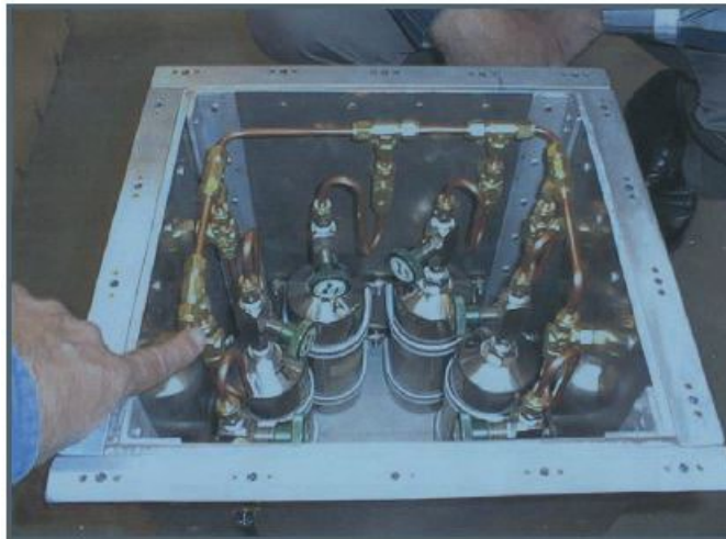
Figure E-2. Vacuum Bottle Sample System Installed on an NTSB Test Aircraft
