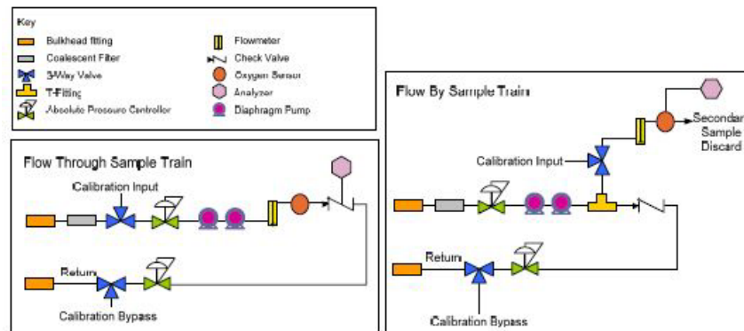
Figure E-1. Block Diagrams of Flow Through and Flow Bypass Sample Systems
