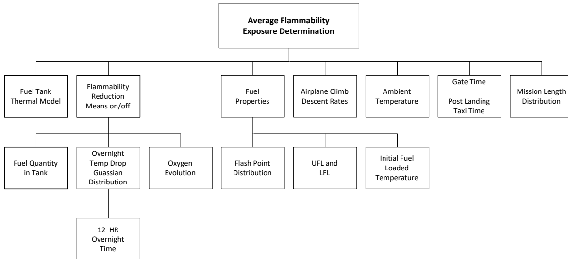
Figure 1. Monte Carlo Parameters to Determine Fuel Tank Flammability
