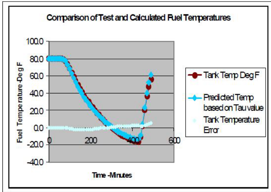
Figure D-1. Comparison of Test and Calculated Fuel Temperatures
