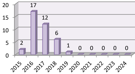
7. Wind
