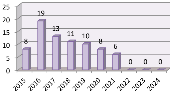
3. Directional Control
