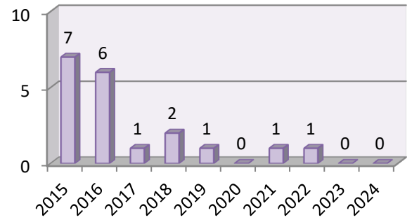
9. Canopy/Door Opened
