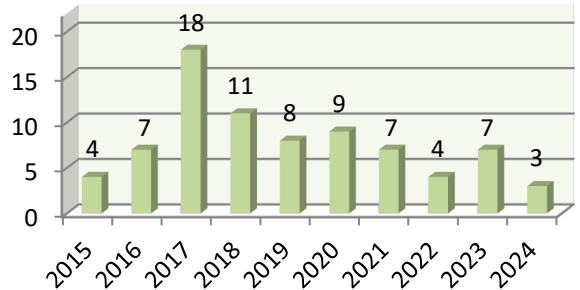
4. Collision w/Obstacles
