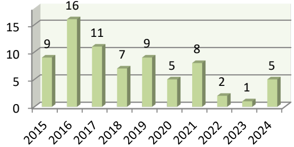
5. LOC Ground
