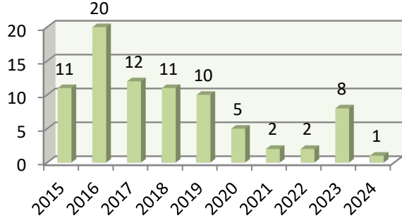
3. Runway Excursion
