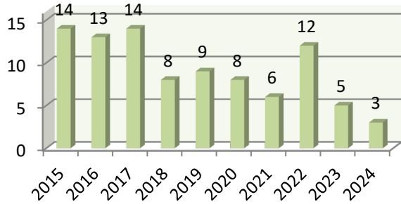
2. LOC In-Flight
