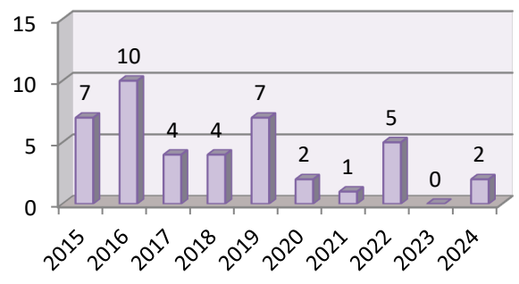
6. Stall/Spin/Spiral
