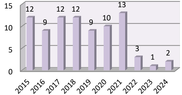
4. Hard/Bounced Landing
