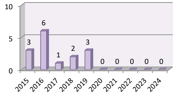
10. Improper Airspeed
