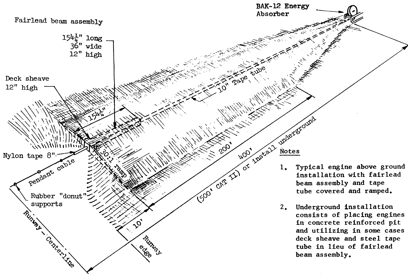
FIGURE 6. BAK-12 ROTARY FRICTION ENERGY ABSORBER/FAIRLEAD BEAM ASSEMBLY OR DECK SHEAVE/PENDANT SUPPORTED PENDANT CATCHING DEVICE
