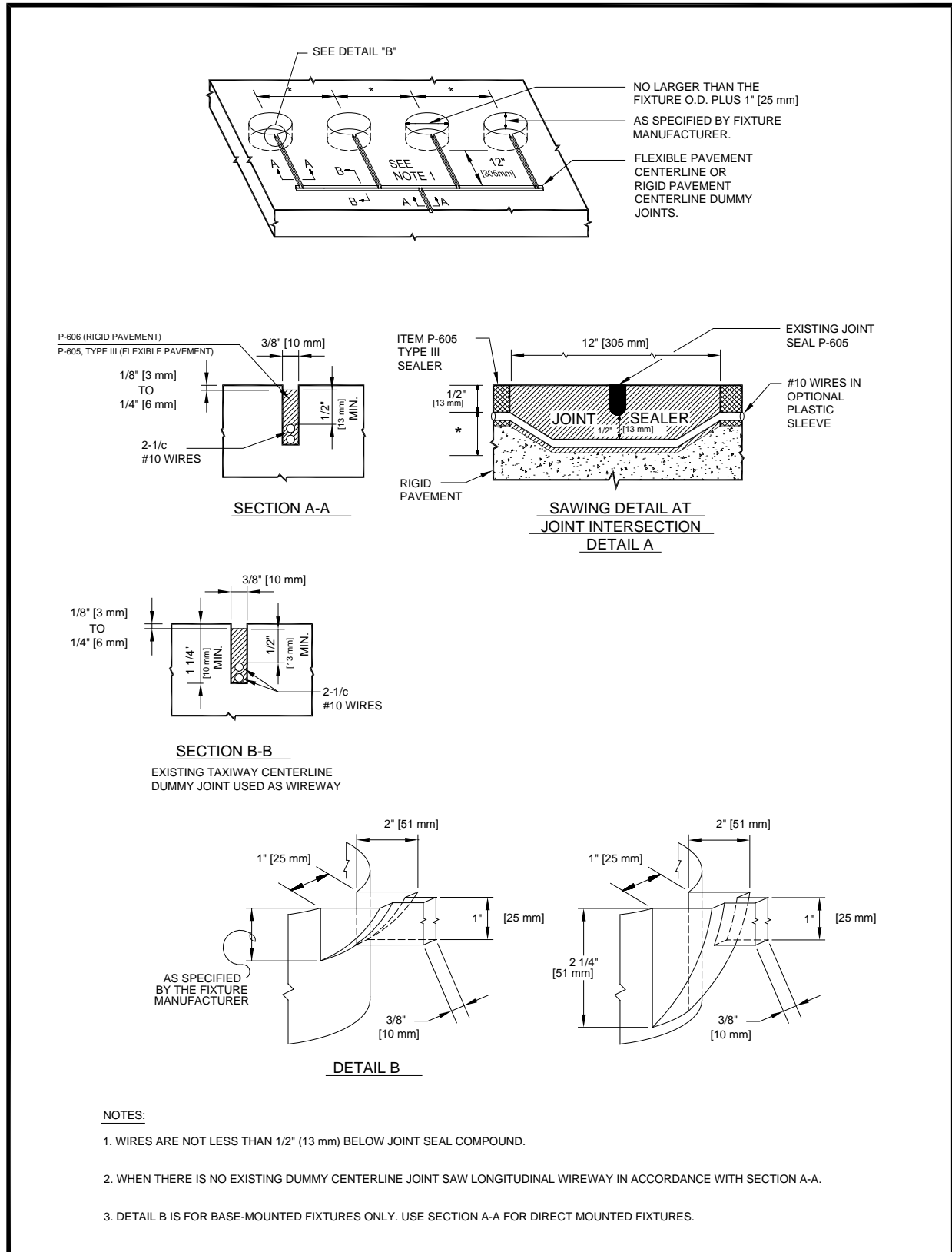
Figure A-106. Sawing and Drilling Details for In-Pavement Taxiway Centerline Lights
