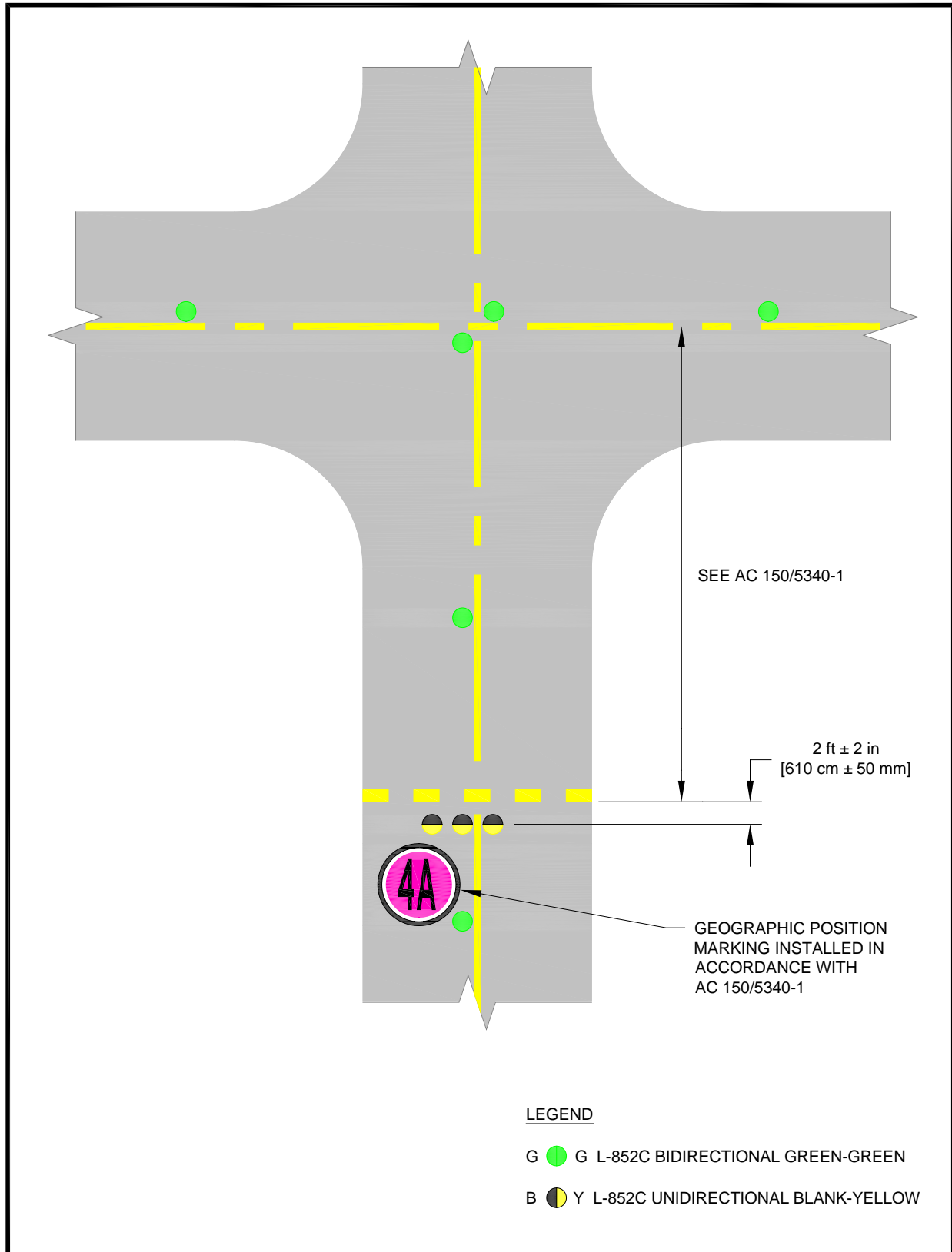
Figure A-53. Clearance Bar Configuration at a Low Visibility Hold Point
