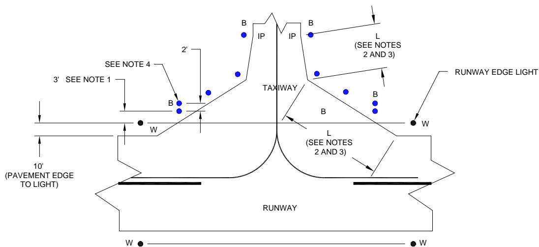
b. Sample Layout for Runway and Taxiway Intersection ( L = 10' \leq L \leq 40' )
