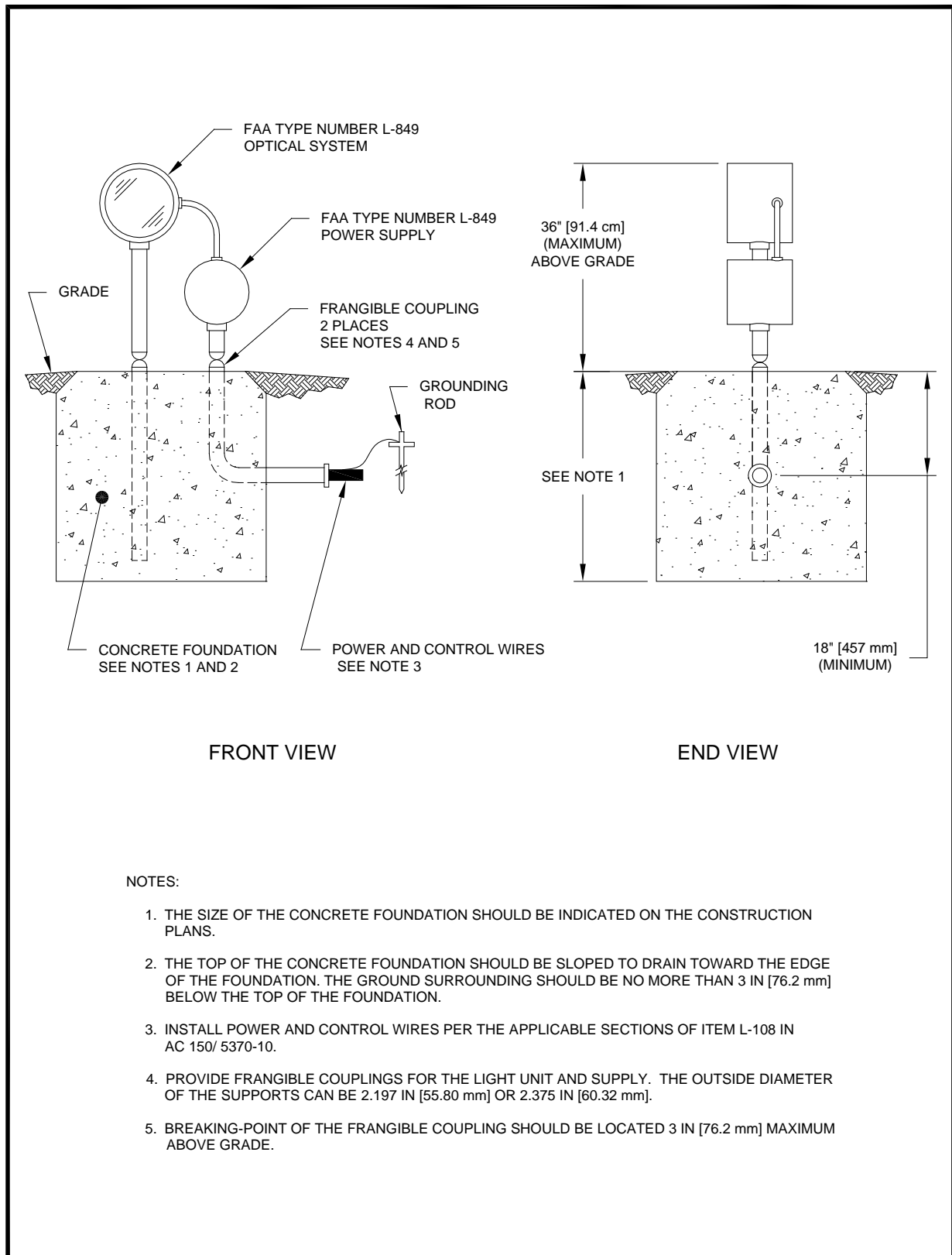
Figure A-93. Typical Installation Details for Runway End Identifier Lights (REILs)
