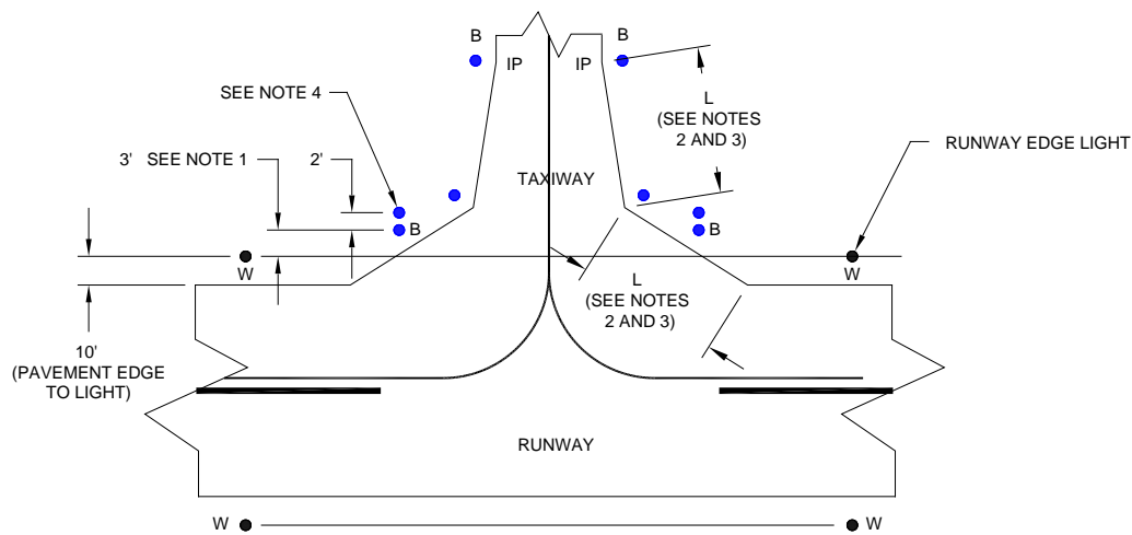
a. Sample Layout for Runway and Taxiway Intersection ( L = 3' \leq L < 10' )
