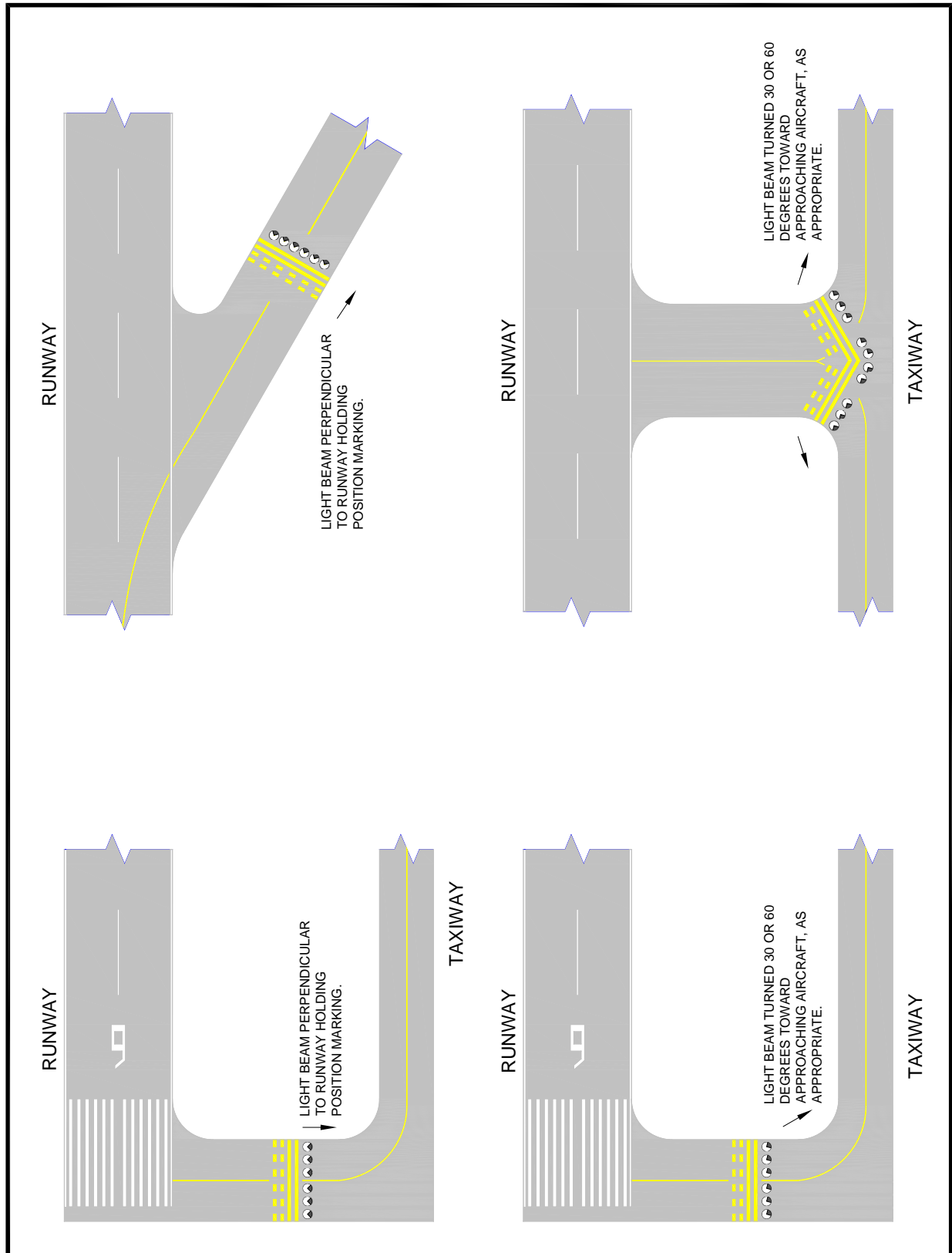
Figure A-52. Typical Light Beam Orientation for In-Pavement RGLs and Stop Bars
