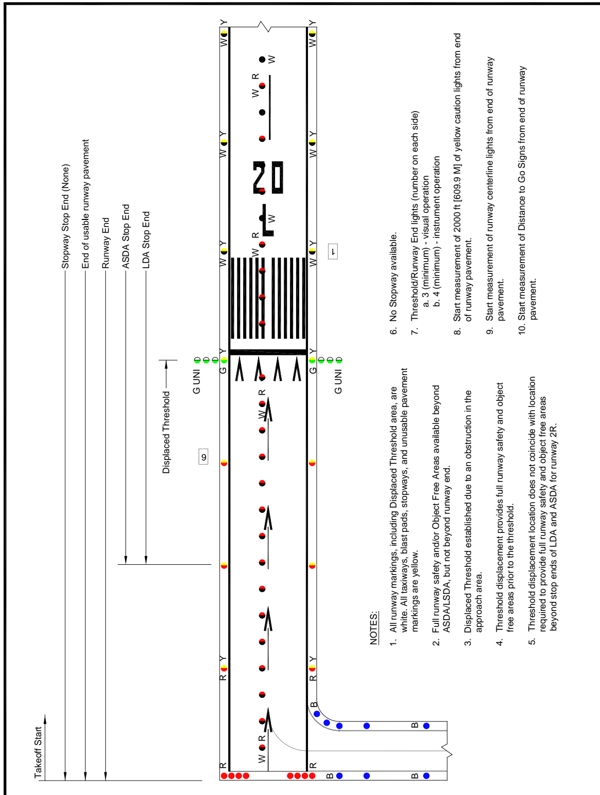
Figure H-8. Lighting for Runway with Displaced Threshold Not Coinciding with Opposite Runway End (Legacy Figure 10)
