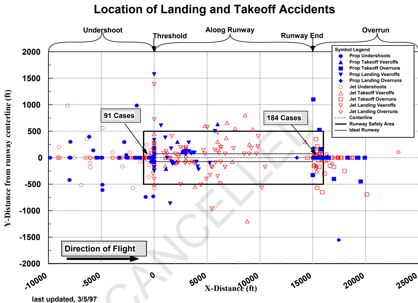
Figure A-2.1. Location of Landing and Takeoff Accidents (Source: ALPA)
