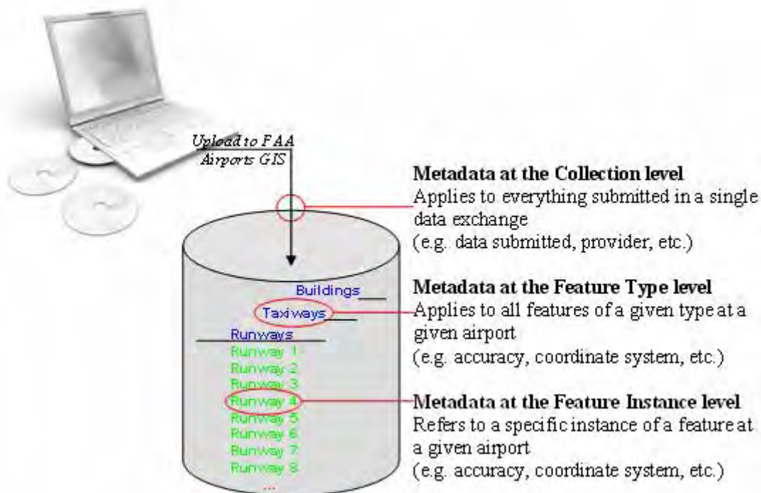
Figure 3-14. MetaData elements have different levels of aggregation.
