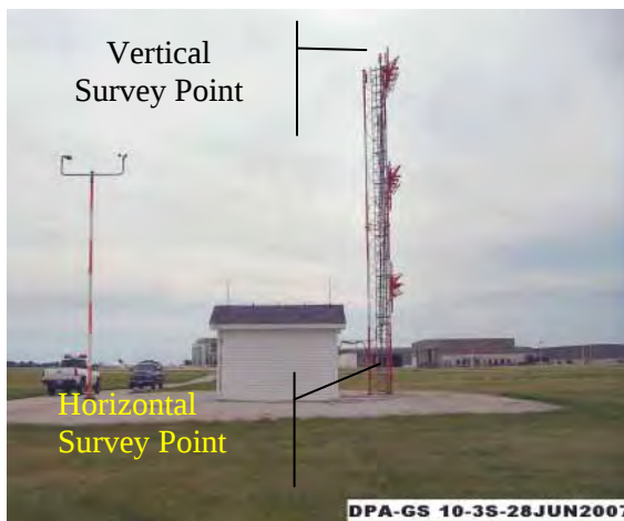
Figure 1-4. Illustrates the documentation of a glideslope antenna from different perspectives.
