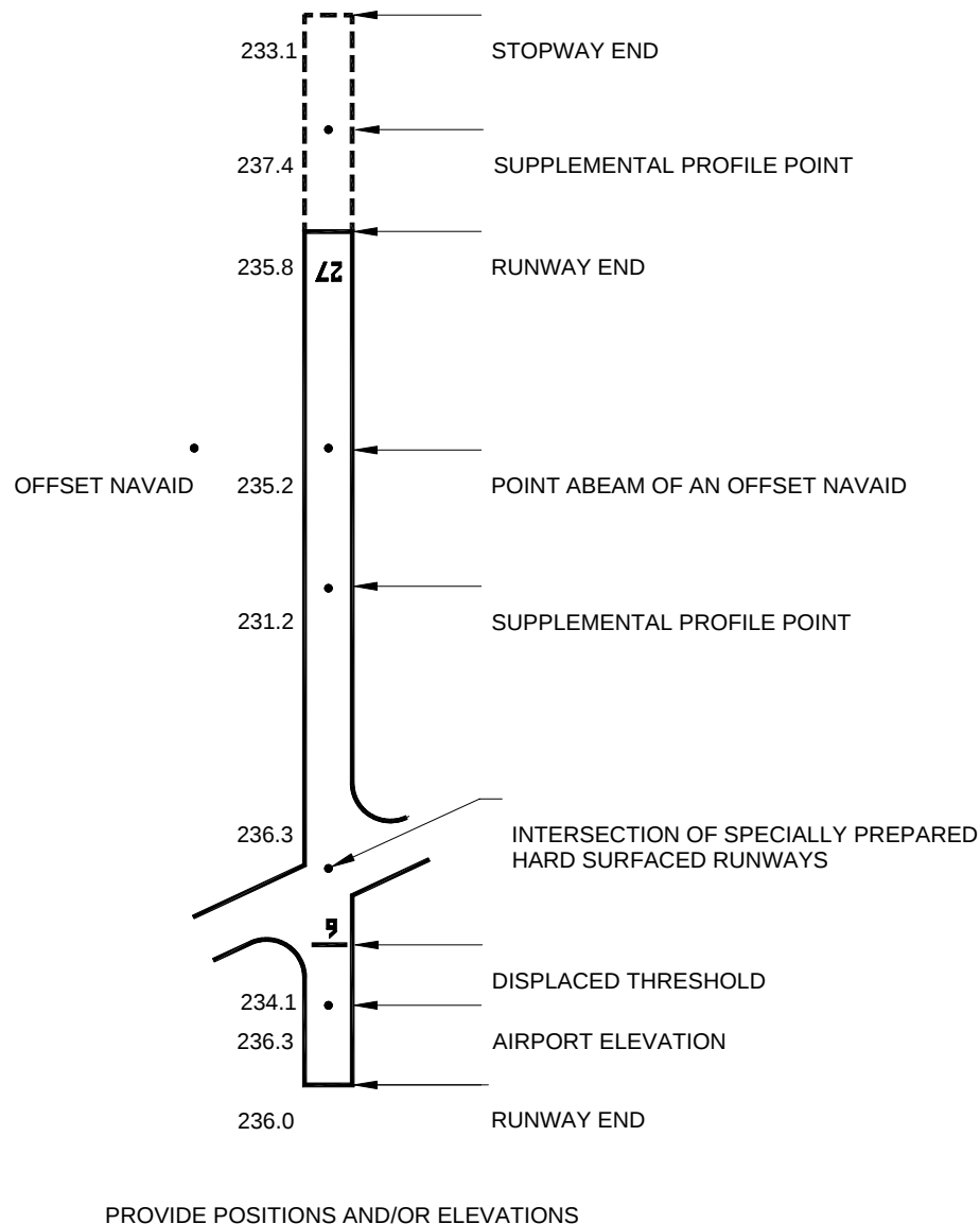
Figure 2-1. Depicts some of the required points and elements of a runway or stopway.
