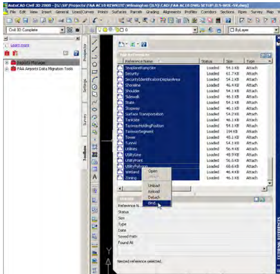
Figure 4-3. Binding Multiple Legacy Files.
