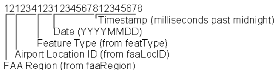
Figure 3-13. Format for globally unique primary keys.
