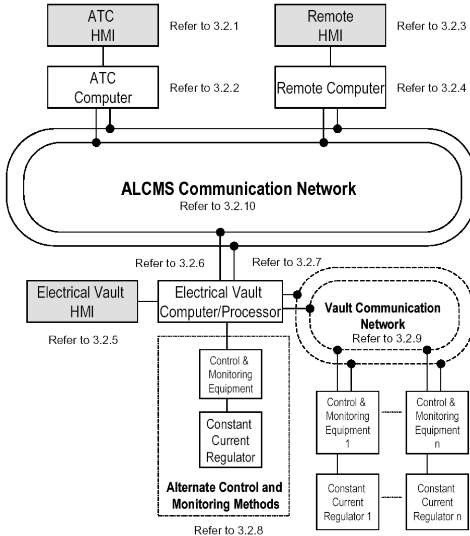
Figure 142. ALCMS Block Diagram
