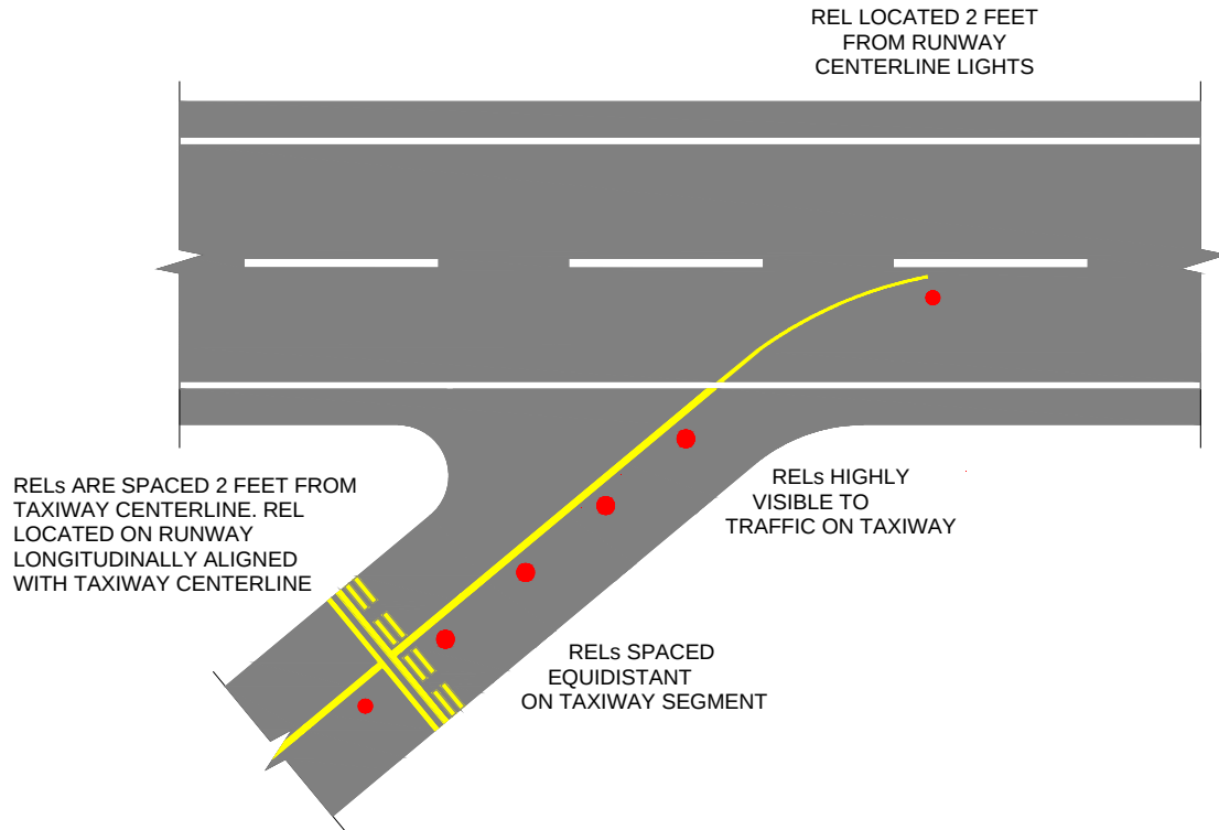
Figure 144. Angled Configuration
