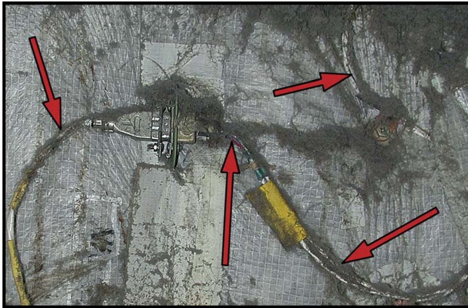
Figure 1: EWIS Contaminated with Dust and Dirt
