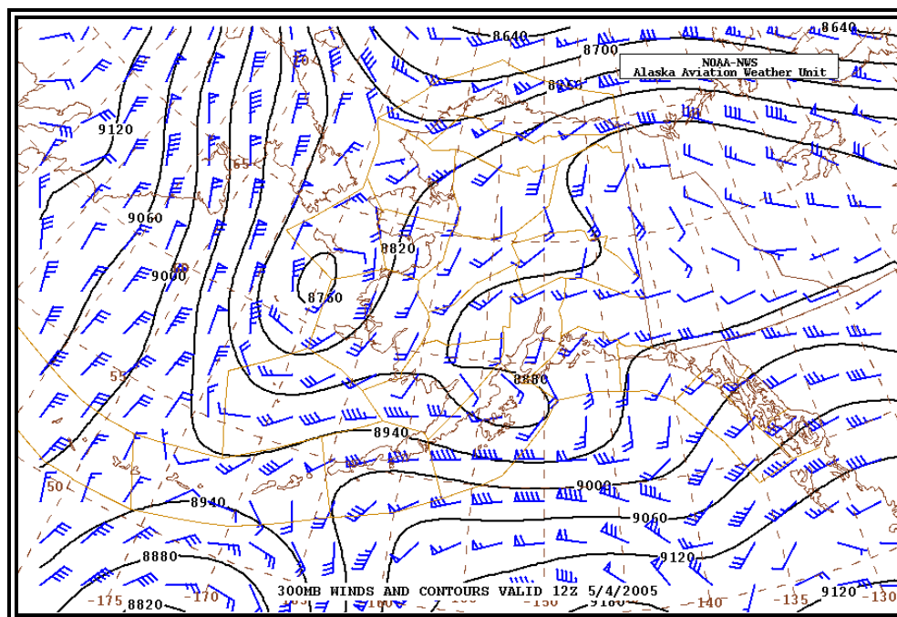
Figure 5-53. Alaskan Initial Geopotential Heights and Winds Chart - 300MB Winds and Contours Chart Example
