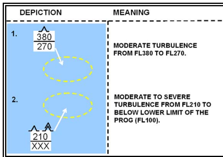
Figure 8-25. Mid-Level SIGWX Chart Turbulence Examples
