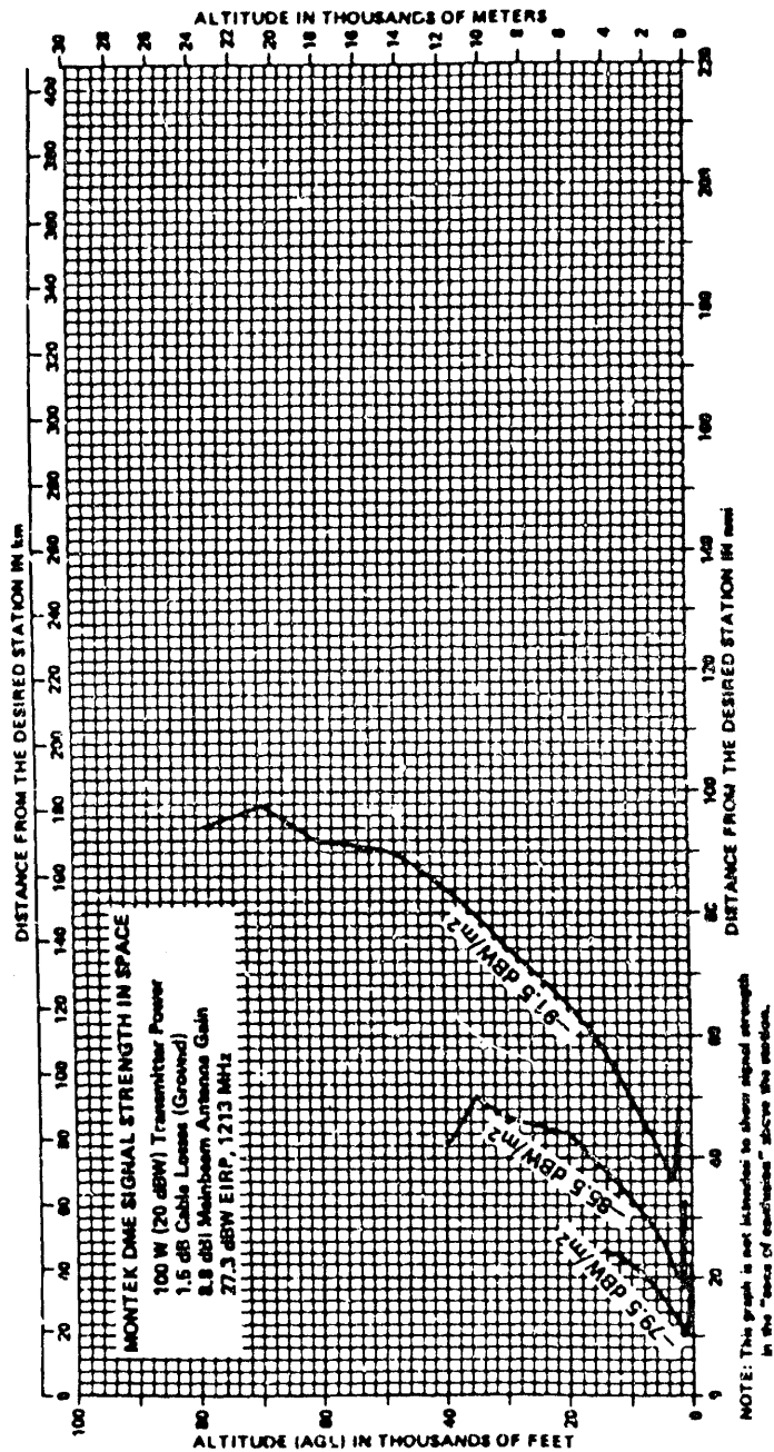
FIGURE 7. MCNTEK DME SIGNAL STRENGTH IN SPACE - LONG RANGE
