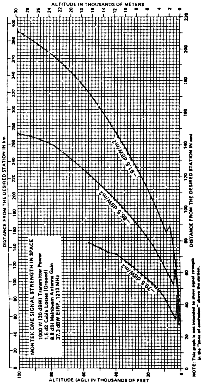
FIGURE 6. MONTEK DME SIGNAL STRENGTH IN SPACE - LONG RANGE
