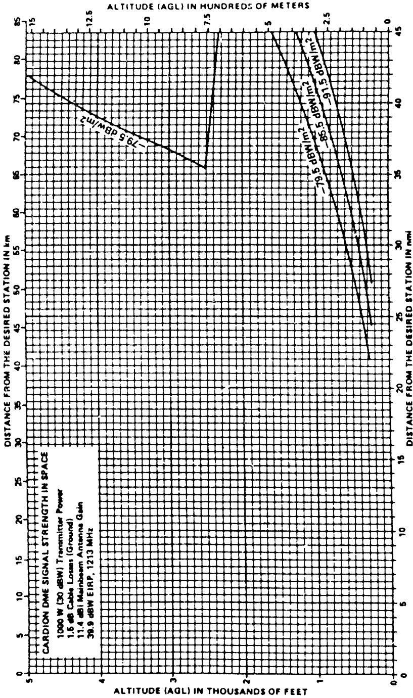
FIGURE 10. CARDION DME SIGNAL STRENGTH IN SPACE - SHORT RANGE
