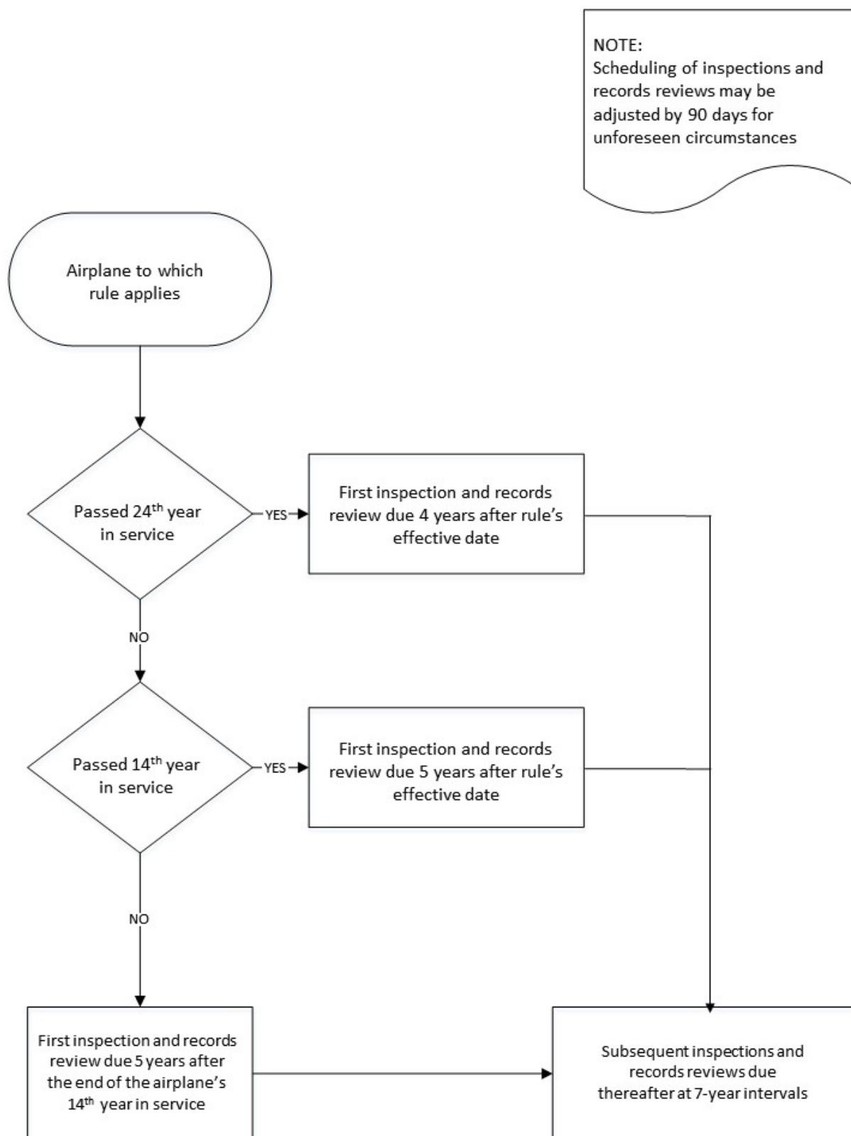
FIGURE 2. DECISION LOGIC—INITIAL INSPECTIONS AND RECORDS REVIEW DUE DATE
