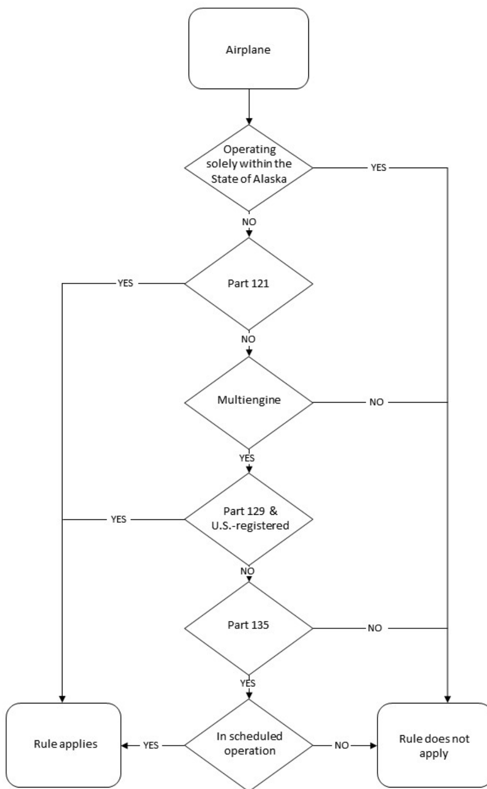
FIGURE 1. DECISION LOGIC—APPLICABILITY OF INSPECTIONS AND RECORDS REVIEW
