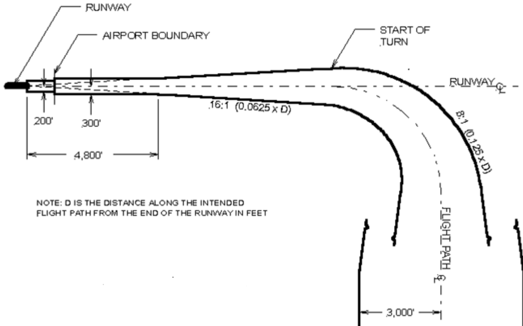
FIGURE 1-2. TURNING DEPARTURES
