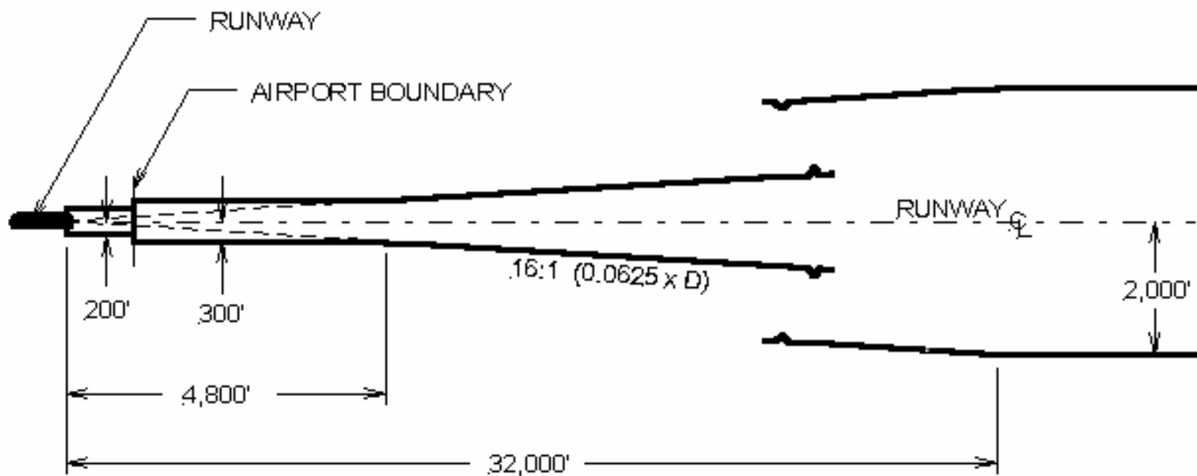
FIGURE 1-1. STRAIGHT-OUT DEPARTURES
