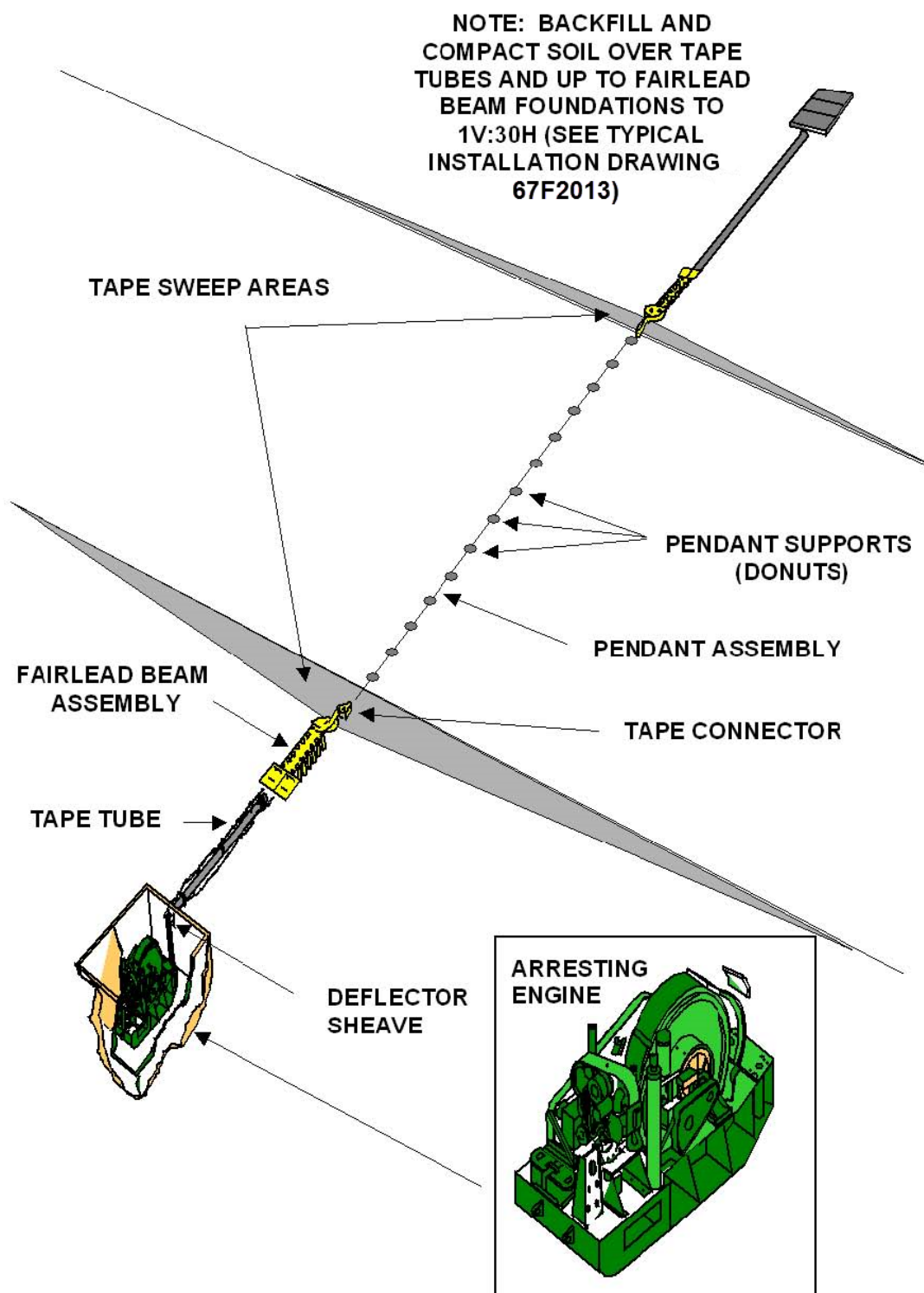
Figure A-2. BAK-12 Aircraft Arresting System.
