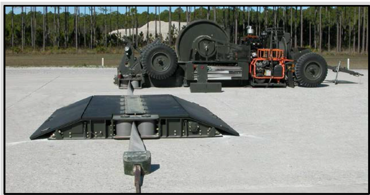
Figure A-22. Mobile Aircraft Arresting System (MAAS) with Mobile Runway Edge Sheave (MRES) in front
