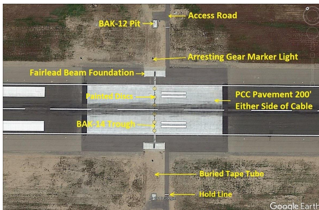
Figure A-20. Plan View of Typical BAK-12/14 (or Type H) Installation
