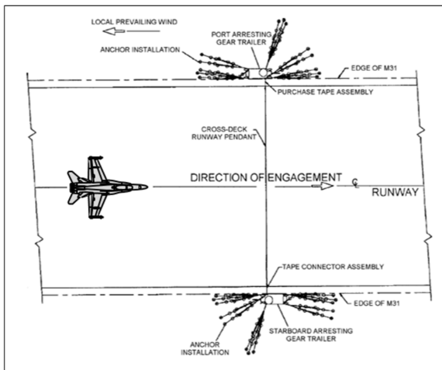
Figure A-10. MCEAGS Installation Diagram (Typical)
