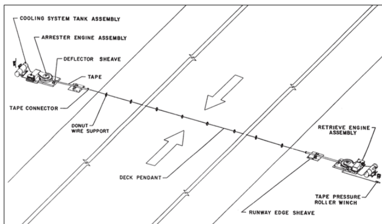
Figure A-11. E-28 Emergency Runway Arresting Gear Installation Diagram
