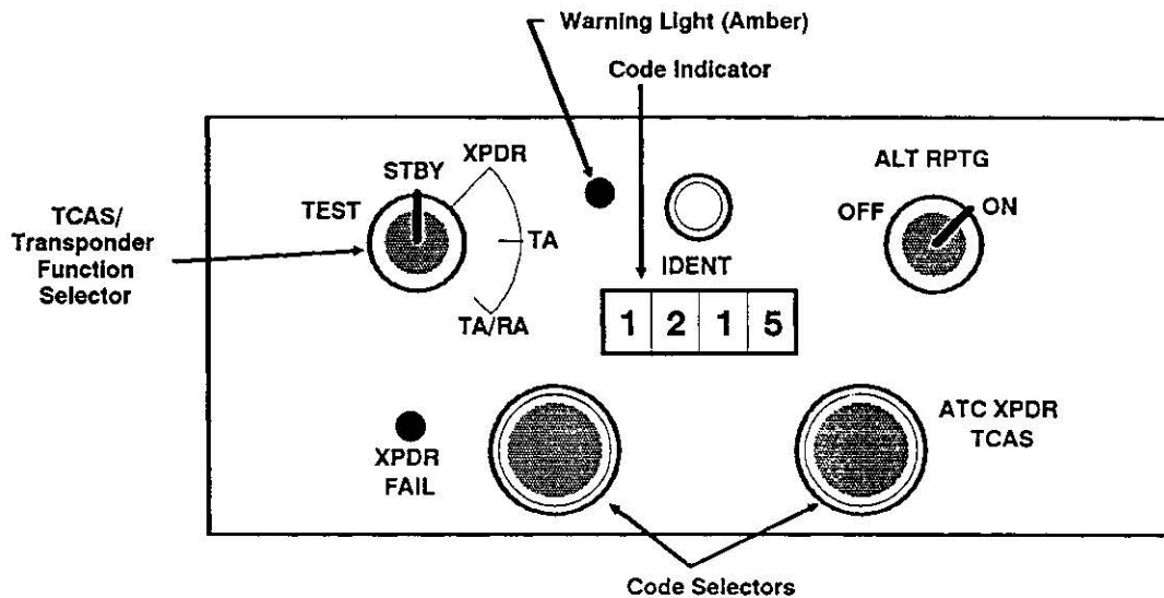
Figure 1: TCAS/Transponder Control Panel (Example).
