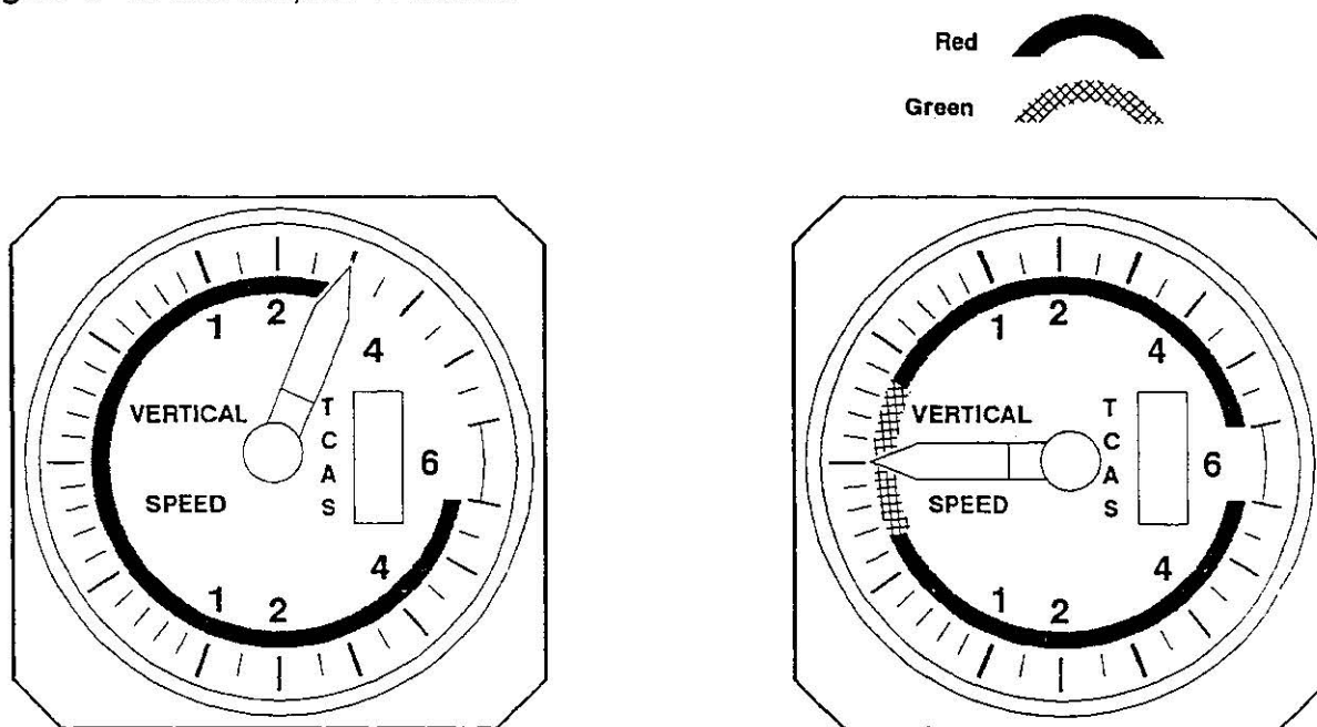
Figure 4: TCAS II Examples - Preventive.
