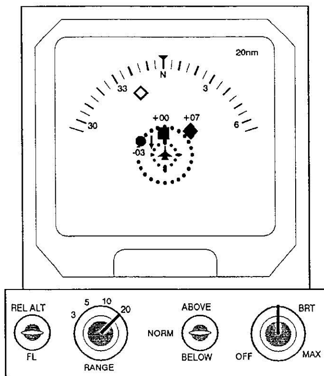
Figure 2: TCAS II - Traffic Display (Example).
