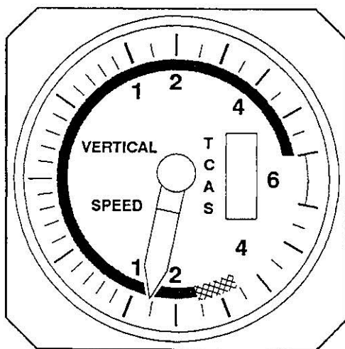
(c) -Corrective INCREASE DESCENT.
