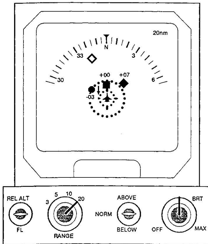
Figure 2: TCAS II - Traffic Display (Example) (Con't).
