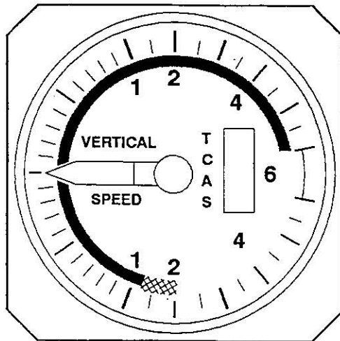
(a) Corrective DESCEND.
