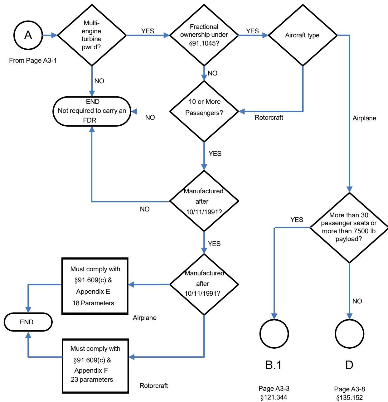
FIGURE 3-2. PART 91 FLIGHT RECORDER PARAMETER REQUIREMENTS § 91.609
