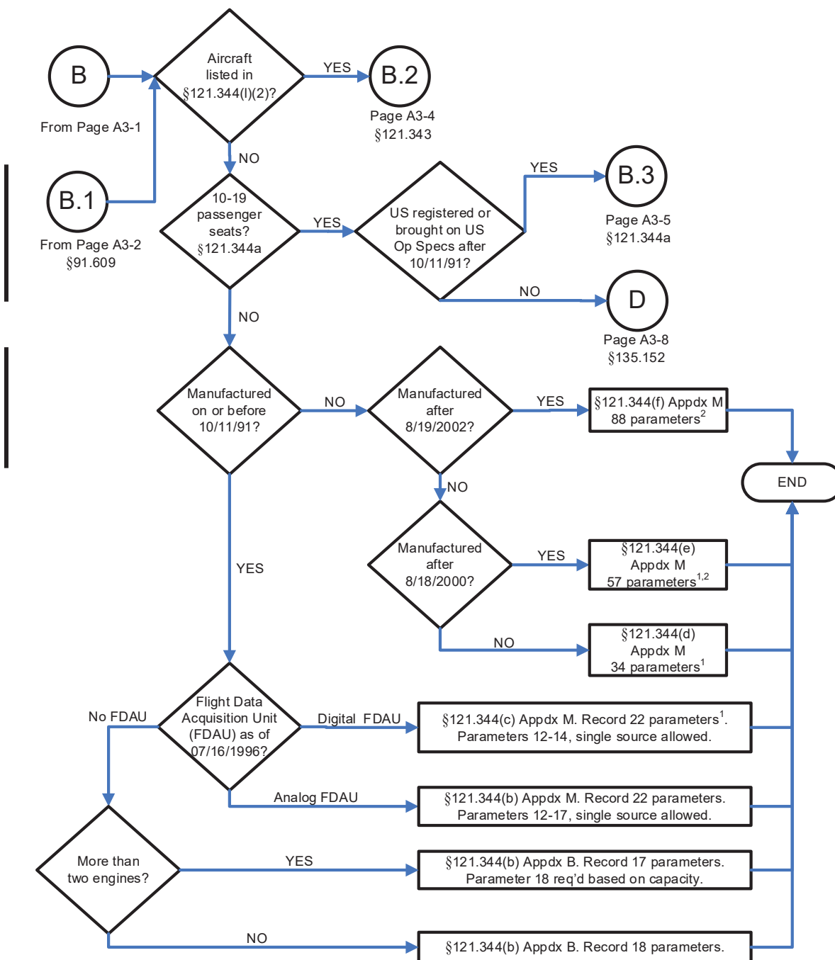
FIGURE 3-3. PART 121 FLIGHT RECORDER PARAMETER REQUIREMENTS § 121.344
