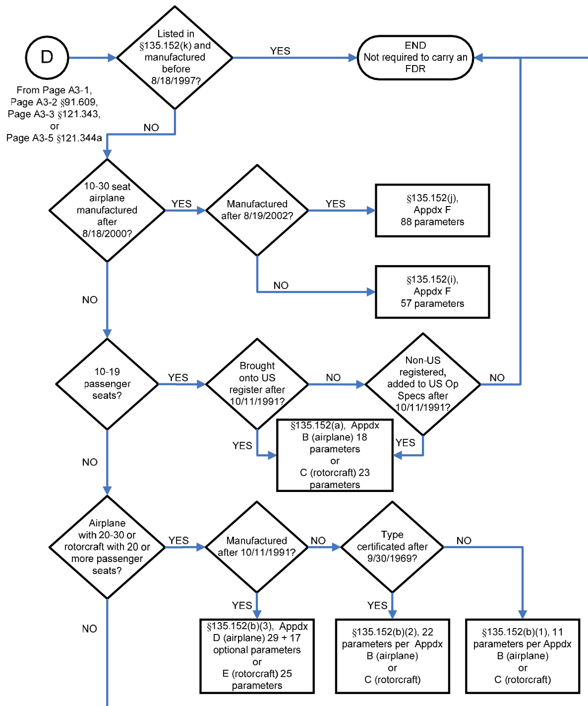
FIGURE 3-8. PART 135 FLIGHT RECORDER PARAMETER REQUIREMENTS § 135.152
