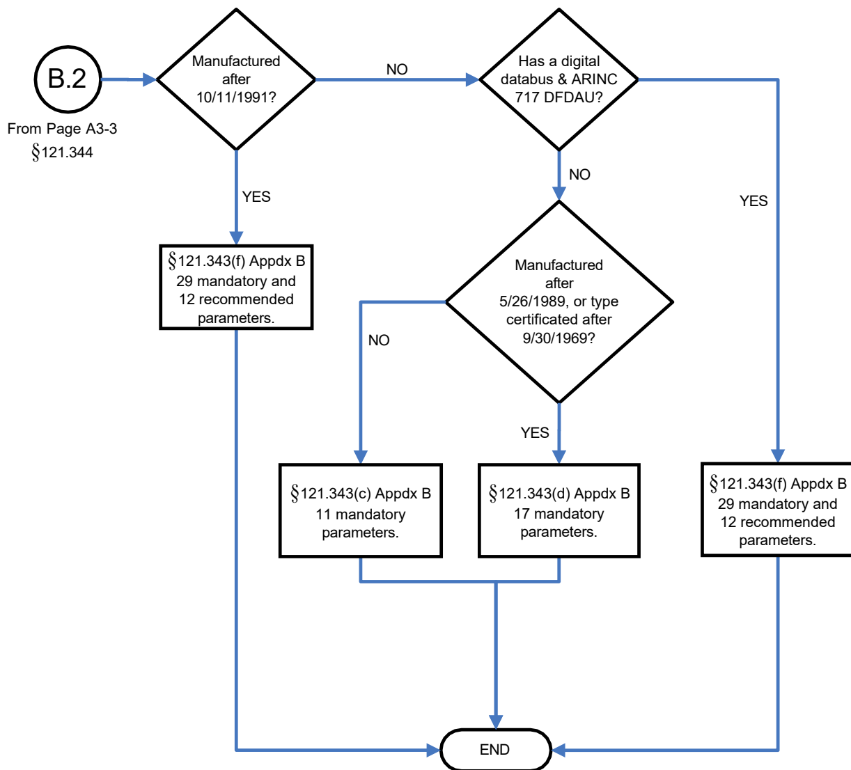
FIGURE 3-4. PART 121 FLIGHT RECORDER PARAMETER REQUIREMENTS § 121.343
