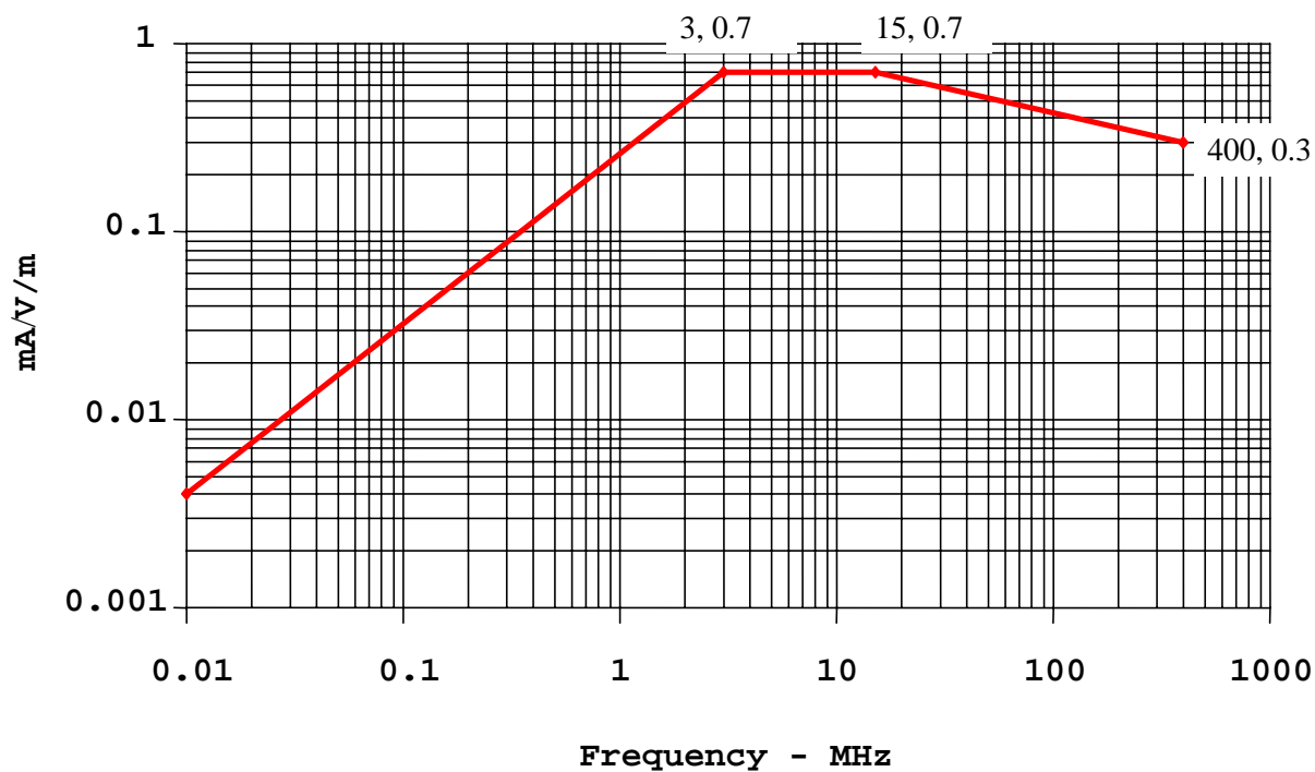
FIGURE A1-1 – Generic Transfer Function - Airplane
