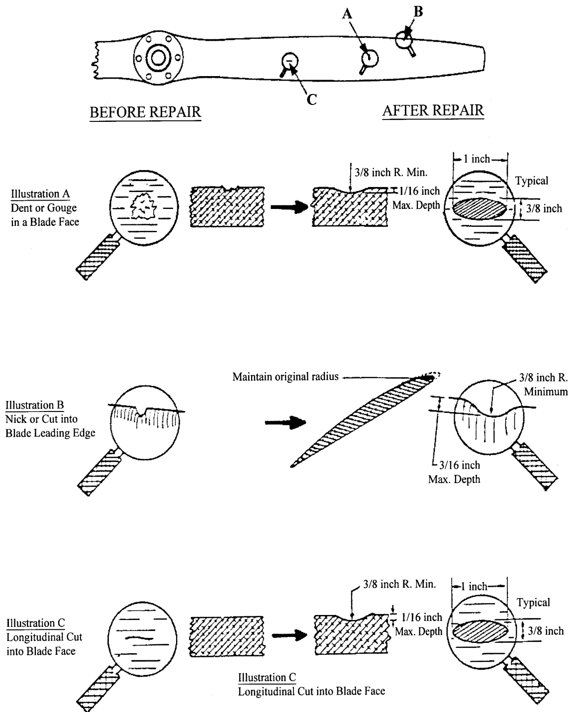
FIGURE 2-5. Techniques for Blade Repair
