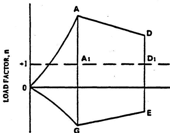
FIGURE 1 PITCHING MANOEUVRES
