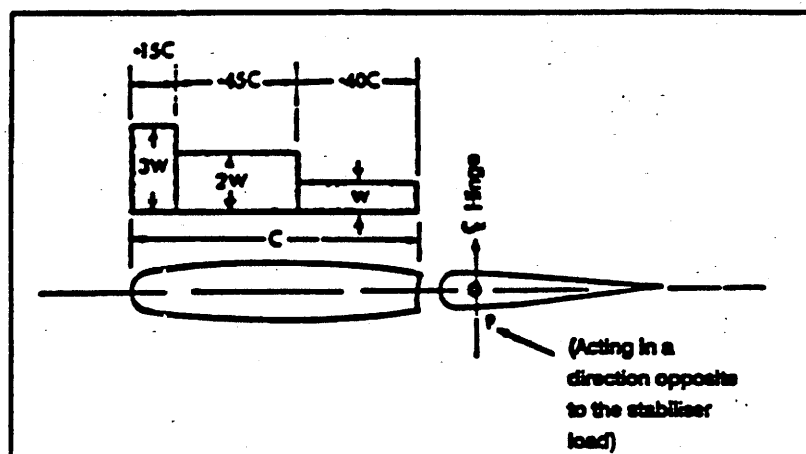
FIGURE B5 — GUST LOADING ON VERTICAL TAIL SURFACE.
