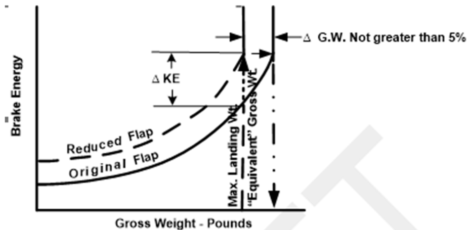
Figure 3-1. Equivalent Weight Extrapolation
