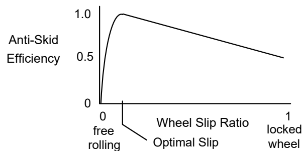
Figure 4-9. Anti-Skid Efficiency–Wheel Slip Relationship
