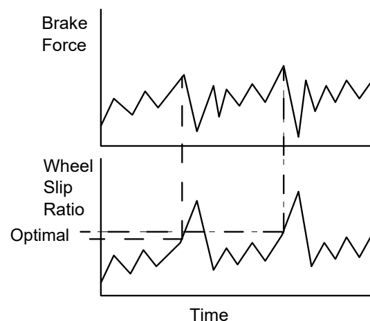
Figure 4-10. Substantiation of the Optimal Slip Value
