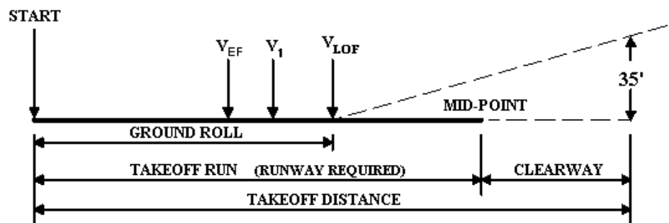
Figure 4-14. Takeoff Run: Critical Engine Fails at V_{EF}
