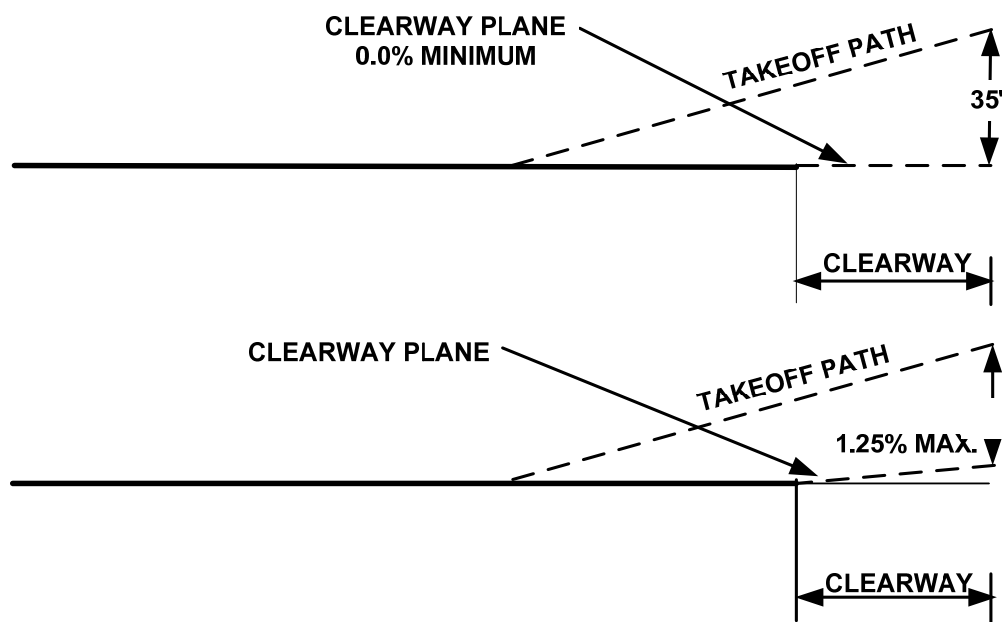
Figure 4-16. Clearway Profiles
