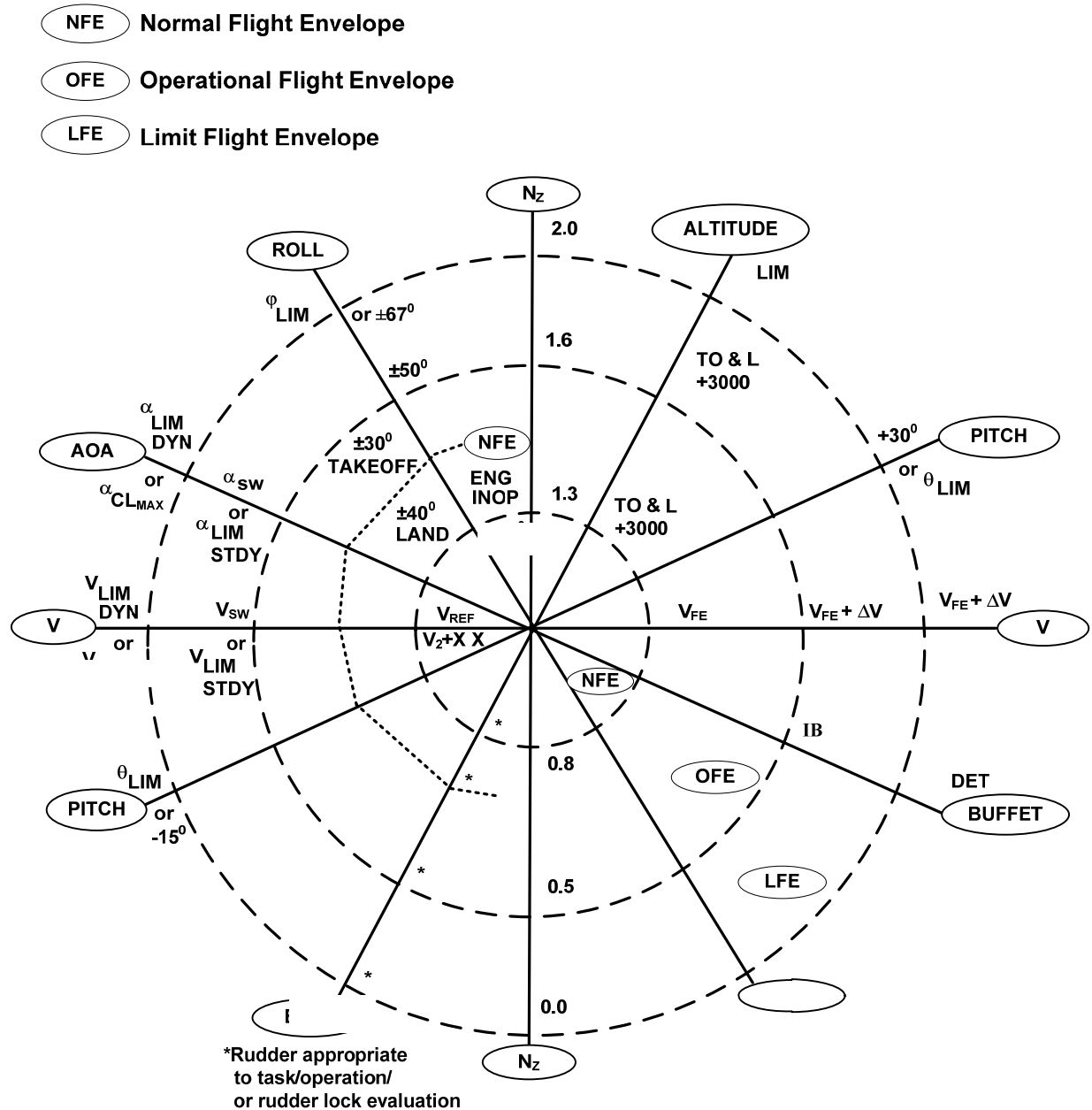
Figure E-5. Flaps DOWN Flight Envelopes
