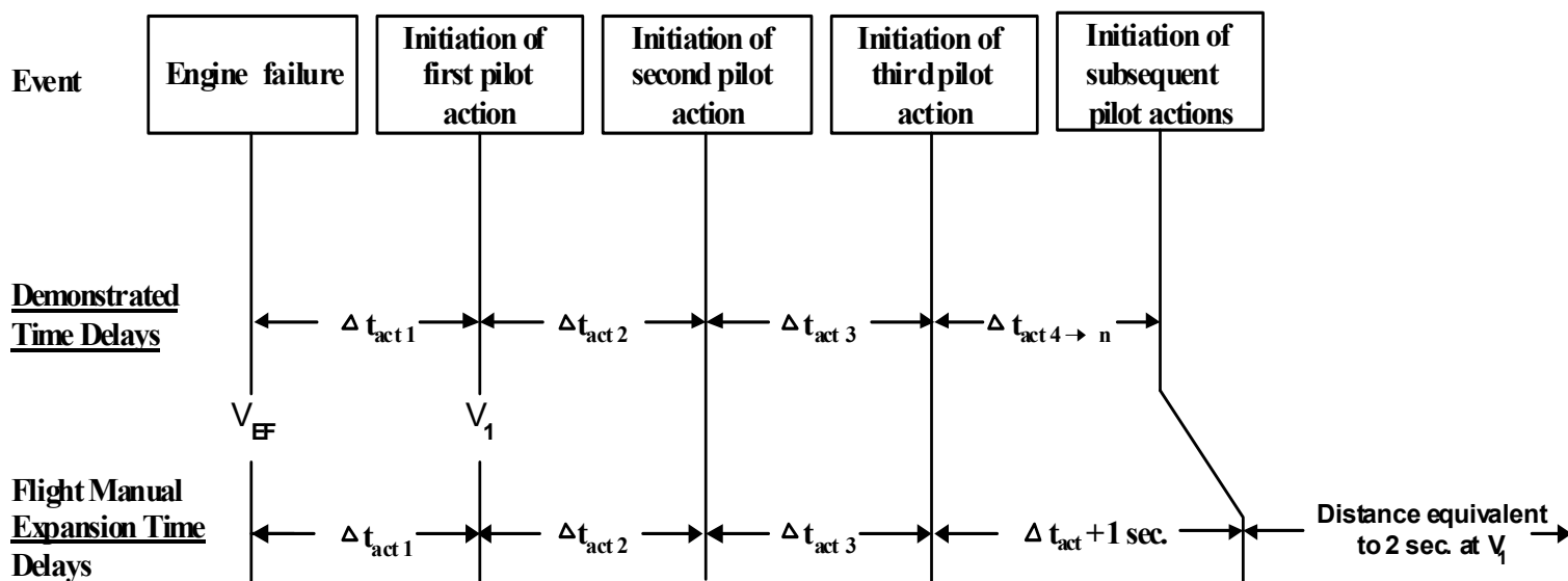
Figure 4-1. Accelerate-Stop Time Delays
