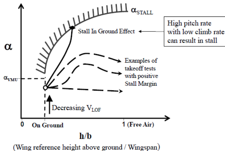
Figure 4-A. In-Ground-Effect Stall Margin
