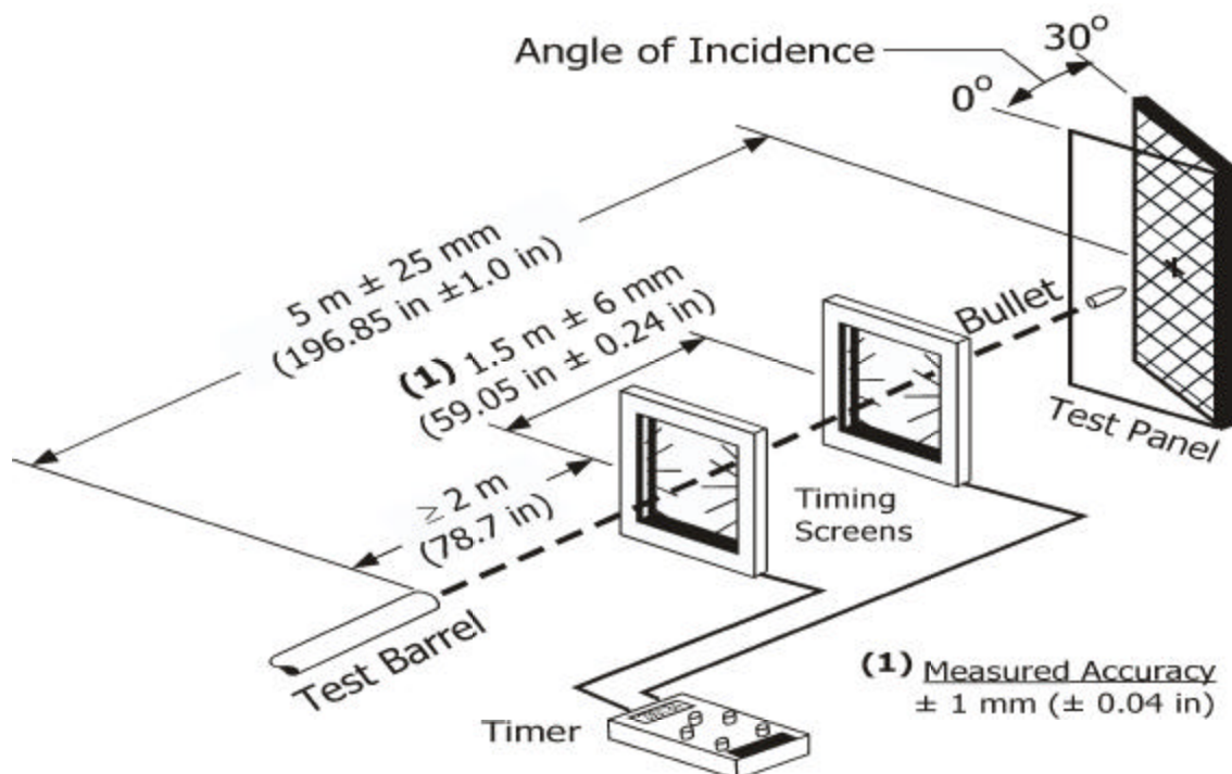
Figure 3. Test Arrangement for Ballistic Test Panels
