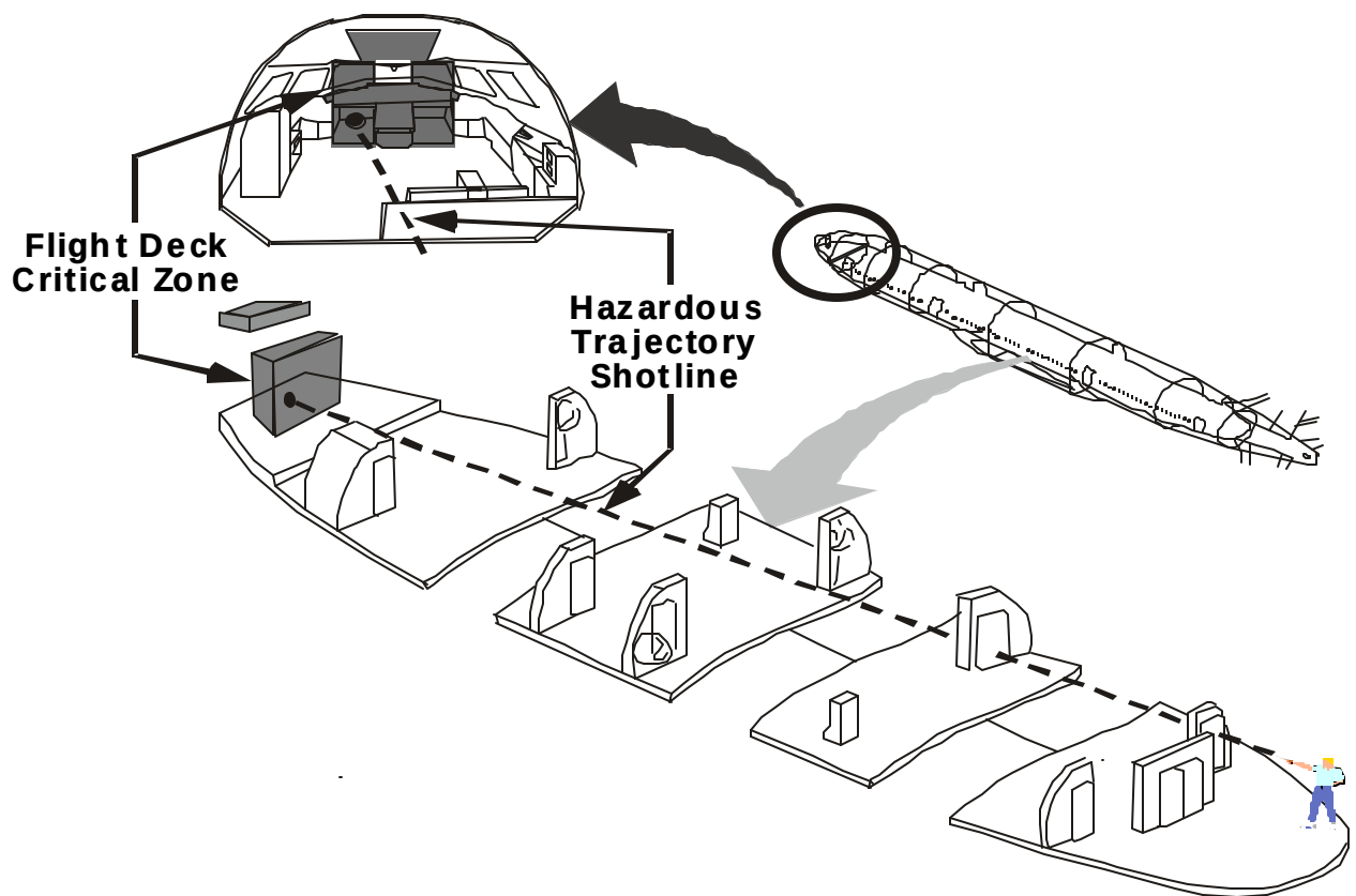
Figure 2. Example of a Hazardous Trajectory (Shotline Intersects Within the Critical Zone of the Flight Deck)
