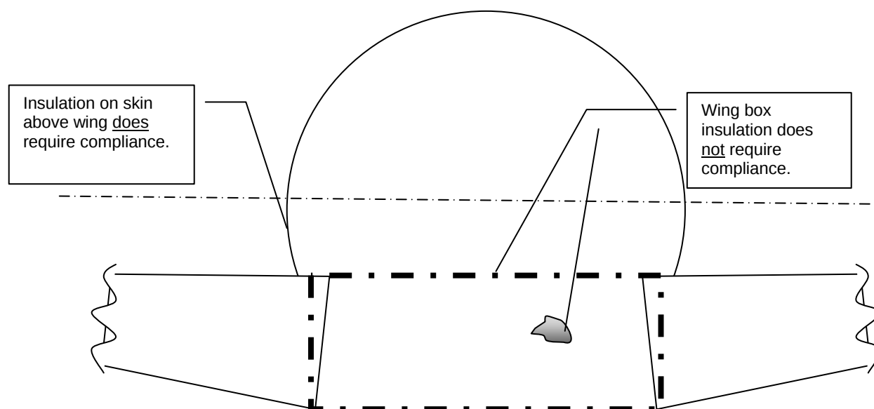
Figure 16. Wingbox Area
