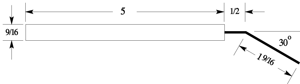
Figure 20. Igniter Geometry
