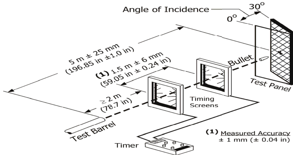
Figure 4. Test Arrangement for Ballistic Test Panels
