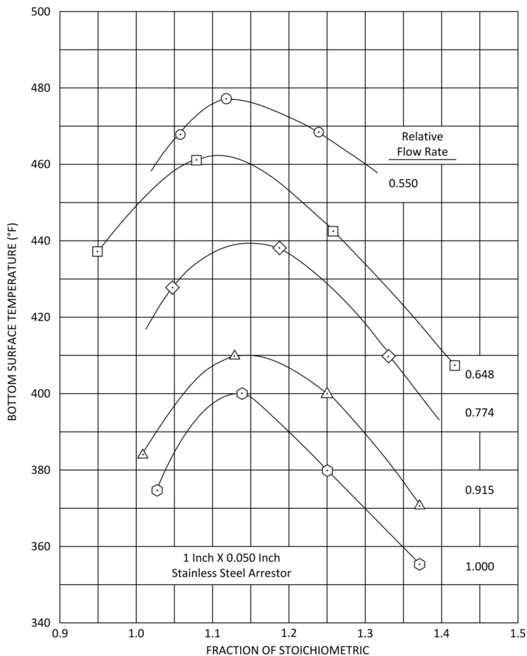
Figure A-2. Flame Arrestor Surface Temperature at Various Flow Rates and Stoichiometric Mixture Ratios 2
