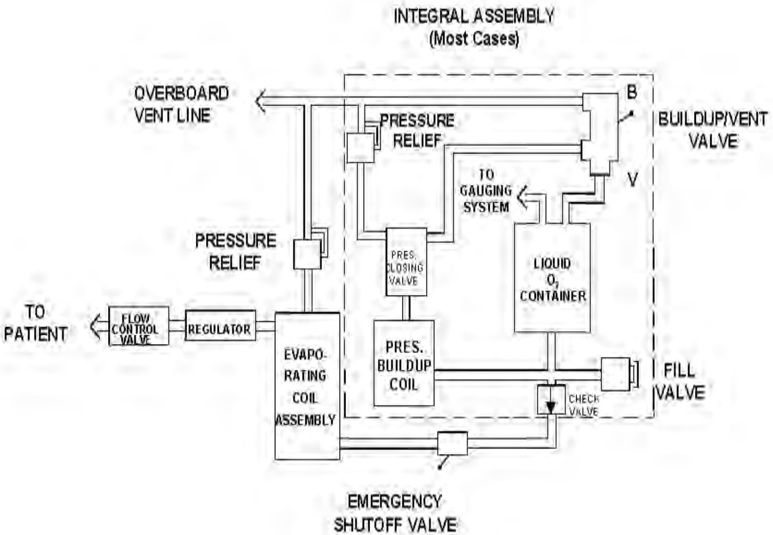
FIGURE AC 27.MG 6-1 TYPICAL LIQUID OXYGEN SYSTEM
