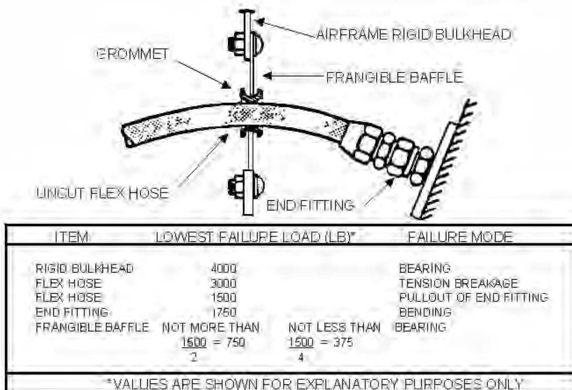
FIGURE AC 27.952-6 TYPICAL METHODS OF FRANGIBLE OR DEFORMABLE ATTACHMENT LOAD CALCULATIONS: EXAMPLE 2, FRANGIBLE BAFFLE.
