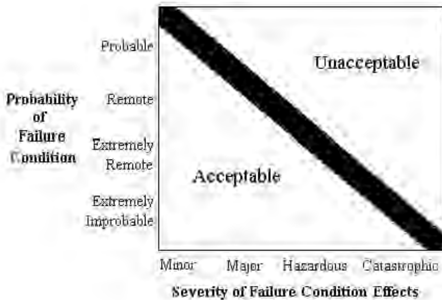
FIGURE AC 27.1309-1
