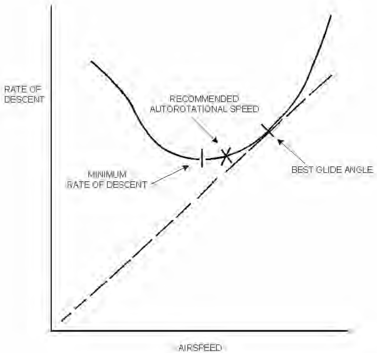
FIGURE AC 27-11-1 AUTOROTATIONAL CHARACTERISTICS - TYPICAL
