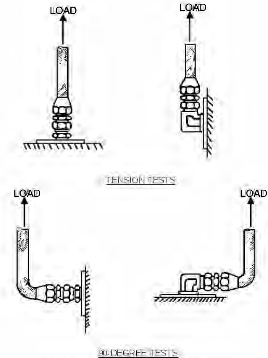
FIGURE AC 27.952-2 HOSE ASSEMBLY TESTS
