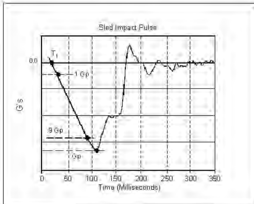
FIGURE AC 27.562-7. Impulse Shape
