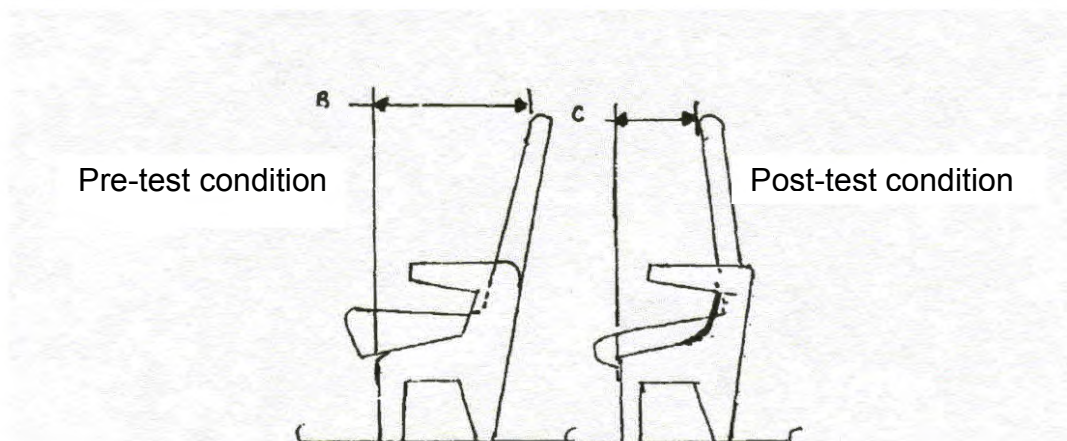
FIGURE AC 27.562-6
