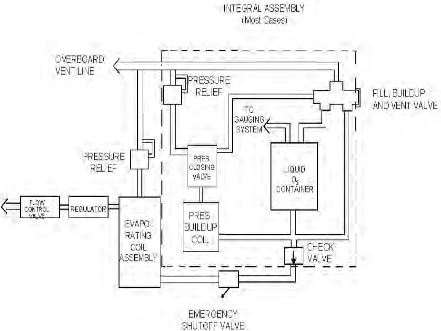
FIGURE AC 27.MG 6-2 TYPICAL LIQUID OXYGEN SYSTEM - USING COMBINATION VALVE
