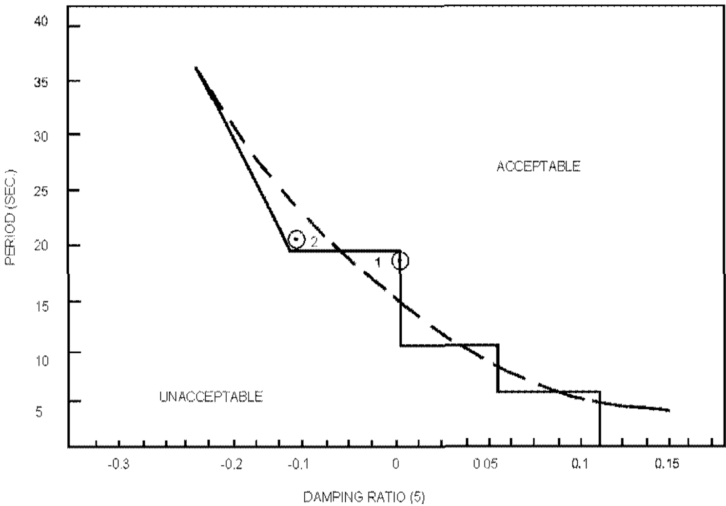
FIGURE AC 27-1B-1 ROTORCRAFT DYNAMIC STABILITY REQUIREMENTS FOR IFR
