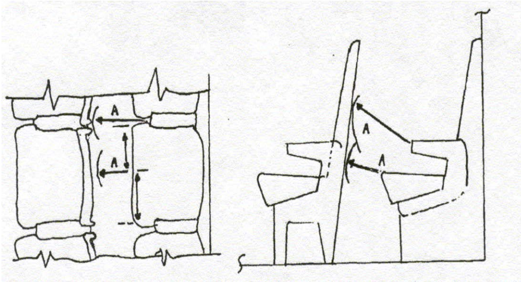
FIGURE AC 29.562-5
