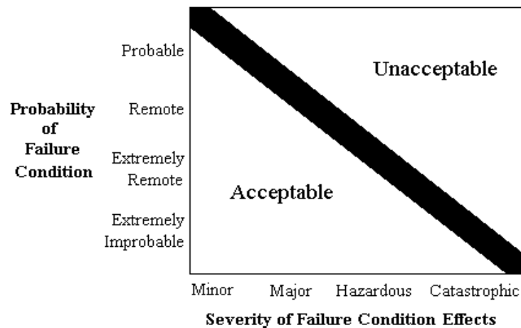
FIGURE AC 29.1309-1
