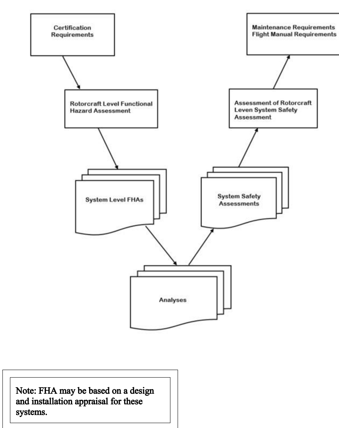
FIGURE AC 29.1309-4: Safety Assessment Process Overview
