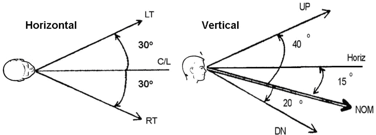
Figure AC 29 MG 19-2 Secondary Field of View
