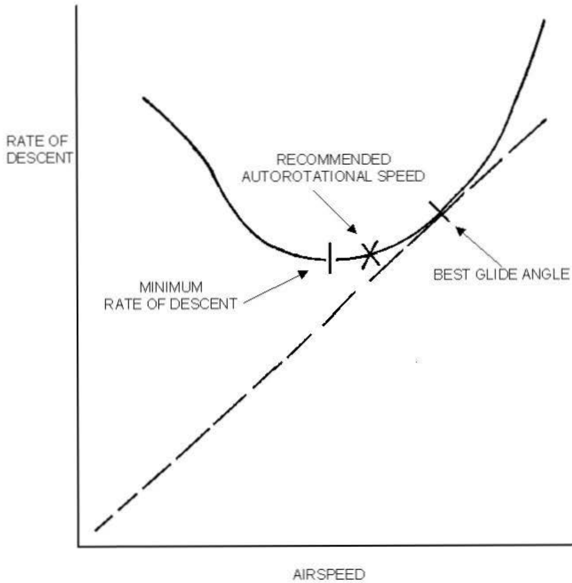
FIGURE AC 29.71-1 AUTOROTATIONAL CHARACTERISTICS - TYPICAL
