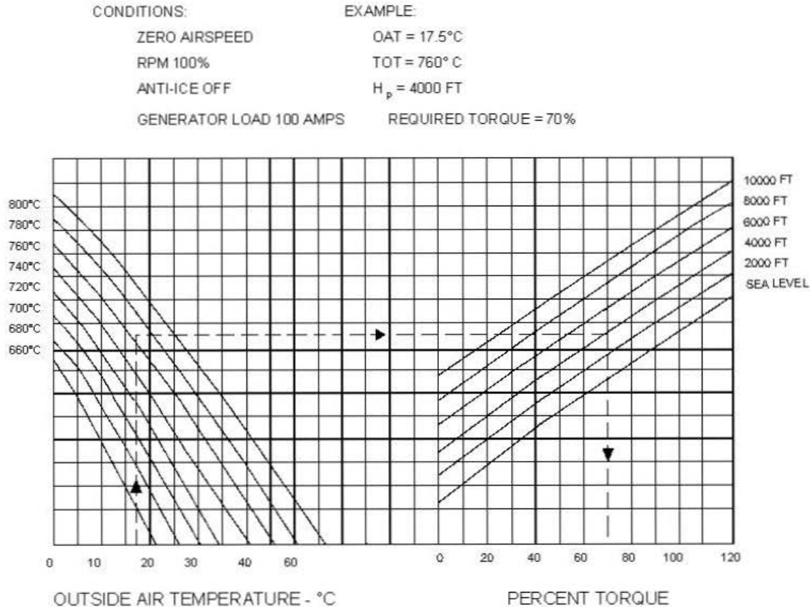
FIGURE AC 29.45-6 POWER ASSURANCE CHECK CHART
