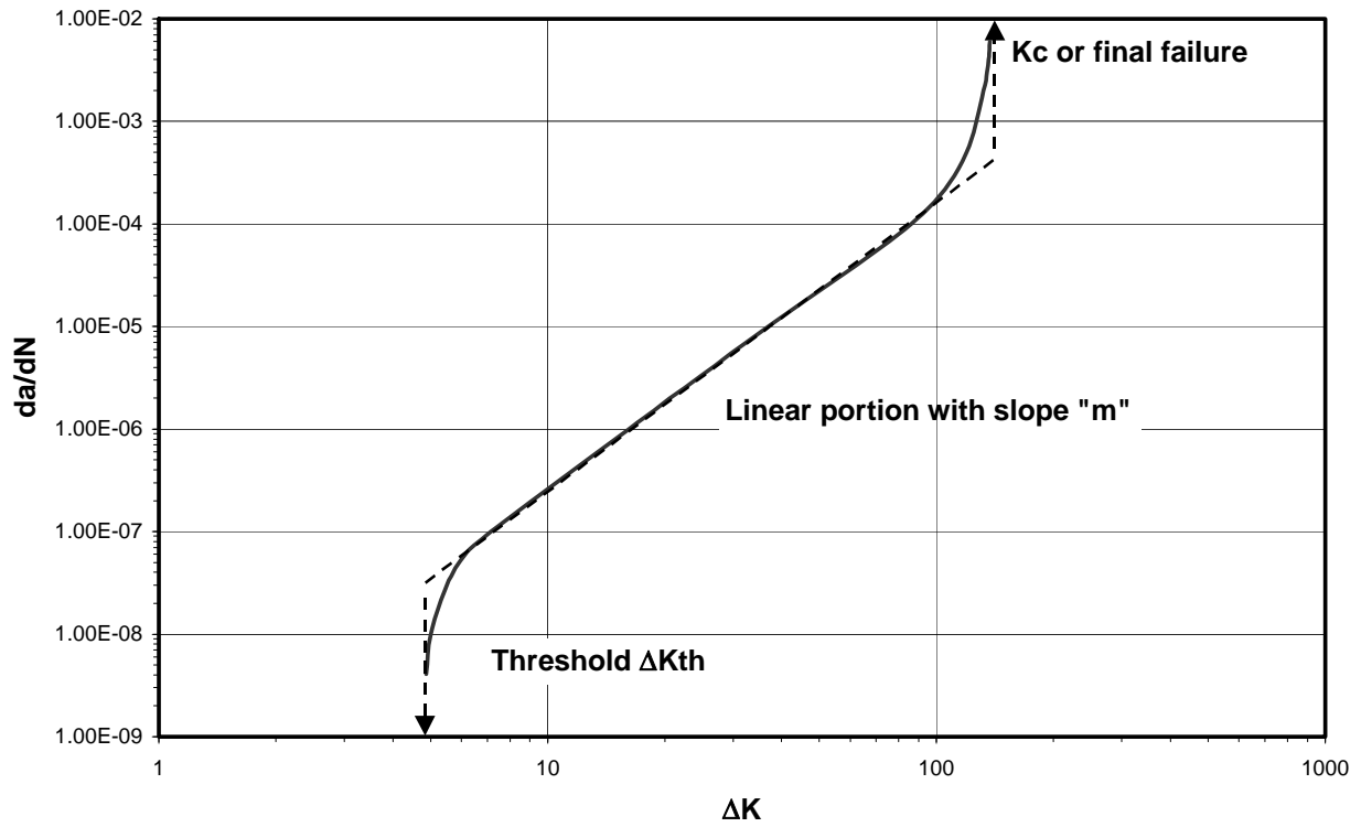
Figure 6 Typical Crack Growth Curve Shape
