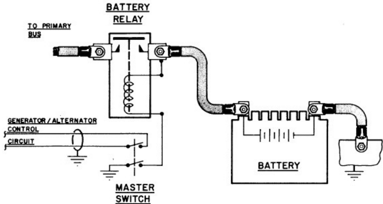
Figure 11-4. Typical Battery Cutoff and Generator Alternator Control Circuit
