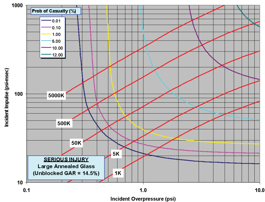
Figure 28 – Large Annealed Windows (~5'H x 6'W x 0.232"T), GAR = 14.5 percent
