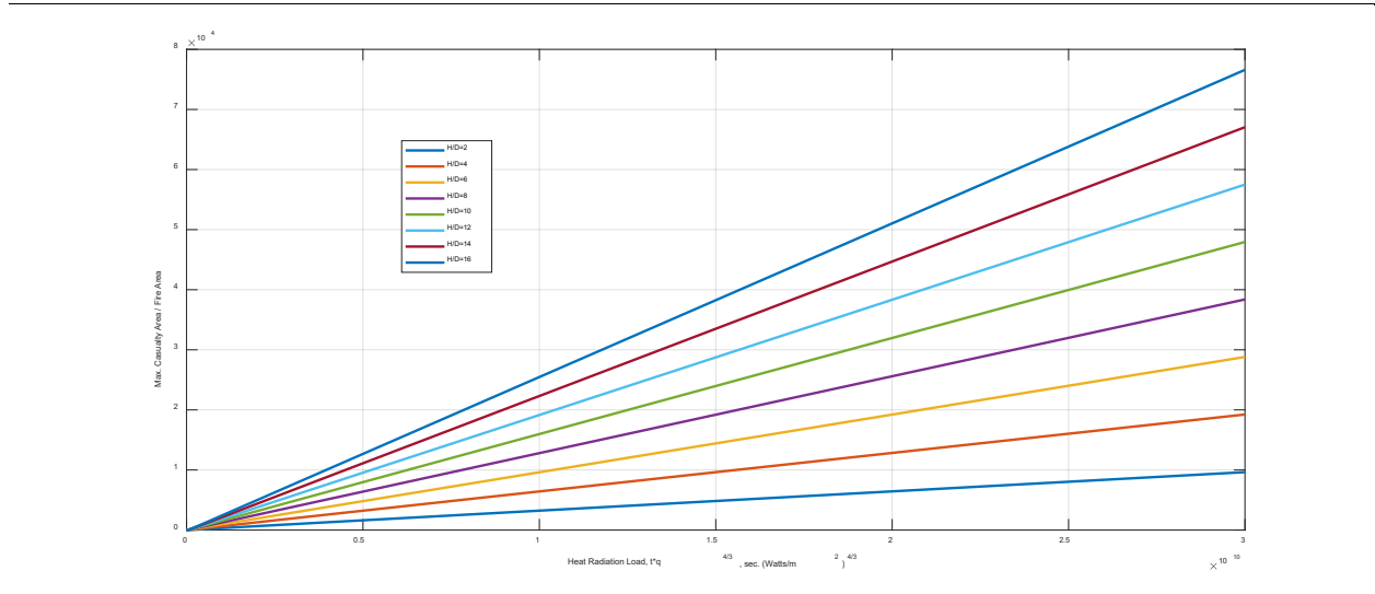
Figure 26 – Normalized Casualty Areas vs. Heat Load
