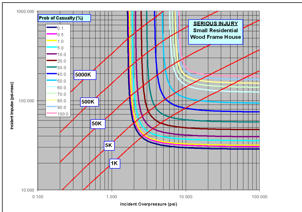
Figure 27 – Probability of Casualty for a Small Wood Structure, ~2500 ft 2
