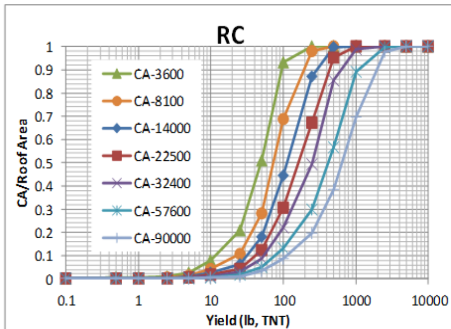
Figure 25 – Reinforced Concrete Roof Effective Casualty Area Ratio as a Function of Roof Area and Yield
