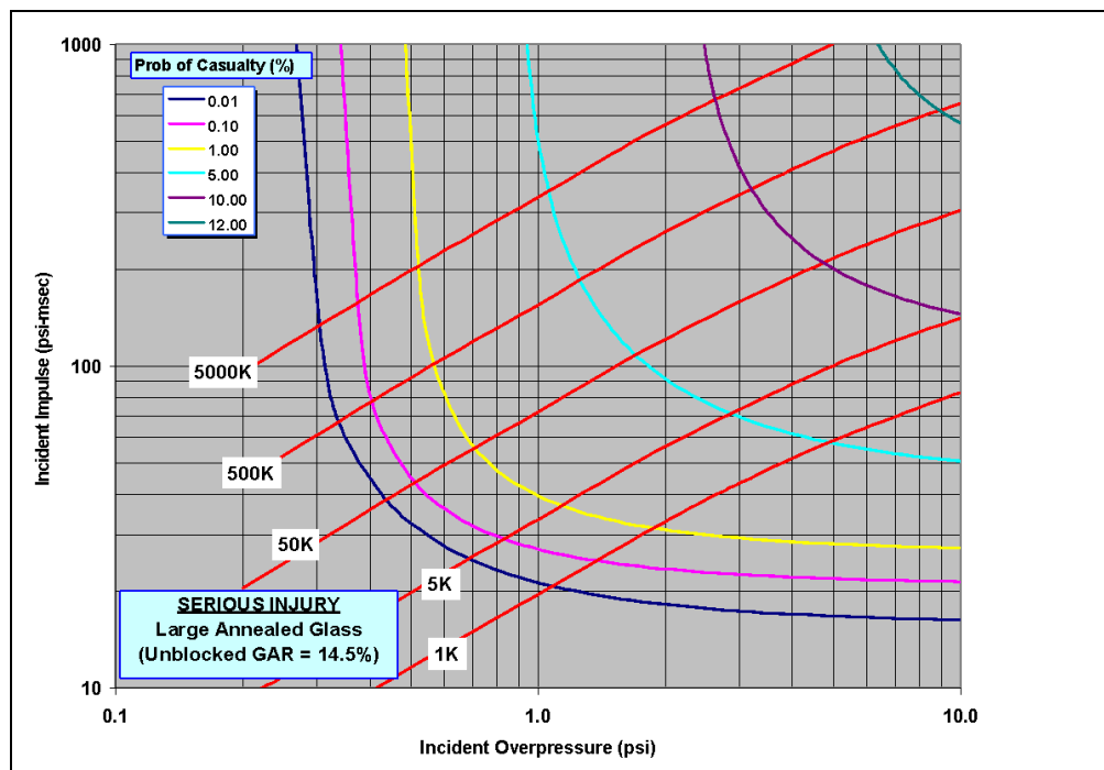
Figure 28 – Large Annealed Windows (~5'H x 6'W x 0.232"T), GAR = 14.5 percent
