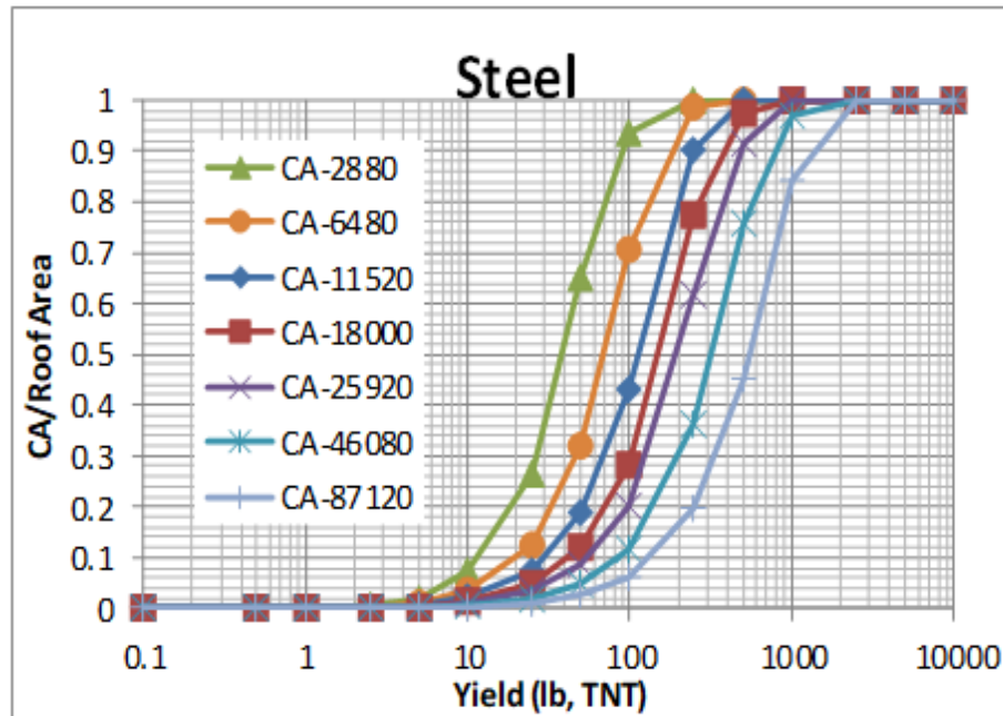
Figure 24 – Steel Roof Effective Casualty Area Ratio as a Function of Roof Area and Yield
