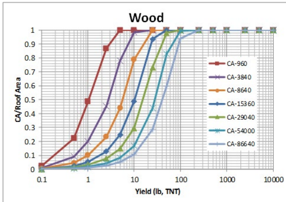
Figure 23 – Wood Roof Effective Casualty Area Ratio as a Function of Roof Area and Yield
