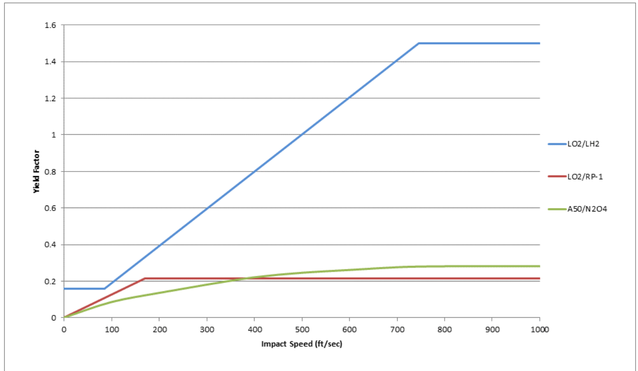
Figure 14 – Yield Curves for Liquid Propellants on Hard Surfaces
