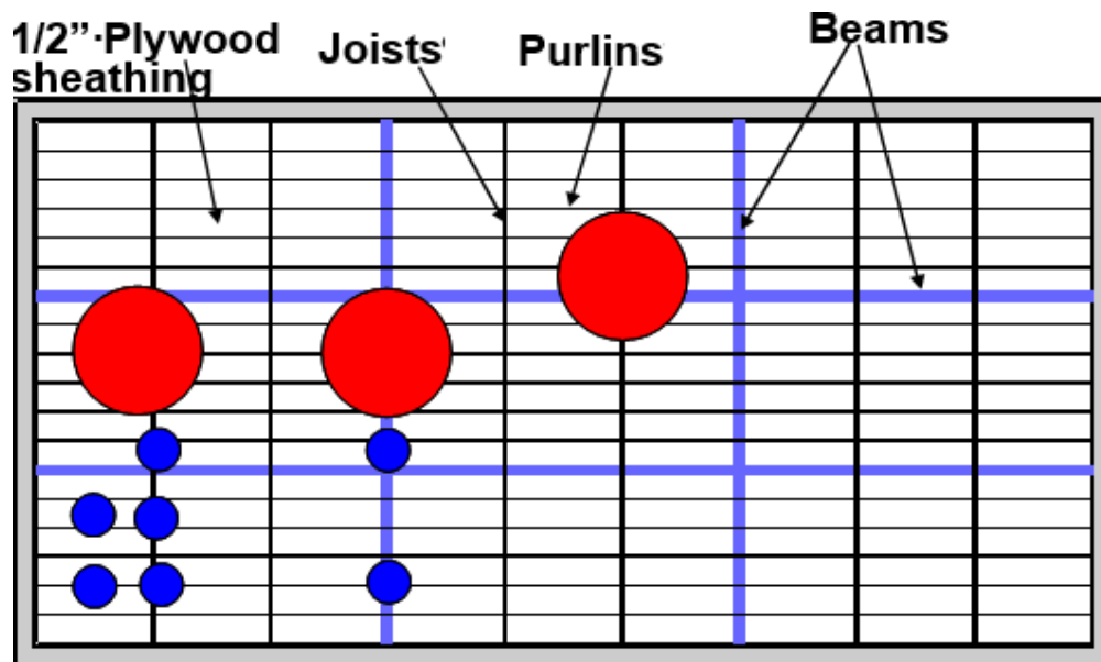
Figure 6 – Illustration of a Wood Built-Up Roof
