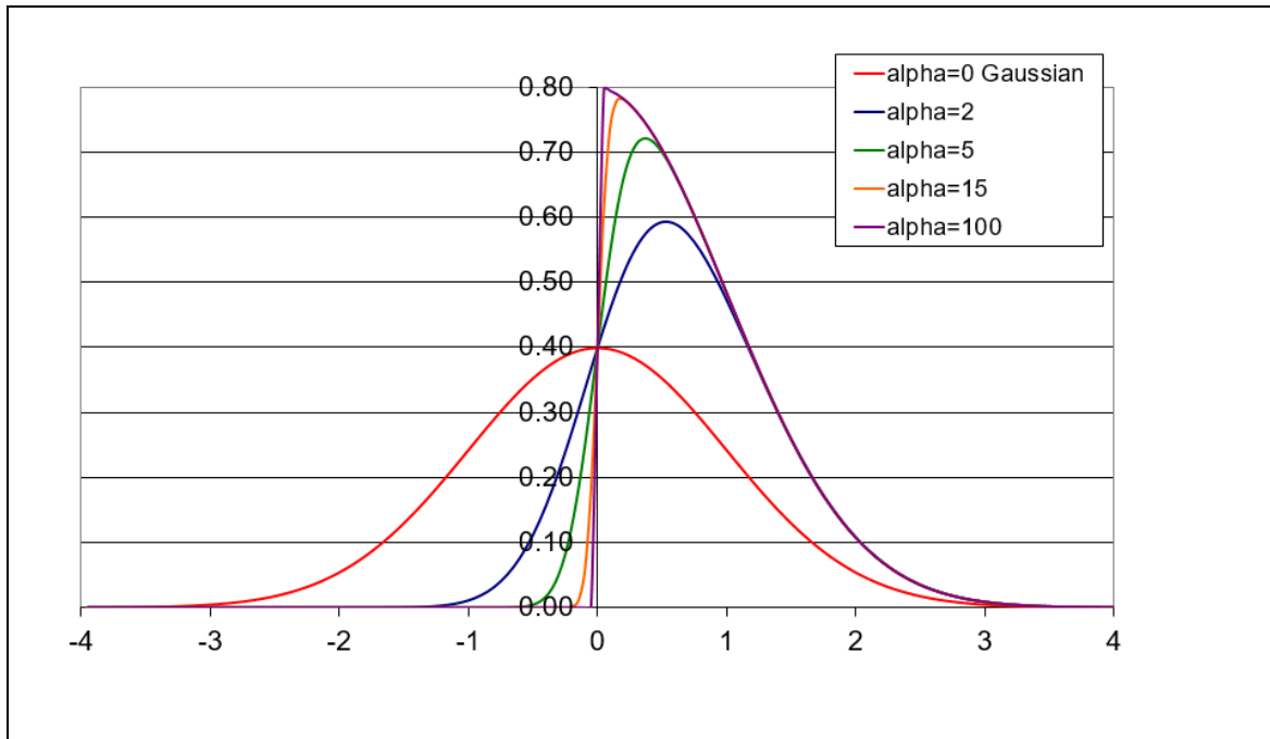
Figure 1 – Comparison of Various Skew-Normal Curves
