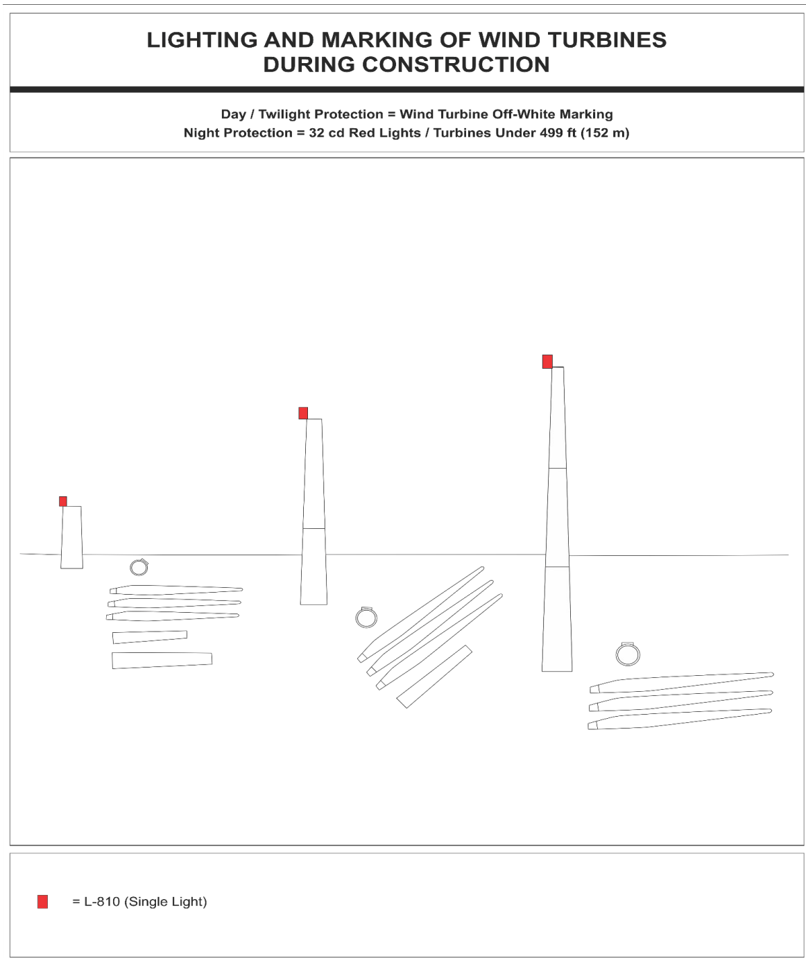
Figure A-30. Marking and Lighting of Turbines During Construction
