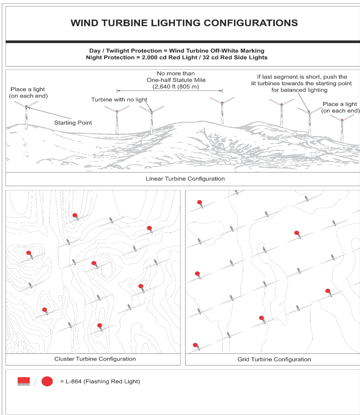
Figure A-26. Wind Turbine Lighting Configurations
