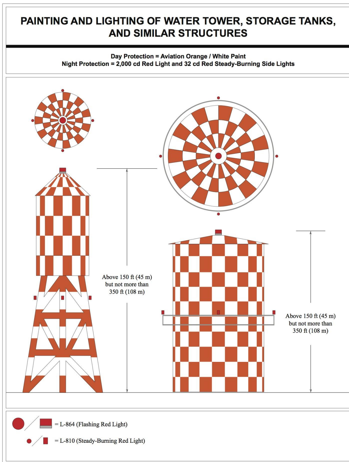
Figure A-15. Painting and Lighting of Water Towers, Storage Tanks, and Similar Structures
