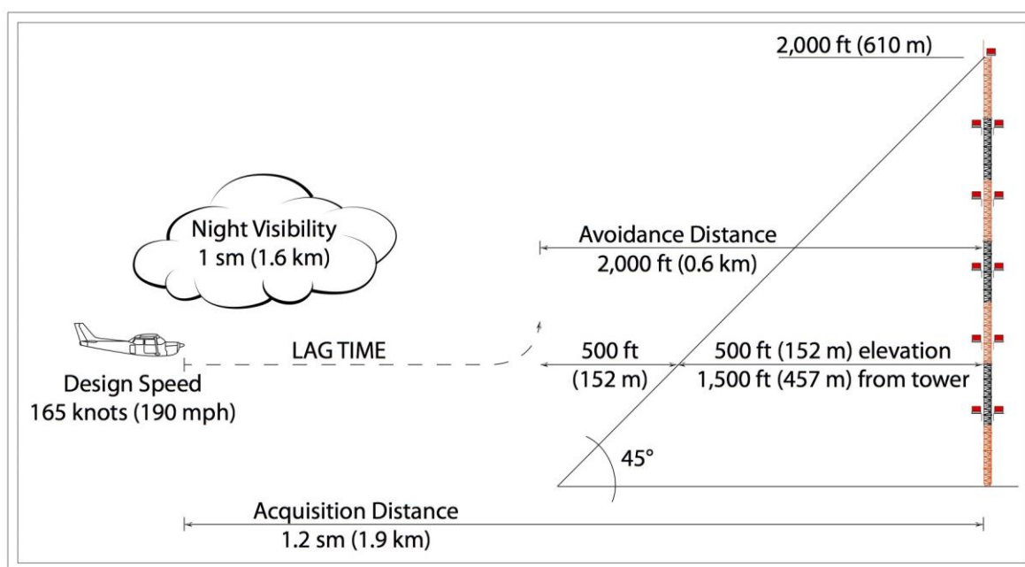
Figure B-1. Illustration of Acquisition Distance Calculation
