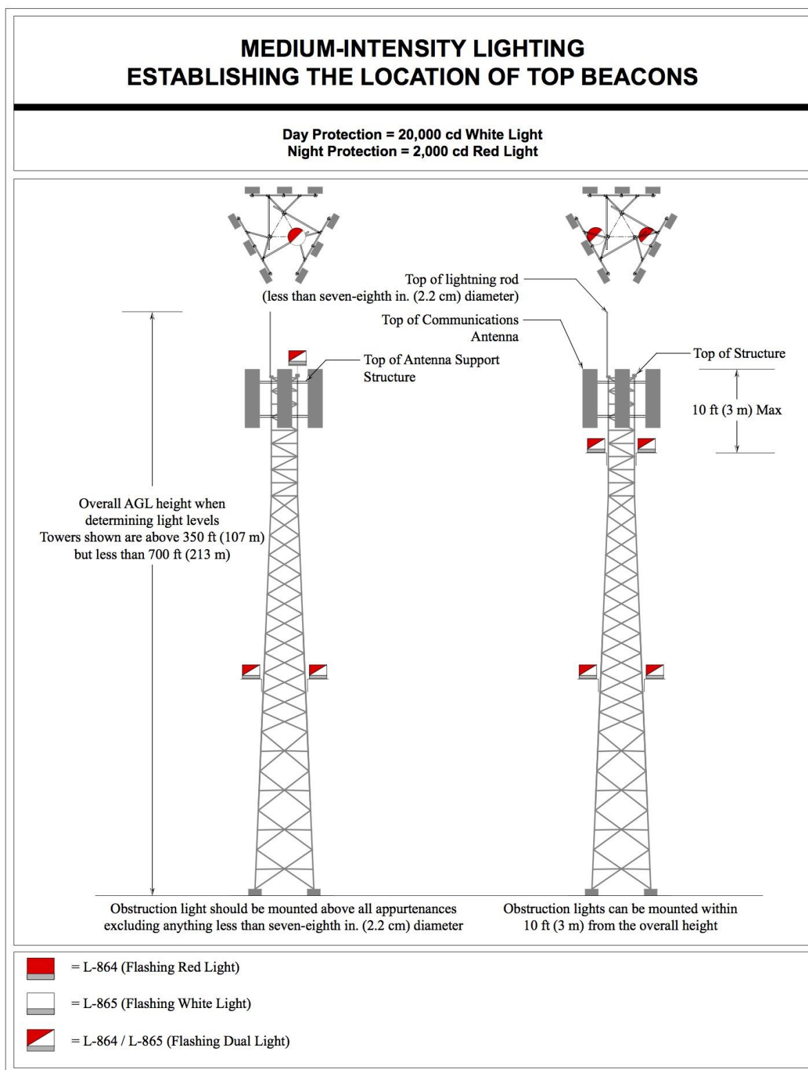
Figure A-14. Medium-Intensity Lighting—Establishing the Location of Top Beacons
