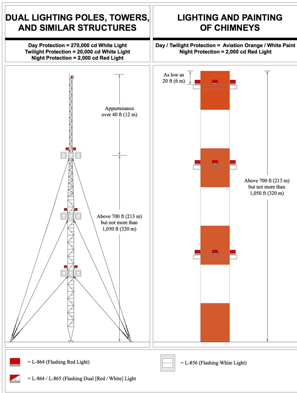
Figure A-13. Painting and/or Dual Lighting of Chimneys, Poles, Towers, and Similar Structures
