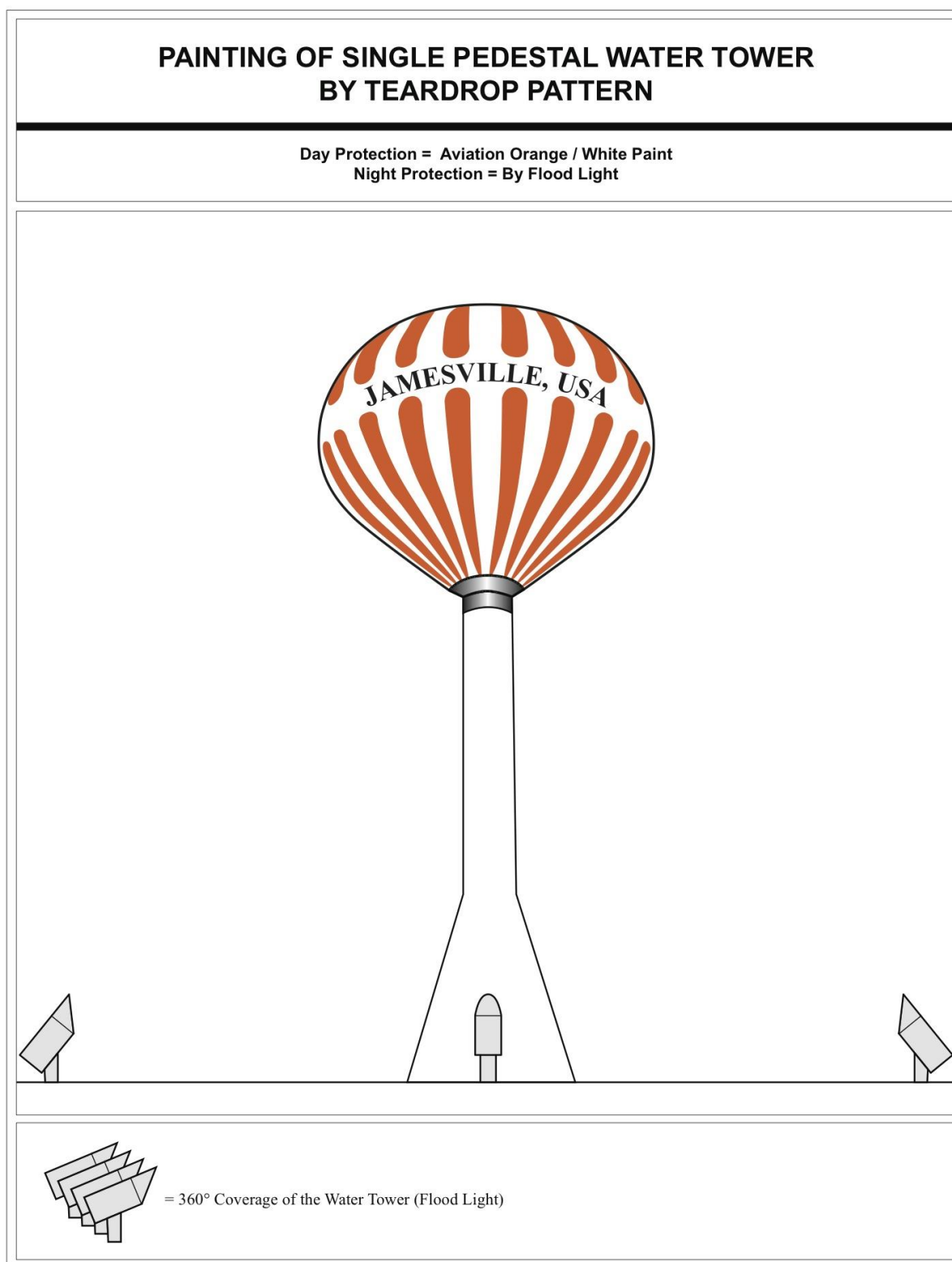
Figure A-17. Painting a Single Pedestal Water Tower Using the Teardrop Pattern
