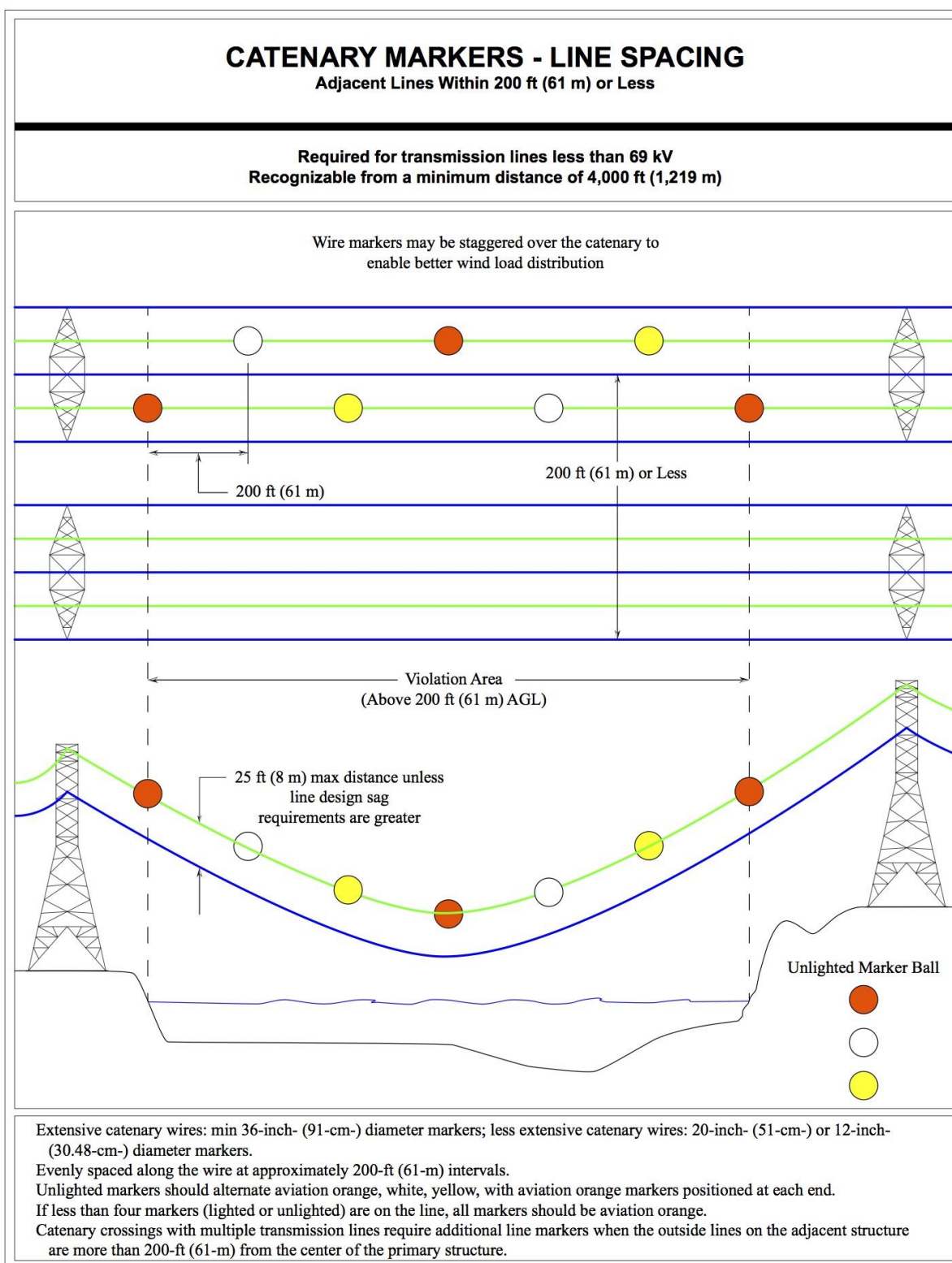
Figure A-3. Catenary Markers – Line Spacing (Adjacent Lines Within 200 ft (61 m) or Less
