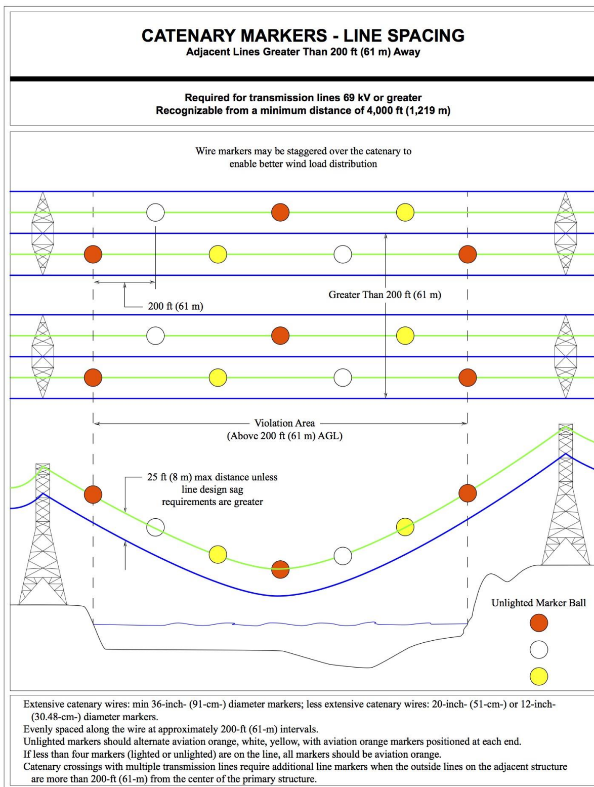
Figure A-2. Catenary Markers - Line Spacing (Adjacent Lines Greater Than 200 ft (61 m) Away)
