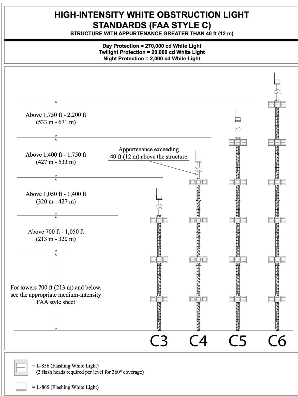
Figure A-9. High-Intensity Obstruction Lighting Standards—Structures With Appurtenance Over 40 Feet High
