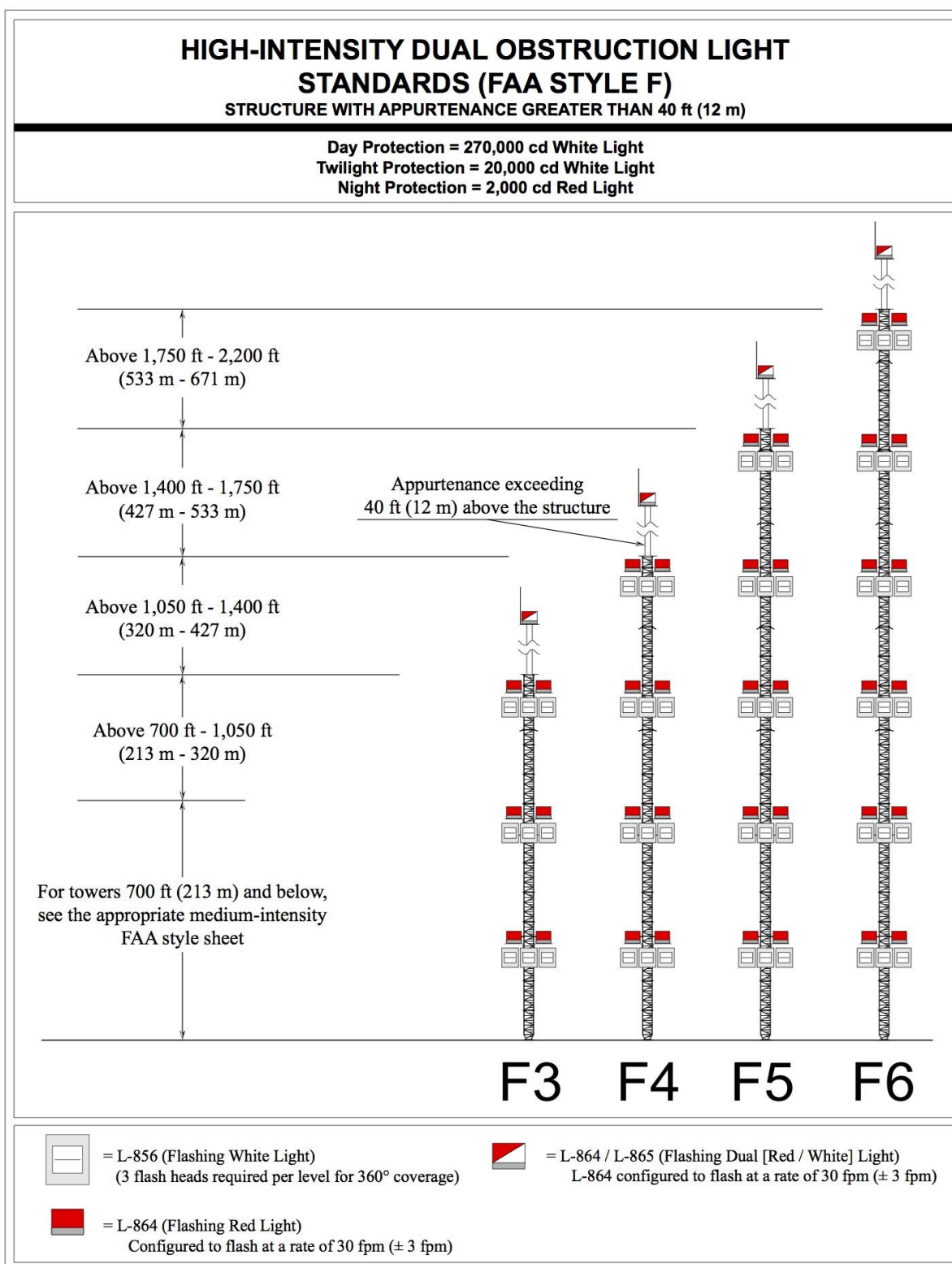
Figure A-11. High-Intensity Dual Obstruction Lighting Standards—Structures With Appurtenance Over 40 Feet High
