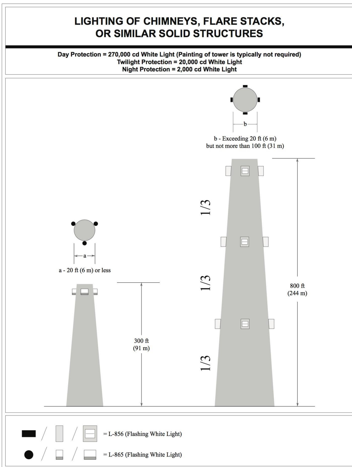
Figure A-20. Lighting of Chimneys, Flare Stacks, or Similar Solid Structures
