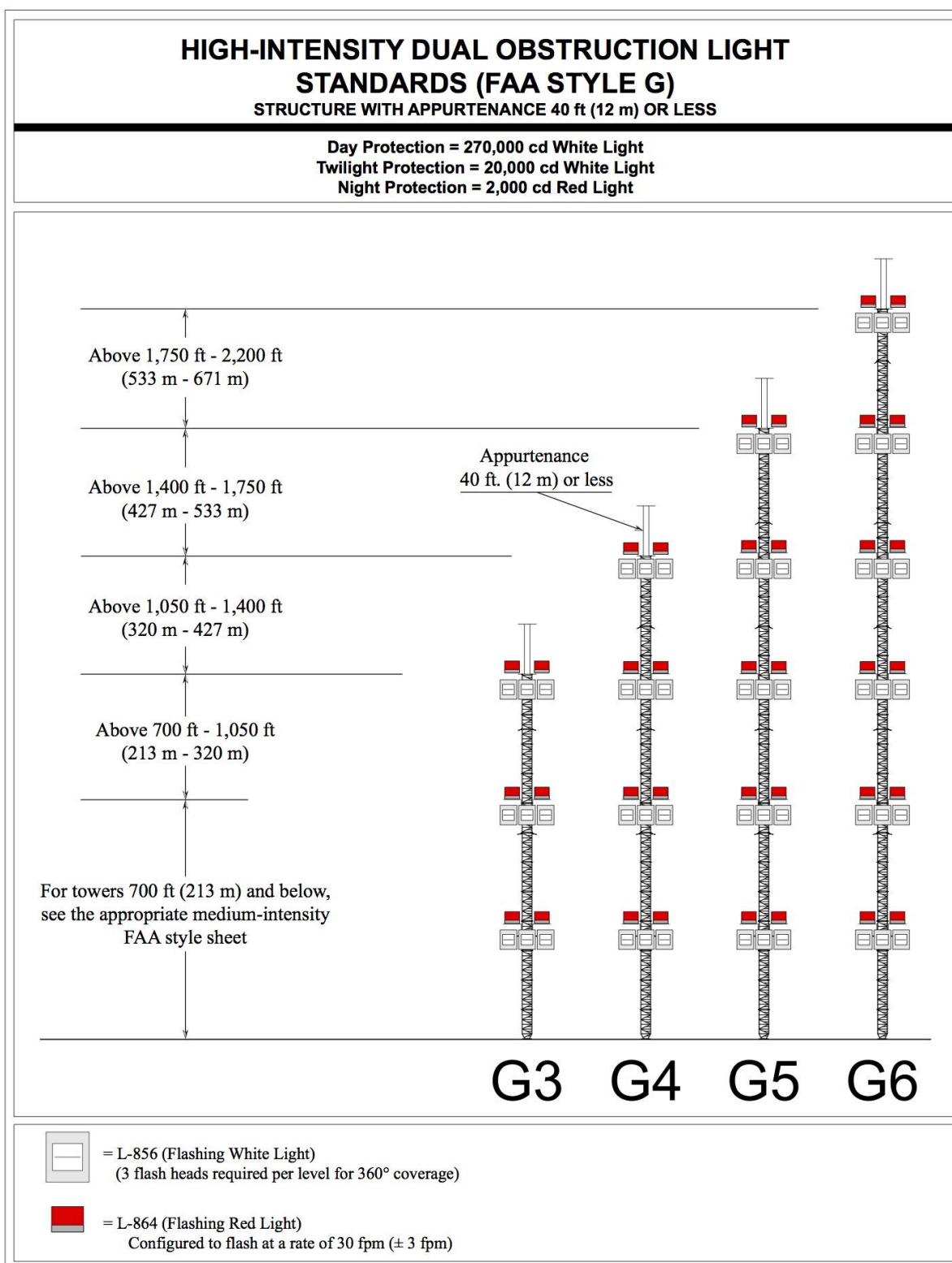
Figure A-12. High-Intensity Dual Obstruction Lighting Standards—Structures With Appurtenance 40 Feet or Less
