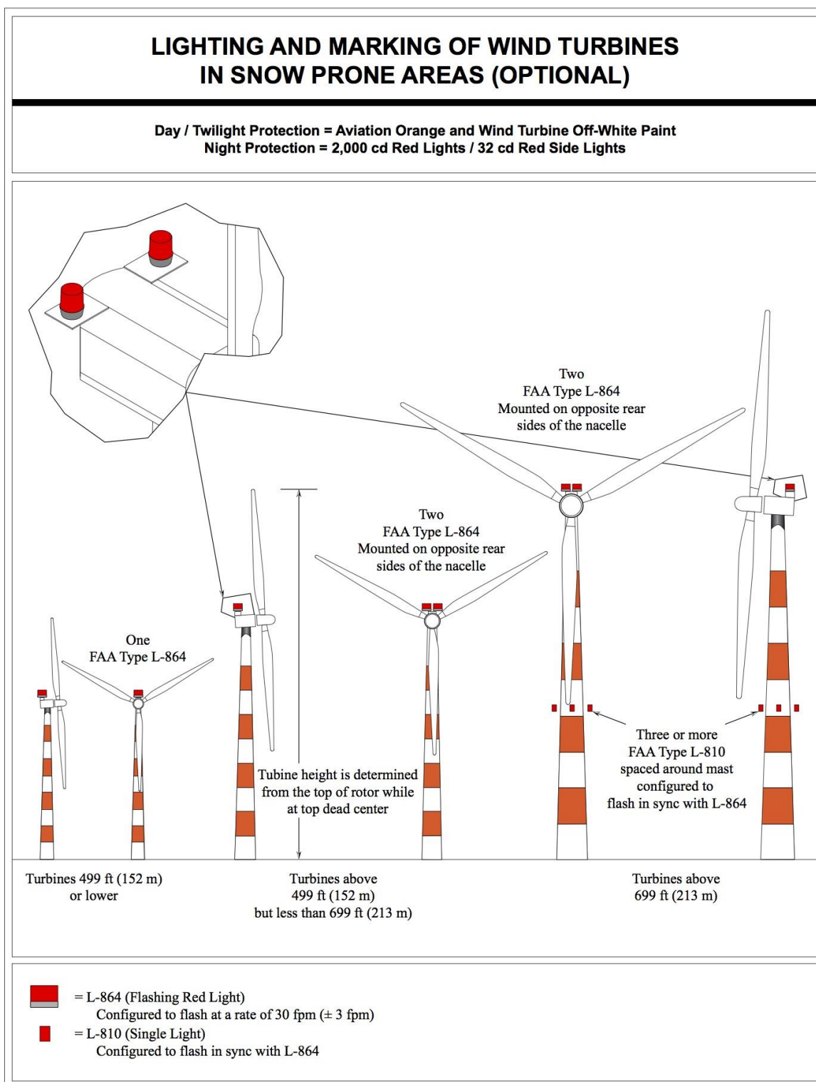
Figure A-24. Wind Turbine Lighting and Marking in Snow Prone Areas (Optional)
