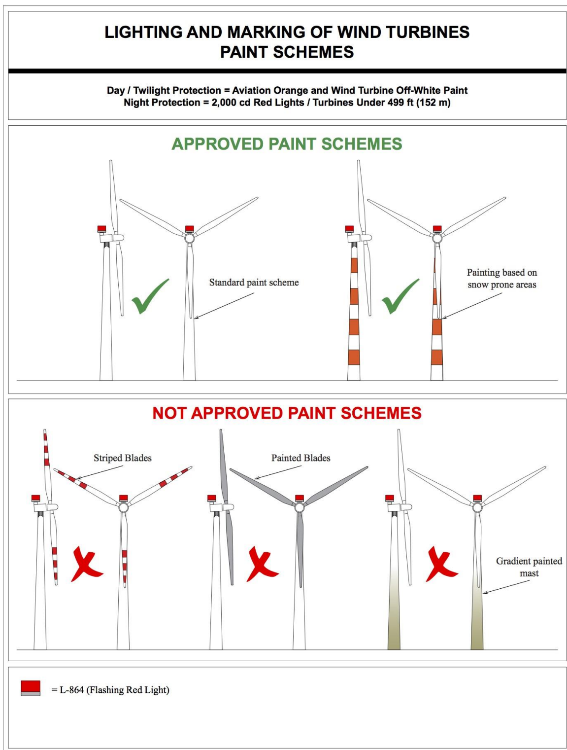
Figure A-25. Lighting and Marking of Wind Turbines – Paint Schemes
