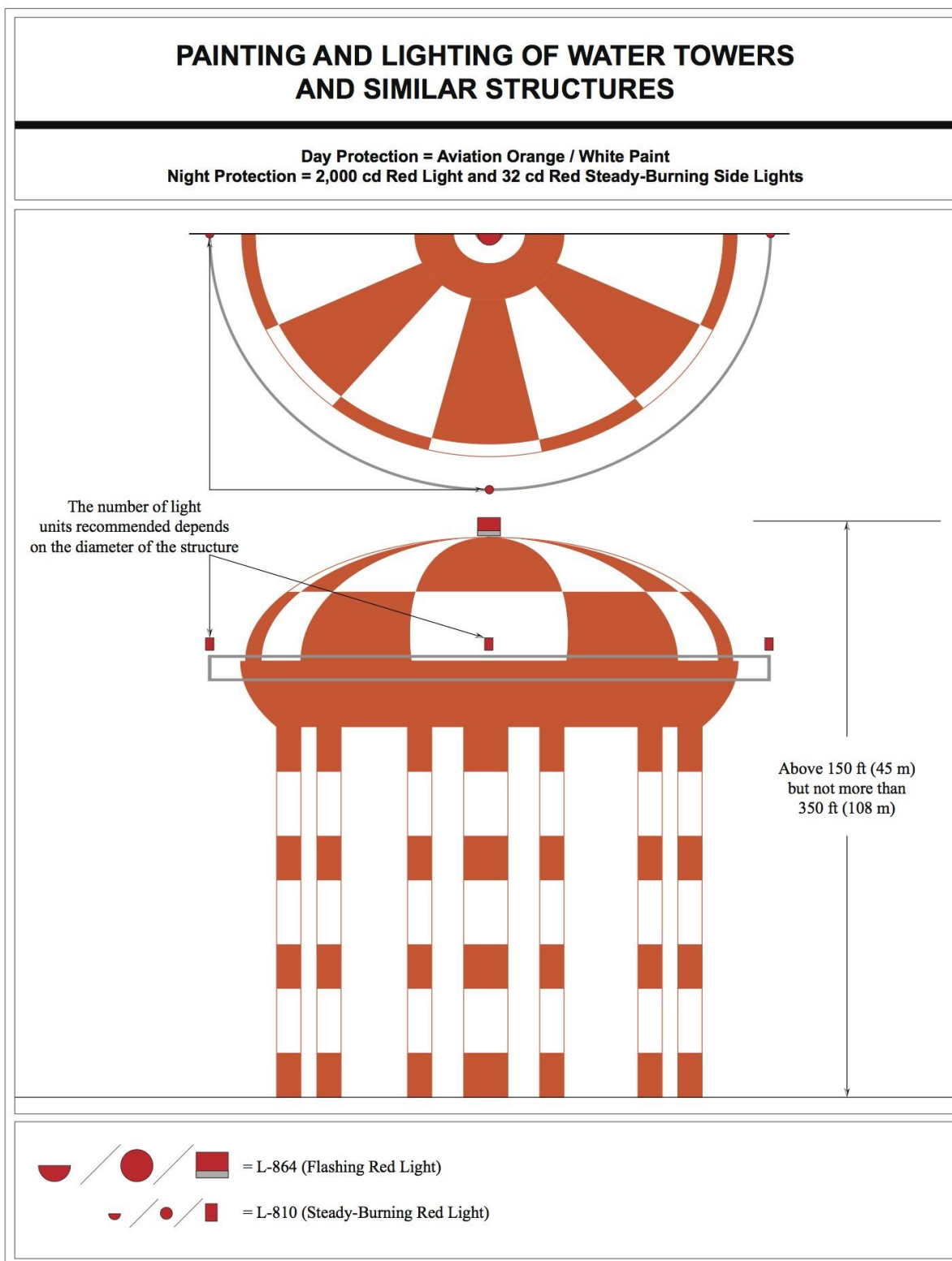
Figure A-16. Painting and Lighting of Water Towers and Similar Structures
