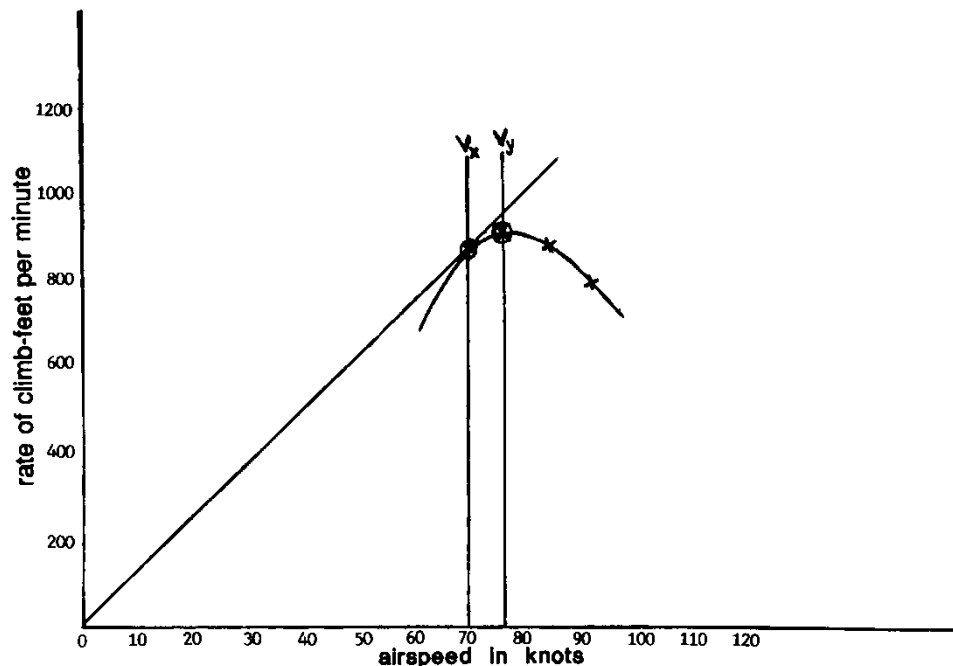
Figure 6-2. Best Rate of Climb Speed Graph
