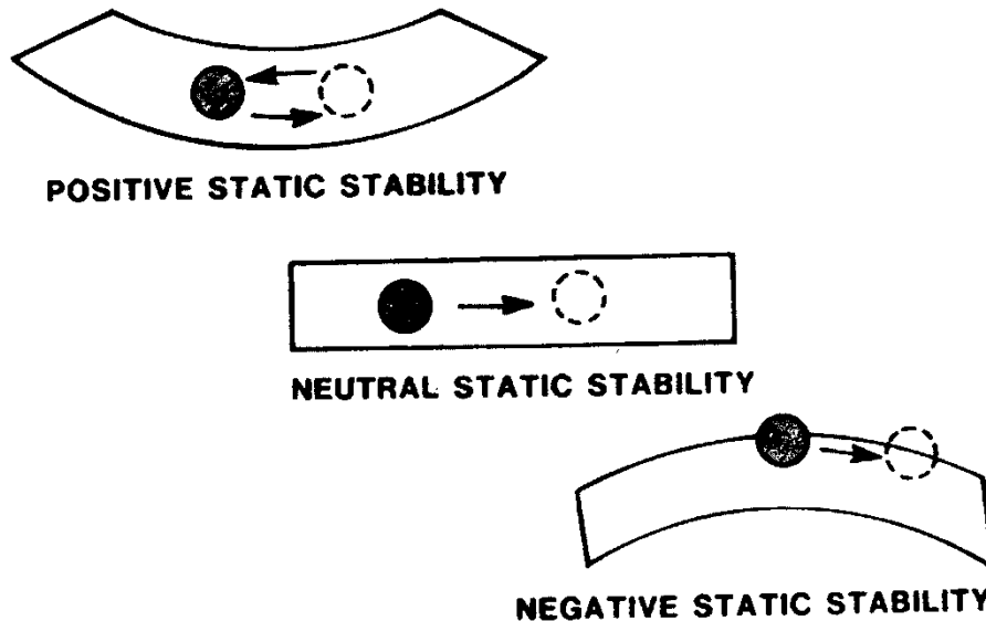
Figure 6-3. Static Stability
