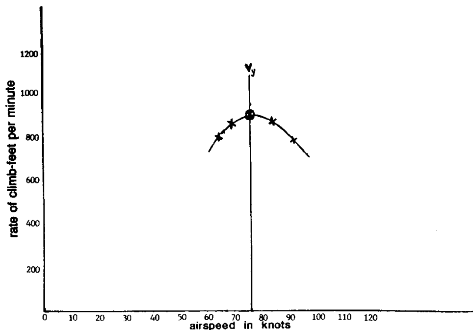
Figure 6-1. Climb Airspeed and Altitude Graph
