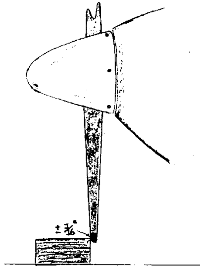
Figure 2-9. Propeller Tracking
