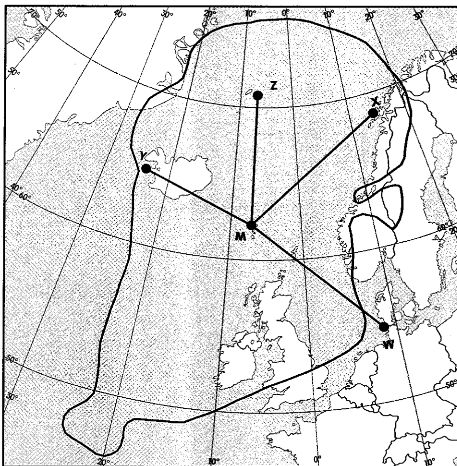
FIGURE 2-5. NORWEGIAN SEA CHAIN - 7970 LORAN-C COVERAGE
