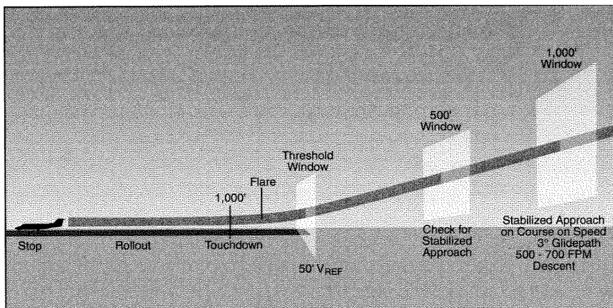
FIGURE 1-1. STABILIZED APPROACH
