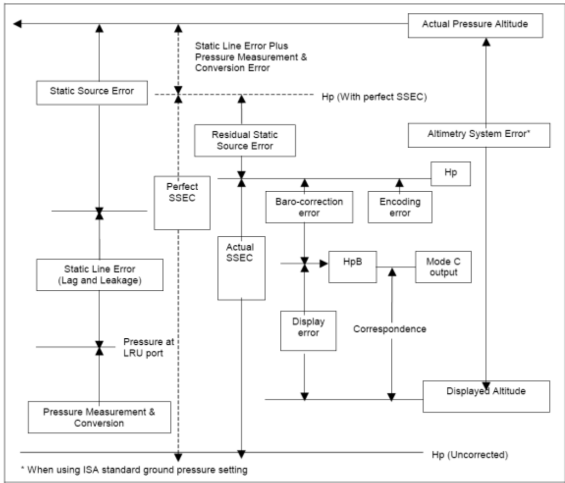
Figure A.8-1. Altimetry System Error and Its Components
